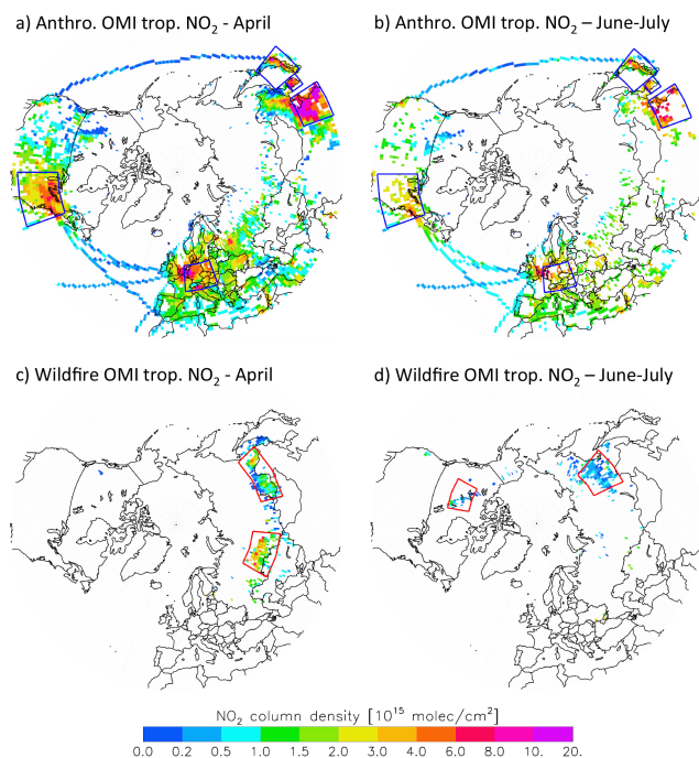
Figure 13. OMI NO 2 filtered for dominant anthropogenic emissions (a, b) and fire emissions (c, d). Boxes indicate the regions for which biases have been calculated in Fig. 14. Panels (a) and (c) show April, panels (b) and (d) show June–July.
