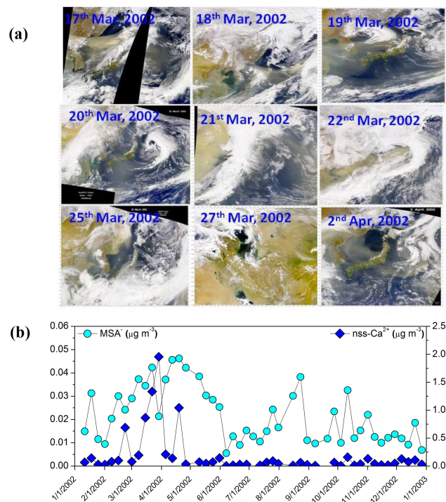
Figure 12. (a) The SeaWiFS images that captured the large Asian dust storm visible over the Sea of Japan and North Pacific during 17 March–2 April 2002. (b) Temporal variations of MSA - and nss-Ca 2+ concentrations during 2002 over the western North Pacific. The black regions in (a) are the gaps between consecutive SeaWiFS viewing swaths and represent areas where no data were collected.
