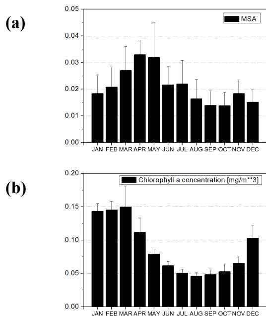
Figure 11. Monthly mean variation of (a) MSA - (μg m -3 ) and (b) chlorophyll a concentrations for the study period. Chlorophyll a concentrations were downloaded from the MODIS Aqua satellite over the region 140–145° E, 25–30° N for the study period.
