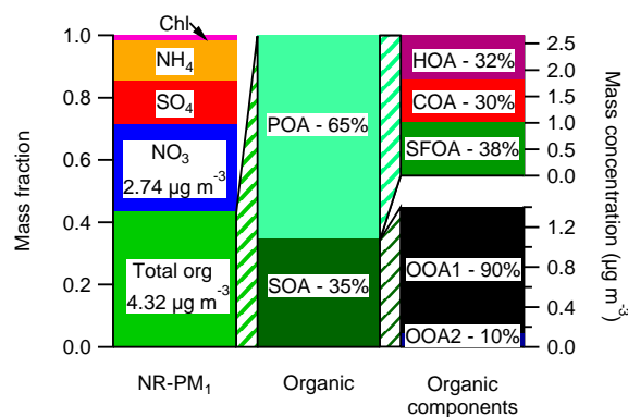
Figure 2. Left: average annual fractional contribution of all species to total NR-PM 1 . The average annual NR-PM 1 concentrations of SO 4 , NH 4 , and Chl were 1.39 , 1.30 , and 0.15 \mu\text{g m}^{-3} respectively. Middle: expansion of the organic fraction into its primary and secondary components following PMF analysis. Right top: expansion of the POA fraction into its three components. Right bottom: magnification of the SOA fraction showing its two subtypes. SFOA and OOA2 refer to SFOA mod and OOA2 mod respectively. See text in Sect. 4.4 for more details. Note that the organic data plotted in the middle and right bars do not include a period from the summer as discussed in Sect. 4.1 as well as Sects. 4.1 and 4.2 in the Supplement.
