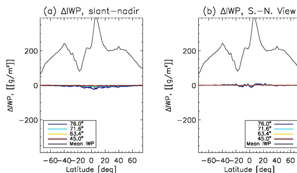
Figure 8. Ground-based view of (a) latitudinal distribution of JJA \Delta IWP between nadir and southward-looking view (solid lines), nadir and northward-looking views (dashed lines with the same color of solid lines). (b) Latitudinal distribution of JJA \Delta IWP between southward-looking and northward-looking views (solid color lines) integrated from 5 to 19 km. The black solid lines are the mean IWP at nadir. See Fig. 7 for viewing geometry.
