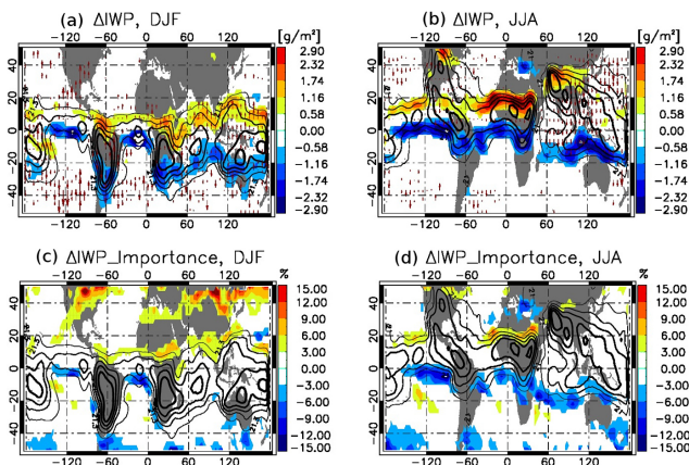
Figure 3. \Delta IWP (color shades; unit is \text{g m}^{-2} ) between the south view and the north view with view-angle of 77^\circ for December–January–February (a) and June–July–August (b) averaged during 2007–2010 between 11 and 17 km. Results are based on CloudSat IWC data set within \pm 50^\circ latitude range. The corresponding percentage difference of IWP (i.e., \Delta IWP/IWP, color shades; unit is %) is shown in (c) for DJF and (d) for JJA. The mean IWP within this altitude range is contoured in black with the contour interval equal to the minimum value shown on the contour line. Modern-Era Retrospective analysis for Research and Applications (MERRA) cloudy-sky meridional wind climatology during the same period is shown in arrow in (a) and (b) with wind speed linearly proportional to the arrow length. The longest arrow corresponds to 16 \text{ m s}^{-1} in (a) and 9.15 \text{ m s}^{-1} in (b). Data in the top panels are smoothed by a 2 \times 2 smoothing window.
