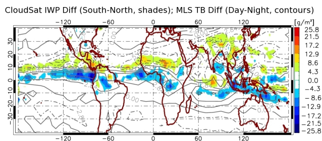
Figure 10. CloudSat \Delta IWP (color shades) and Aura MLS 640 GHz \Delta T_B (descending minus ascending orbits to mimic CloudSat viewing geometry, shown in contours; dashed is negative, solid is positive) for JJA, 2007–2010. The maps are interpolated to a 2^\circ \times 2^\circ grid box, and the correlation coefficient is -0.68 . Note that MLS has a shallower viewing angle, and it has a cloud diurnal cycle embedded in the signal.
