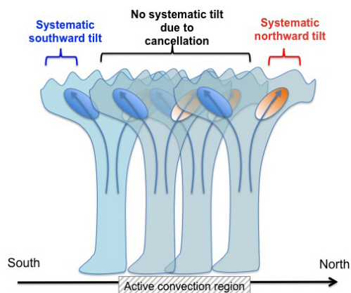
Figure 9. Schematic diagram showing the explanation of systematic poleward UT cloud tilts at the north and south peripheries of active tropical convection regions.
