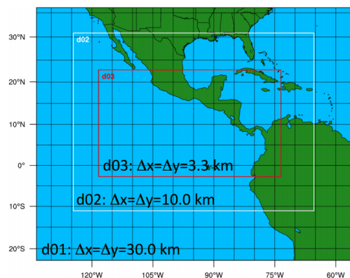
Figure 5. The domain map of WRF nested simulations.
