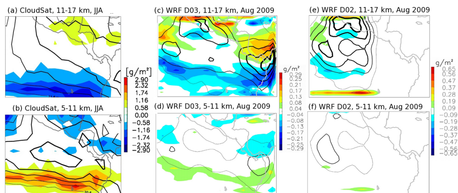
Figure 6. Climatological \Delta IWP (color shades) derived from CloudSat at 77^\circ view angle during JJA, 2007–2010 for ice clouds within 11–17 km (a) and 5–11 km (b), and the same variable derived from WRF D03 (c and d) and D02 (e and f) domains at 77^\circ view angle. The black contours mark the mean IWP integrated along the nadir view within the corresponding altitude range. Note that the magnitude of \Delta IWP from WRF run is much smaller than that from the CloudSat observations.
