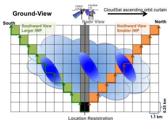
Figure 7. A diagram showing the computation geometry of the ground view.
