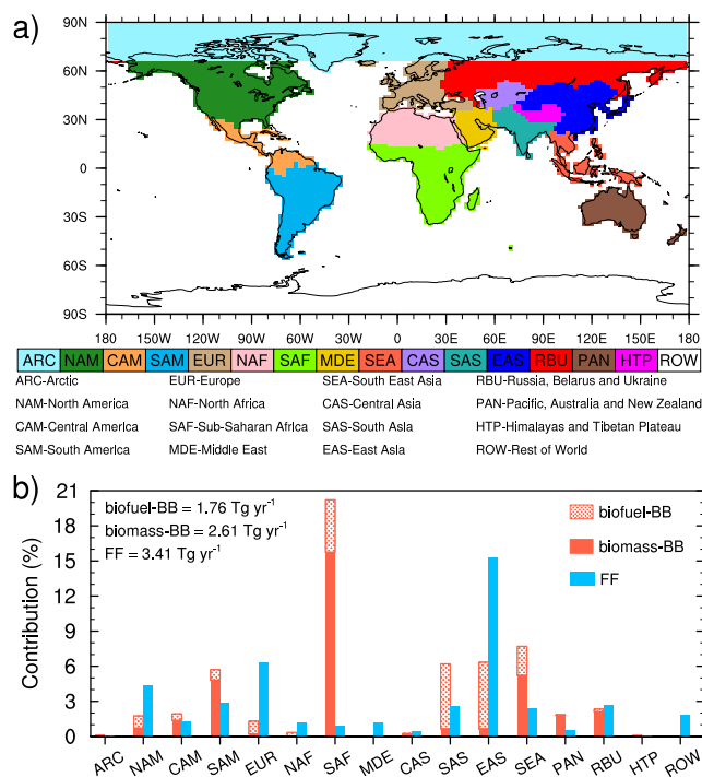
Figure 1. (a) Tagged source regions and (b) the respective percentage contributions to global annual mean BC emissions from the individual source regions and sectors (including biofuel, biomass burning, and fossil fuel). The global annual mean BC emission rate is 7.78 \text{ Tg yr}^{-1} , which is divided into the three sectors as indicated by the numbers in the upper-left corner.
