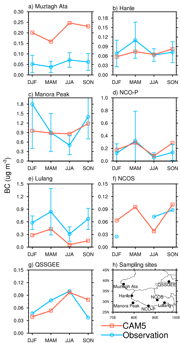
Figure 2. Seasonal mean surface BC concentration ( \mu\text{g m}^{-3} ) from observations (blue lines with error bars denoting SD) and CAM5 simulation (red lines) at the seven sampling sites listed in Table 1 and marked in the map of panel (h).
