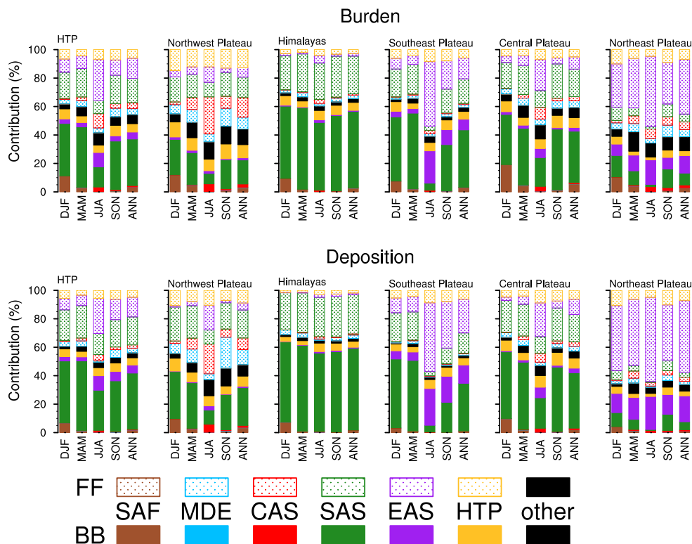
Figure 6. Fractional contributions (measured by the lengths of color bars) to seasonal and annual mean BC column burden (top six panels) and deposition (bottom six panels) over the HTP, northwest plateau, Himalayas, southeast plateau, central plateau, and northeast plateau, originating from six major tagged source regions (indicated by colors) for BB (solid bar) and FF (dotted bar) emissions. The black bar in each column represents the contribution from all of the other tagged source regions and sectors combined.
