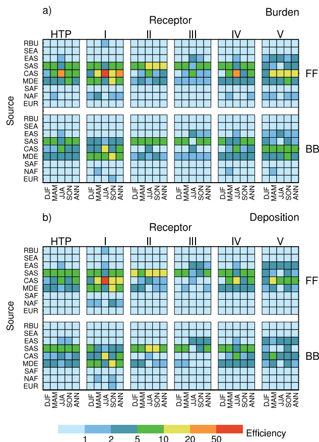
Figure 7. Efficiency of FF (top) and BB (bottom) emissions from 9 source regions (on the y axis) in changing seasonal and annual mean (a) BC column burden and (b) deposition over the HTP and each of the five subregions: northwest plateau (I), Himalayas (II), southeast plateau (III), central plateau (IV), and northeast plateau (V).
