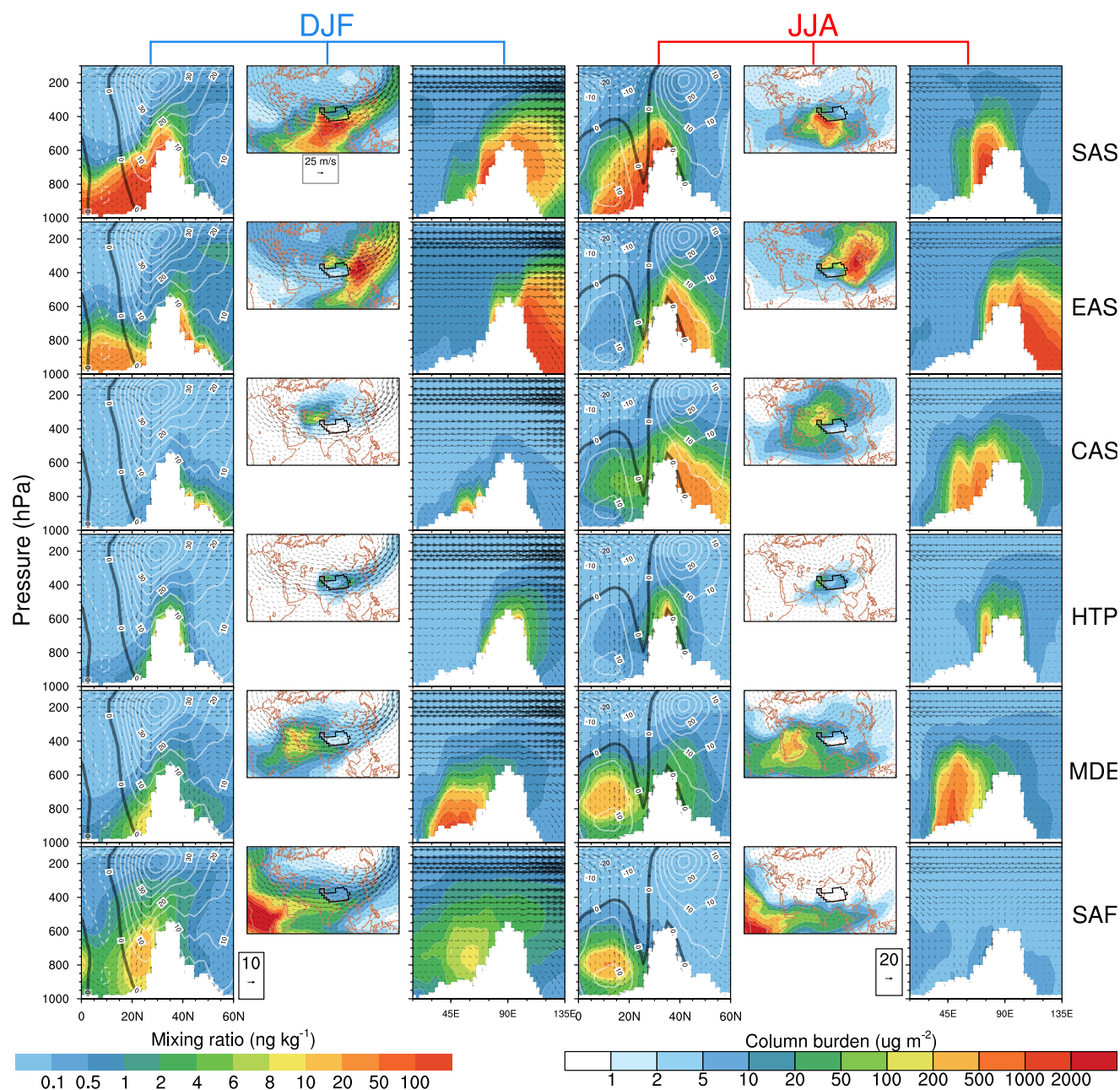
Figure 4. The first column shows the latitude–height distributions of DJF BC mass mixing ratios (in \text{ng kg}^{-1} , colors) averaged over 71.25\text{--}101.25^\circ\text{E} , originating from BB and FF sectors in the tagged source regions (corresponding to different rows); the white area denotes topography, and the superimposed white contours at intervals of 5\text{ m s}^{-1} represent the westerly (solid) and easterly (dashed) DJF mean zonal winds along the cross section with the thick solid black contour at 0\text{ m s}^{-1} ; the wind vectors (consisting of vertical velocity in units of -10^{-4}\text{ hPa s}^{-1} and meridional wind in \text{m s}^{-1} ) are represented by arrows. Colors in the second column denote spatial distribution of the DJF mean BC column burden (in \mu\text{g m}^{-2} ), originating from different source regions, and the arrows represent the DJF mean horizontal wind vectors at 500 hPa; the HTP is marked with a black outline. The third column is similar to the first column except that the quantities are on the longitude–height cross section averaged over 28\text{--}40^\circ\text{N} , and thus the horizontal component of the wind vectors is zonal wind ( \text{m s}^{-1} ) instead. The fourth to sixth columns are the same as the first to third columns, respectively, but for JJA means instead.
