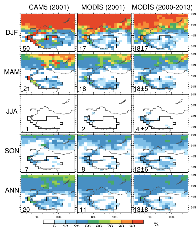
Figure 3. Seasonal and annual mean snow cover fraction from CAM5 simulation for year 2001 (left), and MODIS retrieval for 2001 (middle) and 2000–2013 (right). The summer (JJA) in 2001 for both CAM5 and MODIS only includes July and August due to missing MODIS data in June. The number in the lower-left corner of each panel is the corresponding spatial mean SCF for the HTP region (which is marked with a black outline), and for MODIS the standard deviation calculated from the MODIS multi-year means is also included.
