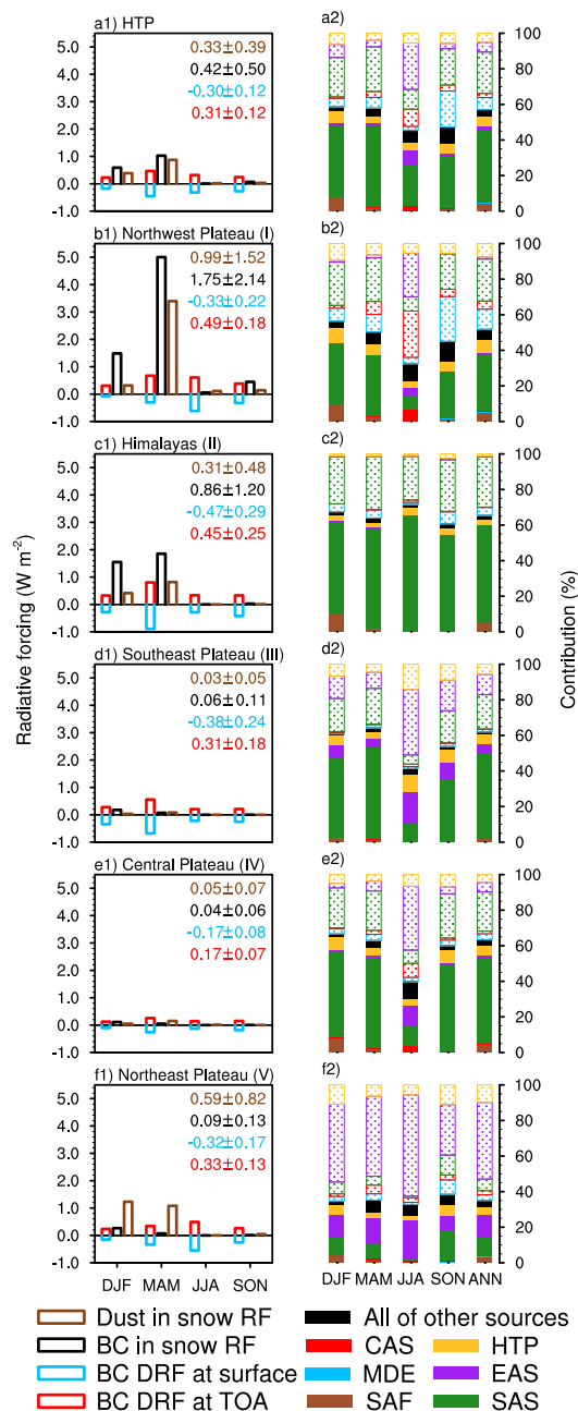
Figure 8. Seasonal mean radiative forcing (left column) induced by the various BC effects (indicated by the color legend at the bottom) and dust-in-snow effect over (a1) the HTP, (b1) northwest plateau, (c1) Himalayas, (d1) southeast plateau, (e1) central plateau, and (f1) northeast plateau. The corresponding annual mean forcings and one SD (for 12 monthly means) are shown in numbers on the top-right corner of each panel. The right column (a2–f2) panels represent source contribution to surface BC-in-snow radiative forcing over the corresponding receptors from tagged source regions (colors) and sectors (solid pattern bar and dotted pattern bar for BB and FF, respectively). The black bar in each column represents the contribution from all of the other tagged source regions and sectors.
