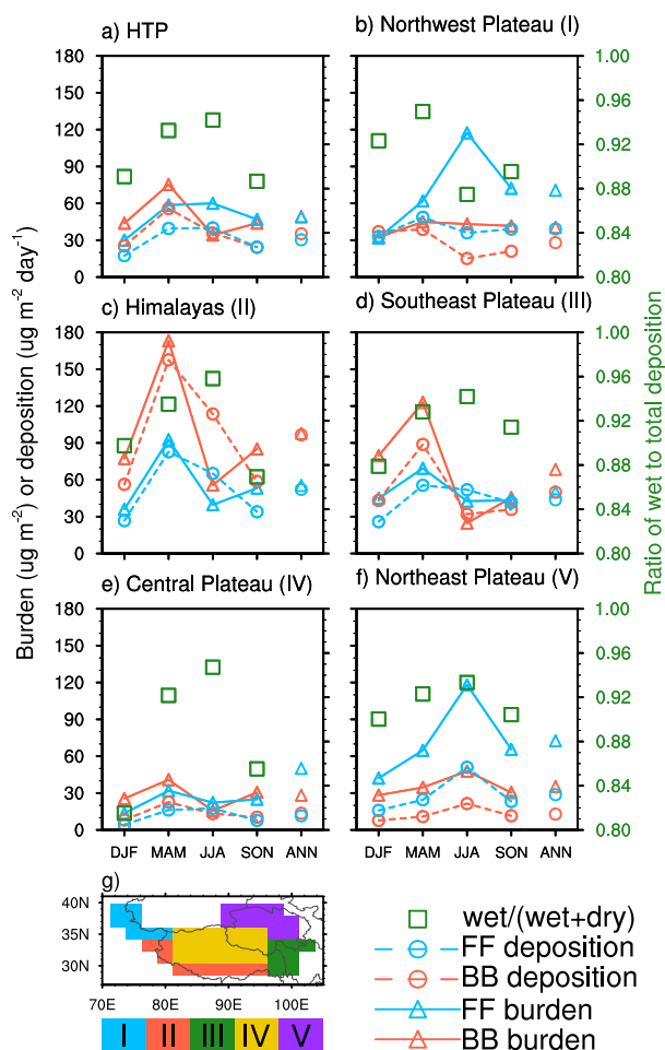
Figure 5. Seasonal and annual mean BC column burden (solid lines and open triangles, in \mu\text{g m}^{-2} ) and deposition rate (dashed lines and open circles, in \mu\text{g m}^{-2} \text{day}^{-1} ) over (a) the HTP, (b) northwest plateau, (c) Himalayas, (d) southeast plateau, (e) central plateau and (f) northeast plateau, emitted from BB (red) and FF (blue) source sectors. The green squares denote the ratio of wet to total BC deposition (using y axis on the right) in four seasons over each receptor region. The geographical locations of five subregions of HTP are indicated in panel (g).
