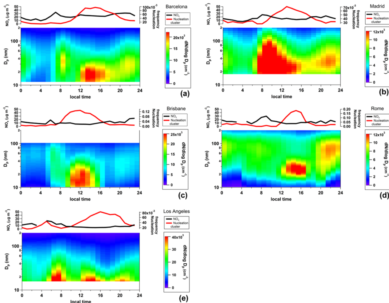
Figure 5. Mean SMPS size distributions on a nucleation day at each selected city, NO x average concentration and the frequency of occurrence of the Nucleation cluster for: (a) Barcelona, (b) Madrid, (c) Brisbane, (d) Rome and (e) Los Angeles. Please note that NO x concentrations for Madrid represent NO x /2 and for Los Angeles NO x /10. These values are 30–65 % lower on nucleation days than the corresponding sampling period average levels.
