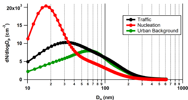
Figure 4. Average aerosol size distributions for the main k -means cluster category: Traffic, Nucleation and Urban Background. Only the main cities BCN, MAD and BNE were considered.
