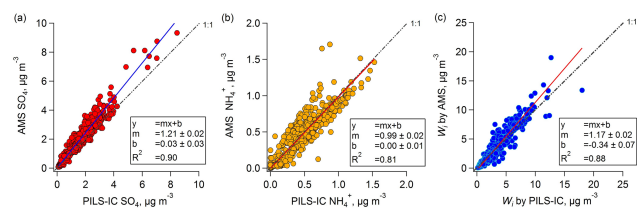
Figure 2. Comparisons of \text{PM}_{10} AMS sulfate, ammonium to \text{PM}_{10} and \text{PM}_{2.5} PILS-IC (i.e., complete SOAS study) and predicted W_i . Orthogonal distance regression (ODR) fits were applied.
