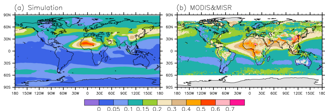
Figure 1. Global distributions of simulated and observed annual mean aerosol optical depth (AOD) at 550 nm. (a) Simulation and (b) MODIS&MISR (van Donkelaar et al., 2010).
