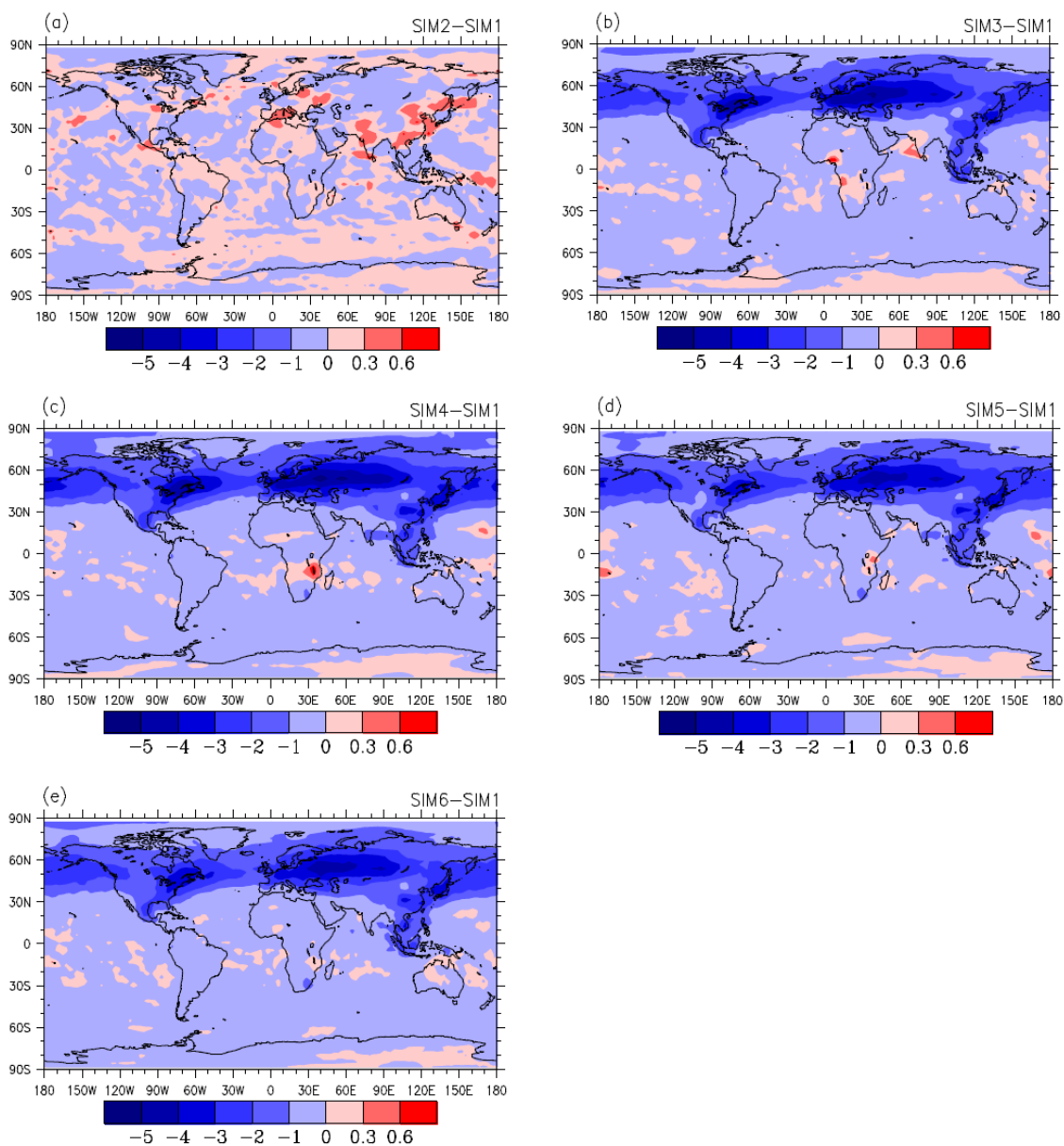
Figure 5. Global distributions of difference in simulated annual mean column CDNC (units: 10^{10} \text{ m}^{-2} ). (a) SIM2–SIM1, (b) SIM3–SIM1, (c) SIM4–SIM1, (d) SIM5–SIM1, and (e) SIM6–SIM1.
