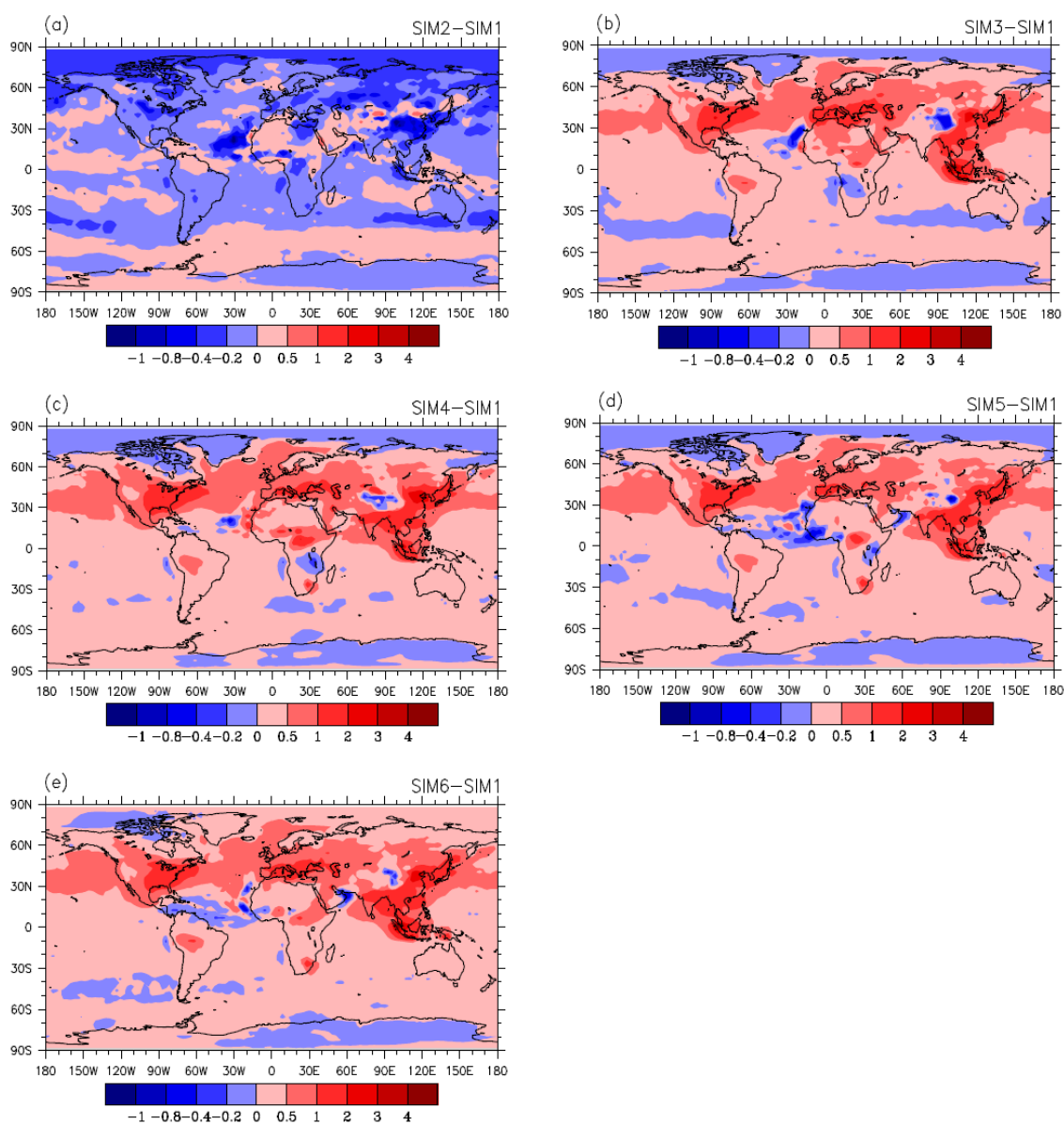
Figure 3. Global distributions of difference in simulated annual mean aerosol direct effect (units: \text{W m}^{-2} ). (a) SIM2–SIM1, (b) SIM3–SIM1, (c) SIM4–SIM1, (d) SIM5–SIM1, and (e) SIM6–SIM1.
