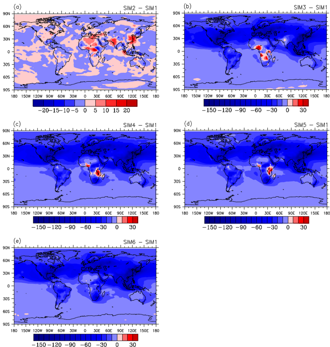
Figure 4. Global distributions of difference in simulated annual mean CCN concentration at surface (units: \text{cm}^{-3} ). (a) SIM2–SIM1, (b) SIM3–SIM1, (c) SIM4–SIM1, (d) SIM5–SIM1, and (e) SIM6–SIM1.
