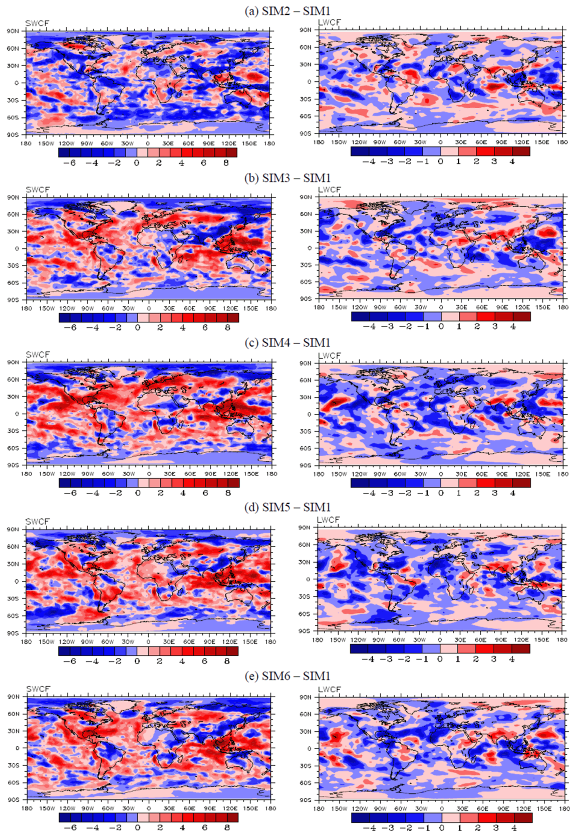
Figure 6. Global distributions of difference in simulated annual mean SWCF and LWCF (units: \text{W m}^{-2} ). (a) SIM2–SIM1, (b) SIM3–SIM1, (c) SIM4–SIM1, (d) SIM5–SIM1, and (e) SIM6–SIM1.
