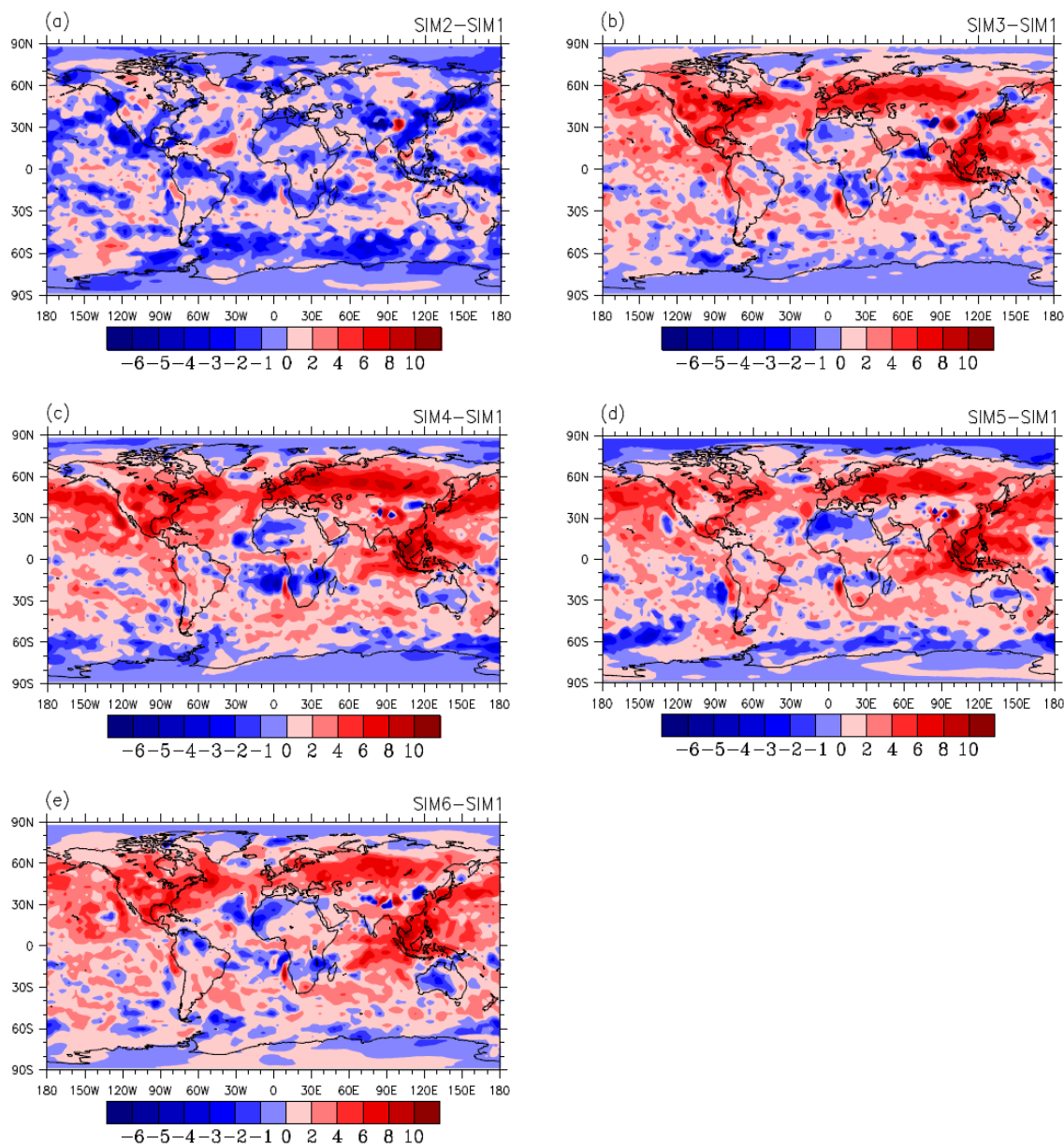
Figure 7. Global distributions of difference in simulated annual mean aerosol net effect (units: \text{W m}^{-2} ). (a) SIM2–SIM1, (b) SIM3–SIM1, (c) SIM4–SIM1, (d) SIM5–SIM1, and (e) SIM6–SIM1.
