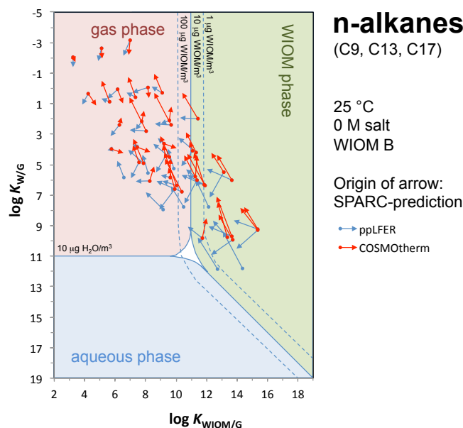
Figure 5. Arrows indicating the uncertainty of chemical placement in the partitioning space based on the discrepancy of K_{WIOM/G} and K_{W/G} predictions made with SPARC (origin of arrows), ppLFRs (tip of blue arrows) and COSMOtherm (tip of red arrows). For some compounds, no COSMOtherm predictions are available.
