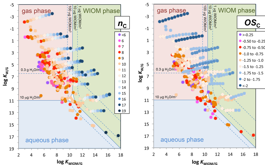
Figure 3. Same as Fig. 2, except that markers are coloured based on a chemical's number of carbon atoms ( n_C ) (left) or its average carbon oxidation state ( OS_C ) (right).
