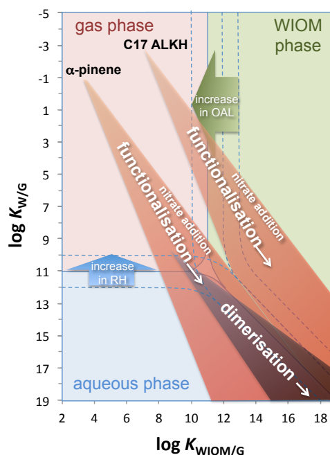
Figure 11. Visualisation in the partitioning space of processes occurring during the oxidation of VOC precursors in a chamber experiment or a photochemical smog episode (in the presence of water). While the addition of functional groups and dimerisation reactions lead to an increase in K_{\text{WIOM}/\text{G}} and K_{\text{W}/\text{G}} and therefore a gradual shift to the lower right, the attendant increase in the organic aerosol load shifts the threshold for the gas–WIOM transition to the left.
