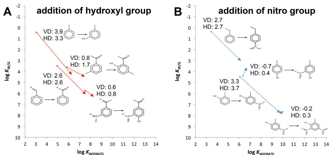
Figure 9. Displacement in the chemical partitioning space occurring upon the addition of a hydroxyl (a) or nitro (b) group to a mono-aromatic hydrocarbon, as predicted by SPARC for 15 °C and using structure B for WIOM (VD: vertical displacement; HD: horizontal displacement).
