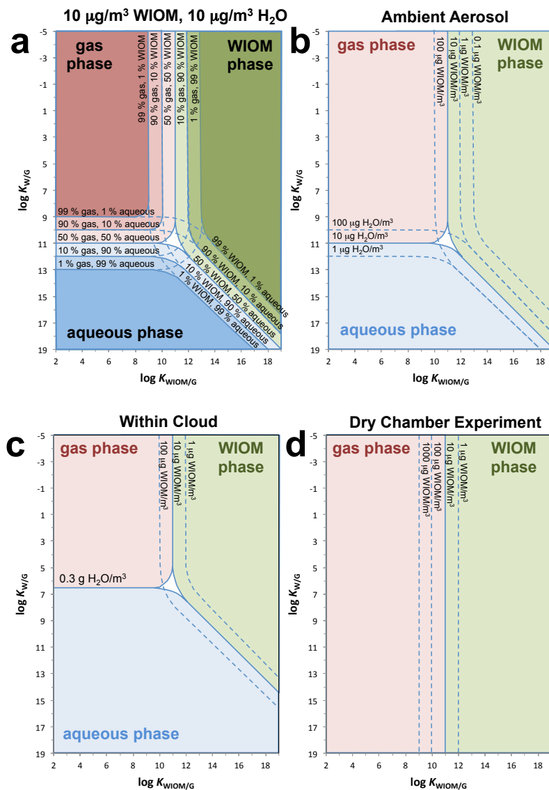
Figure 1. Different versions of the chemical partitioning space for the atmosphere, showing in red, blue and green the combinations of partitioning properties that lead to dominant equilibrium partitioning to the gas, aqueous and water-insoluble organic matter (WIOM) phase, respectively. Panel (a) refers to typical atmospheric conditions of 10 \mu\text{g} of both WIOM and liquid water per \text{m}^3 of air and demonstrates that the transition from 1 (10) to 99 (90)% in a particular phase occurs over a 4 (2) order of magnitude range in a partition coefficient. A clear atmosphere (a and b), a cloud (c) and a dry chamber experiment (d) only differ in terms of the relative volume of the three phases present, leading to shifts in the thresholds indicating 50% partitioning into any one phase. Dashed lines in (b)–(d) indicate the 50% threshold for various loadings of WIOM and various liquid water contents.
