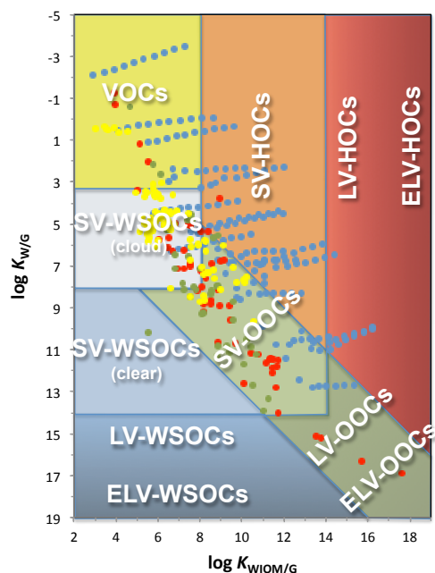
Figure 4. Same as Fig. 2, except that different regions of the chemical partitioning space have been named according to the type of compounds that fall into these regions.
