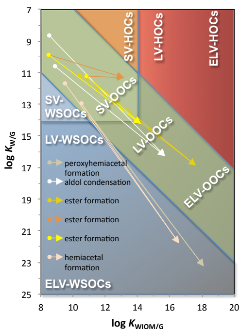
Figure 10. Displacements in the chemical partitioning space due to various dimerisation reactions proposed for ozonolysis reaction products of \alpha -pinene by Camredon et al. (2010). K_{\text{WIOM}/\text{G}} and K_{\text{W}/\text{G}} at 15 °C were estimates with SPARC using structure B as a surrogate for WIOM. Also shown is the categorisation into compounds with different atmospheric phase distribution behaviour introduced in Fig. 4.
