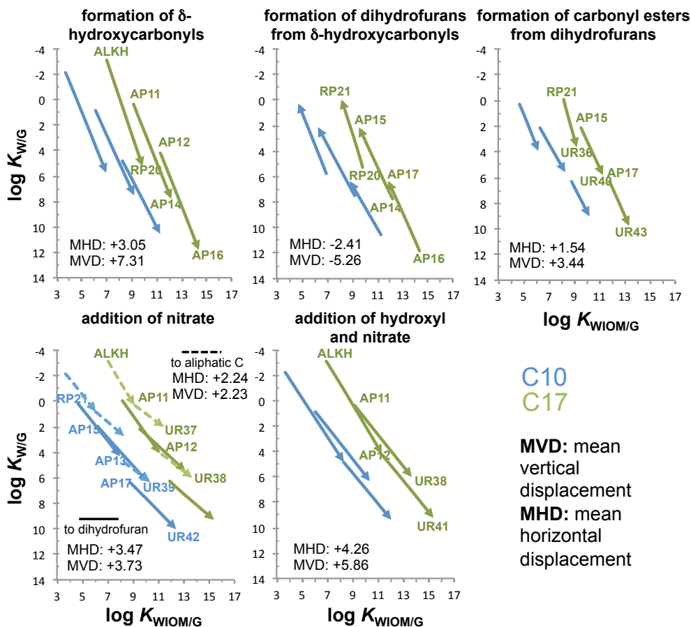
Figure 8. Displacement of chemicals in the partitioning space caused by transformations involved in the oxidation of n -alkanes with 10 (blue) and 17 (green) carbons using predictions of K_{W/IOM/G} and K_{W/G} at 25 °C obtained by ppLFER. Also given are the mean vertical displacement (MVD) and mean horizontal displacement (MHD).
