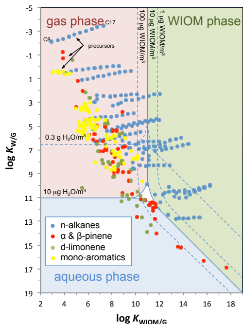
Figure 2. Placement of the selected oxidation products of n -alkanes, biogenic terpenes and mono-aromatic hydrocarbons in the partitioning space. K_{\text{WIOM/G}} and K_{\text{W/G}} at 15 °C and 0 M salt of the compounds were estimated using SPARC assuming the solvation properties of WIOM can be approximated by those of structure B.
