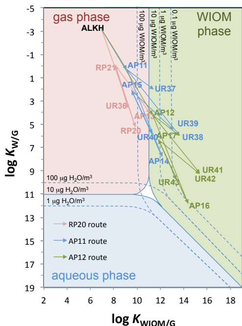
Figure 7. Oxidation products of the n -alkane with 17 carbon atoms placed within the chemical partitioning space based on partition coefficients at 25 °C predicted with ppLFRs and connected by arrows based on sequence of reaction by which they are formed. The code names for the compounds are based on Jordan et al. (2008).
