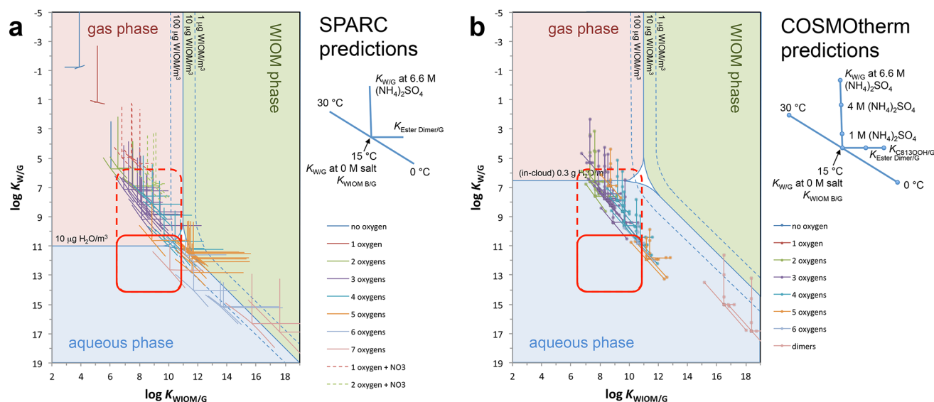
Figure 6. Placement of \alpha -pinene and some of its oxidation products in the chemical partitioning space based on predictions with SPARC (a) and COSMOtherm (b). Each chemical is represented by three lines, which account for the influence of temperature variations between 0 and 30 °C (diagonal line), the salting-out effect by 6.6 M (\text{NH}_4)_2\text{SO}_4 (vertical line) and the polarity of the surrogate representing the solvation properties of WIOM (horizontal line). The chemicals are superimposed on the dominant phase distribution maps for wet aerosol (a) and a cloud (b). The red lines encircle regions where chemicals fall whose contribution to SOA formation would not be considered if the aqueous phase in an aerosol (solid line) or cloud (dashed line) were ignored.
