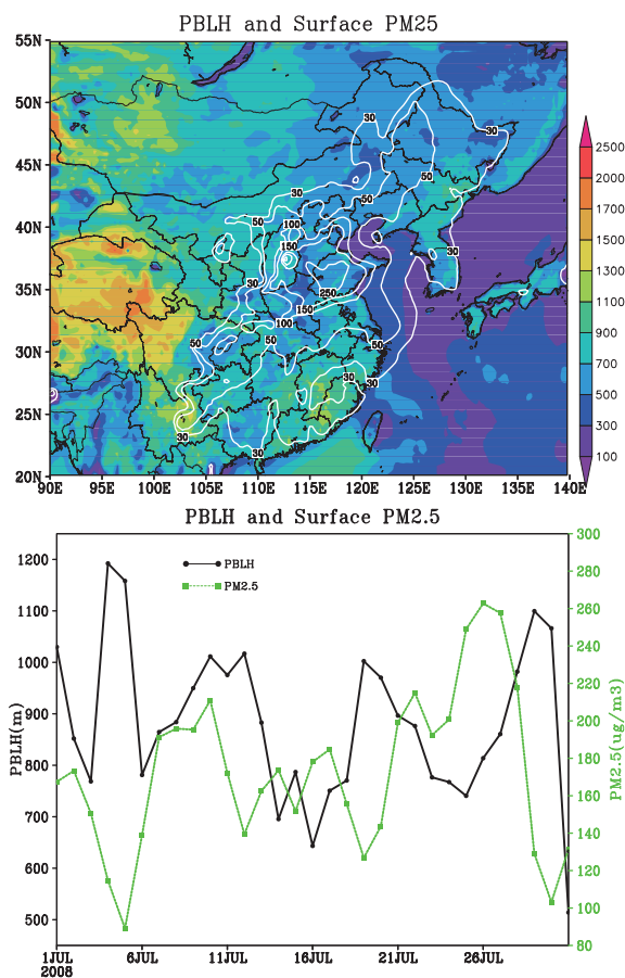
Figure 8. The mean surface PM 2.5 ( \mu\text{g m}^{-3} , contours) and PBL height (m, shaded) for 7–11 July 2008 (top), and daily changes in the 3JNS mean surface PM 2.5 and PBL height (bottom).
