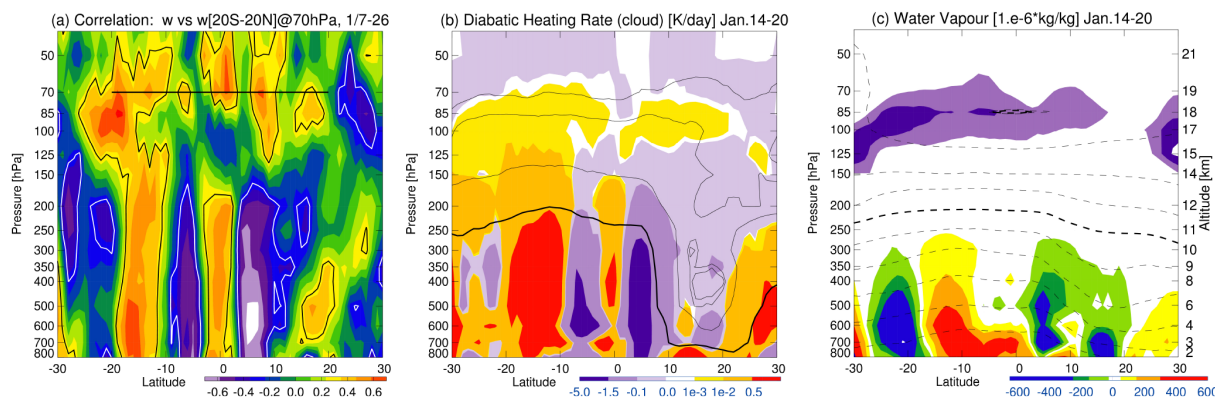
Figure 3. (a) Latitude–pressure sections of correlation between the vertical wind averaged over 20° S–20° N at 70 hPa (thick line) and vertical wind at each level and latitude for the period of 7–26 January. Latitude–pressure sections of (b) latent heating rate due to cloud formation ( \text{K day}^{-1} ) (contours) and (c) the water vapour concentration ( 10^{-6} \text{ kg kg}^{-1} ) (dashed contours) averaged between 14 and 20 January. The thin contours in (b) are values of 10^{-3} \times 10^i ( i = 0, 1, 2 ) ( \text{K day}^{-1} ). The thick contour is 1.0 ( \text{K day}^{-1} ). The dashed contours in (c) are values of 10^4 \times 10^{i/3} ( i = 0, 1, 2, \dots, 10 ) ( 10^{-6} \text{ kg kg}^{-1} ); the thick dashed contours indicate 4.6 and 100 ( 10^{-6} \text{ kg kg}^{-1} ). Anomalies with respect to the 7–13 January average are shown by colour shading. The light and heavy purple in (c) indicate values of -0.3 ( 10^{-6} \text{ kg kg}^{-1} ) and below and -0.6 ( 10^{-6} \text{ kg kg}^{-1} ) and below, respectively.
