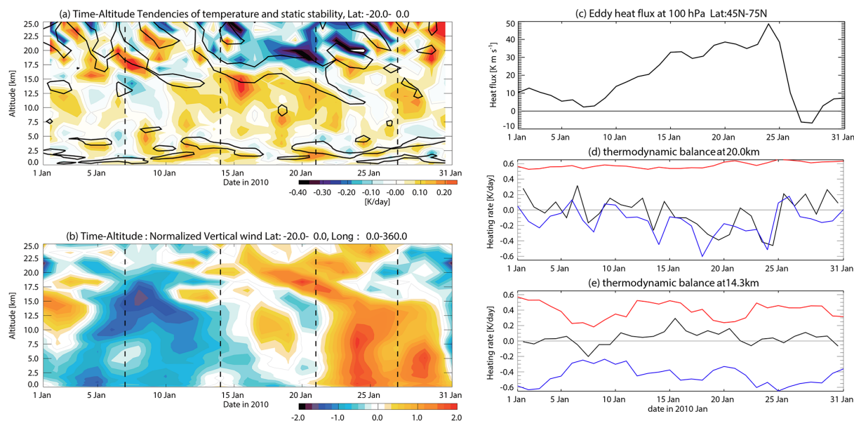
Figure 4. Time–altitude section of (a) temperature tendency ( \text{K day}^{-1} ) (colour shading) and tendency of static stability with value of -0.02 ( 10^{-4} \text{ s}^{-2} \text{ day}^{-1} ) shown by black contours and (b) anomalous normalized vertical velocity averaged between 20^\circ \text{ S} and equator from 1 to 31 January 2010. The normalized values are obtained by dividing them by the standard deviation at each altitude. (c) Time series of zonal mean eddy heat flux ( \text{K m s}^{-1} ) at 100 hPa averaged between 45^\circ \text{ N} and 75^\circ \text{ N} . Panels (d, e) show the time series of thermodynamic balance at 14.3 and 20.0 km averaged between 20^\circ \text{ S} and Equator. The black, red and blue lines indicate temperature tendency ( \partial T/\partial t ), diabatic heating rate due to cloud microphysics and radiation, and adiabatic heating rate due to residual vertical velocity ( -N^2\omega^* ), respectively.
