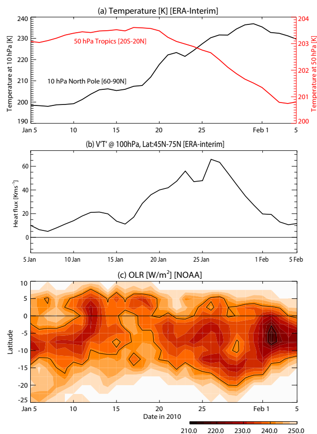
Figure 1. (a) Time series of observed zonal mean temperature (K) in the northern high latitude at 10 hPa (black line) and tropical at 50 hPa (red line) from 5 January to 5 February 2010. Note the different temperature scales for the polar (left) and tropical (right) regions. (b) Time series of observed zonal mean eddy heat flux ( \text{K m s}^{-1} ) at 100 hPa averaged between 45^\circ\text{N} and 75^\circ\text{N} . (c) Time–latitude ( 25^\circ\text{S} – 10^\circ\text{N} ) section of NOAA observed zonal mean OLR ( \text{W m}^{-2} ). The horizontal line indicates the equator.
