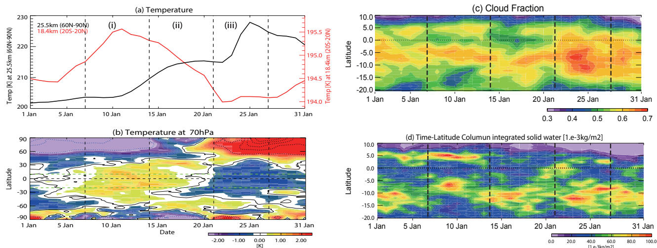
Figure 2. (a) Same as Fig. 1a but for simulated zonal mean temperature from 1 to 31 January 2010. (b) Time–latitude ( 90^{\circ} N– 90^{\circ} S) section of simulated temperature anomaly (K) at 70 hPa with respect to the January 2010 monthly mean at each latitude. The solid contour indicates zero anomaly and the dotted contours indicate -2.5 K and 2.5 K. The light green horizontal dashed lines indicate the latitudinal region of (c) and (d). (c) Time–latitude ( 20^{\circ} S– 10^{\circ} N) section of simulated zonal mean column-integrated cloud fraction. (d) Same as (c) but for column-integrated ice cloud ( 10^{-3} kg m ^{-2} ). The four vertical dashed lines in (a–d) are 7, 14, 21 and 27 January; the periods between the lines are the (i) initial, (ii) transition and (iii) mature phases. The horizontal dashed lines in (b, c and d) indicate the equator.
