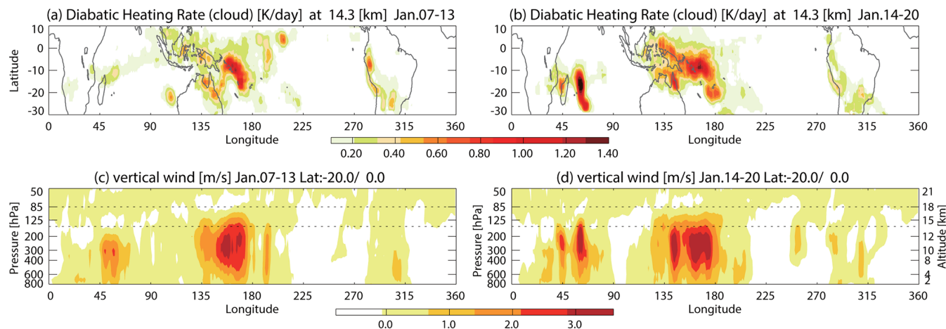
Figure 5. Maps of diabatic heating rate from cloud microphysics ( \text{K day}^{-1} ) at 14.3 km ( a , b ) averaged over 7–13 January (left, a ) and 14–20 January (right, b ). The panels ( c , d ) show longitude–pressure sections of vertical wind ( \text{m s}^{-1} ) averaged between 20^\circ\text{S} and equator on 7–13 and 14–20 January, respectively. The vertical wind data are smoothed by applying a weighting function of five-degree-longitude width. The horizontal dotted lines in ( c , d ) show the 85 hPa and 150 hPa pressure levels for reference.
