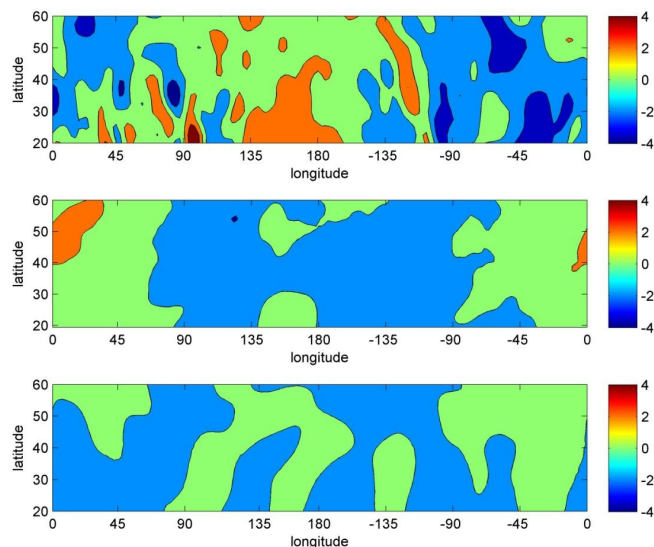
Figure 3. The same as Fig. 1 but for July. Positive values (poleward wind): red; negative values (equatorward wind): blue.
