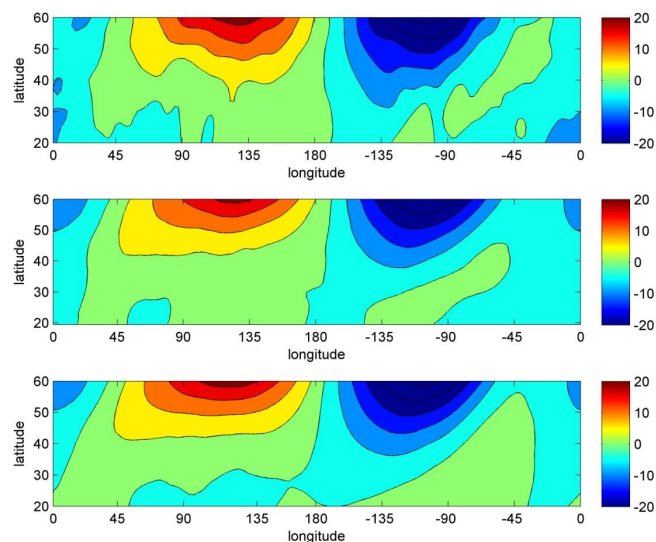
Figure 1. Plot of average meridional wind speed ( \text{m s}^{-1} ) component for January at 20–60° N, 180° E–180° W and 10 hPa. Top panel NCEP/NCAR (1958–2012), middle ERA-Interim (1979–2012), and bottom MERRA (1979–2012). Positive values (poleward wind): red; negative values (equatorward wind): blue.
