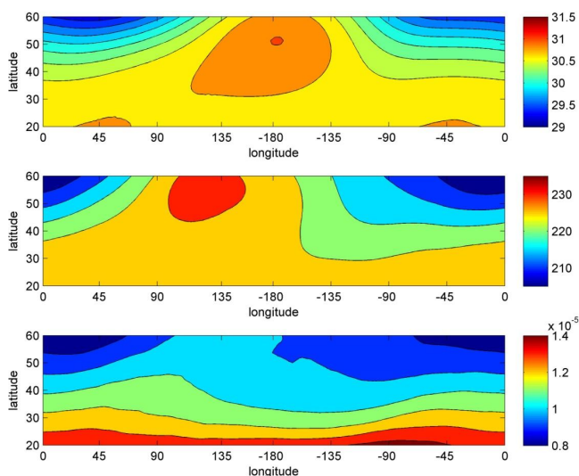
Figure 7. Plot of average geopotential height (km, top panel), temperature (K, middle panel) and ozone mixing ratio (ppmv, bottom panel) for January at 20–60° N, 180° E–180° W and 10 hPa.
