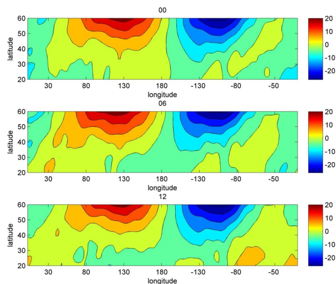
Figure 4. Plot of average meridional wind speed ( \text{m s}^{-1} ) component at 10 hPa for January 1958–2012 at 20–60° N, 180° E–180° W. Top panel: 00:00 UTC; middle: 06:00 UTC; bottom: 12:00 UTC. Positive values (poleward wind): red; negative values (equatorward wind): blue. NCEP/NCAR reanalysis only.
