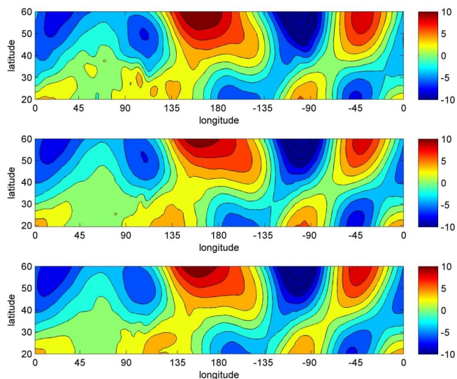
Figure 2. The same as Fig. 1 but for 100 hPa.
