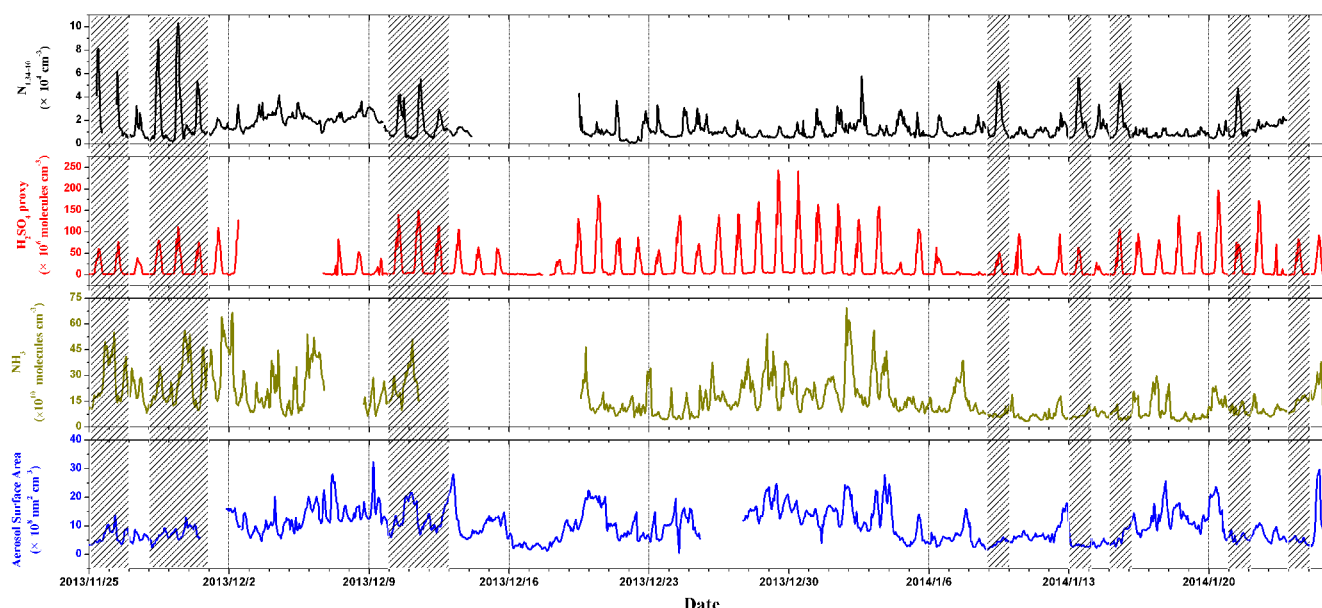
Figure 7. Number concentrations of 1.34–10 nm particles ( N_{1.34\sim 10} ), sulfuric acid proxy ( [H_2SO_4] ), concentrations of ammonia, and aerosol surface area during the campaign. NPF events are illustrated with shadows.
