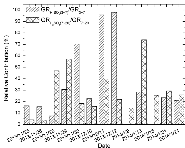
Figure 6. Relative contribution of sulfuric acid to growth of particles in the range of 3–7 and 7–20 nm, respectively, on each NPF day.
