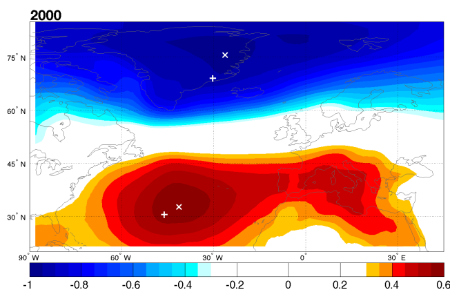
Figure A1. Correlations between North Atlantic winter SLP (December–February) and the PC1 of SLP. The markers indicate the maxima in CI (+ sign) and in the SLP/PC1 (x sign) correlations.
