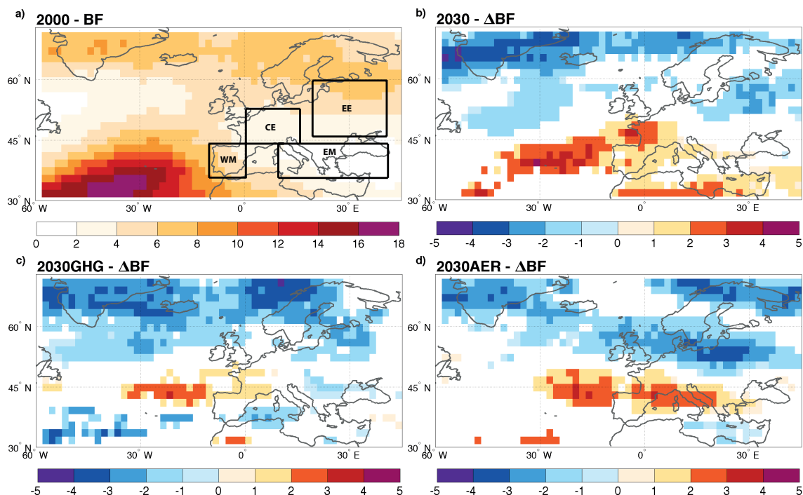
Figure 3. Blocking frequency (in % of days in which a blocking event occurs at a given gridbox) over the Atlantic sector for the 2000 simulation (a); changes in blocking frequency compared to the 2000 simulation for 2030 (b), 2030GHG (c) and 2030AER (d) simulations in winter (DJF). Only areas in which the difference between the 2000 control and the sensitivity simulation is significant at 95 % confidence level are shaded (in white non-significant areas). In panel (a) we have highlighted the regions discussed in Sect. 3.3 and Table 2.
