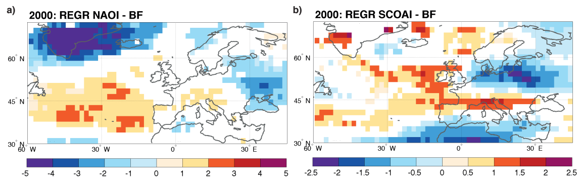
Figure 4. Blocking frequency anomalies (in % of days in which a blocking event occurs at a given gridbox) per unit of NAO index (NAOI, a) and SCOAI index (SCOAI, b) standard deviation. The anomalies are calculated using a one-point regression analysis (see Appendix B). Only differences significant at 95 % confidence level are shown (based on the correlation significance between NAOI/SCOAI and blocking frequency). Note that the two panels use different colour scales.
