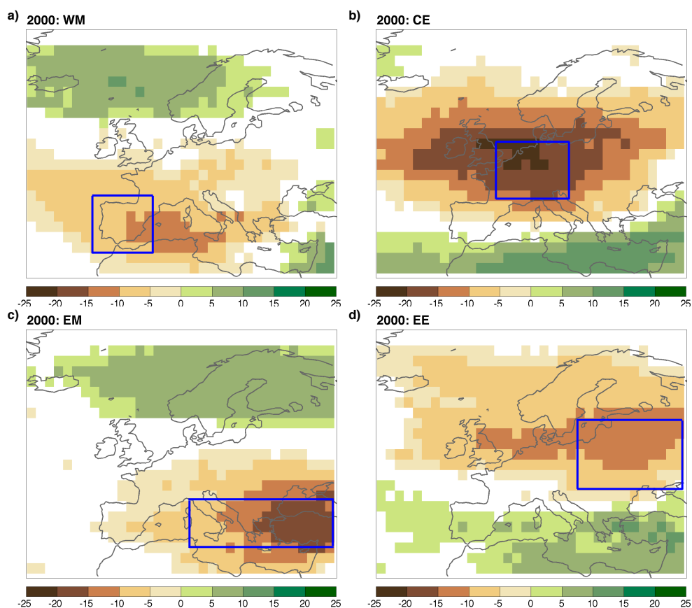
Figure B2. The values at each grid point show the composite anomaly in rainy days (in %) in the selected domain – WM (a), CE (b), EM (c), EE (d) – while said grid point is blocked compared to the case where said grid point is unblocked. The composite is taken by averaging the rainy day anomaly maps obtained for each gridbox within the selected domain. For example, in panel (a) (WM) the positive values over southern Norway indicate that, when there is a blocking event there, rainy days over the WM increase by about 10 % compared to the case with no blocking over southern Norway. On the other hand, blocking events west and over the WM lead to 10–15 % precipitation anomalies relative to the case with no blocking events over the same regions. The regional domains analysed in each panel are marked by the blue rectangles.
