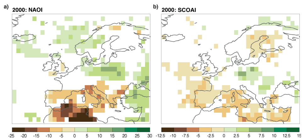
Figure B1. Rainy day anomalies (in %) per unit of NAOI (a) and CI time series (b) standard deviation. The CI time series has been constructed as described in Appendix B. The anomalies are calculated using a one-point regression analysis. Only differences significant at the 95 % confidence level are shown. Note that the two panels use different colour scales.
