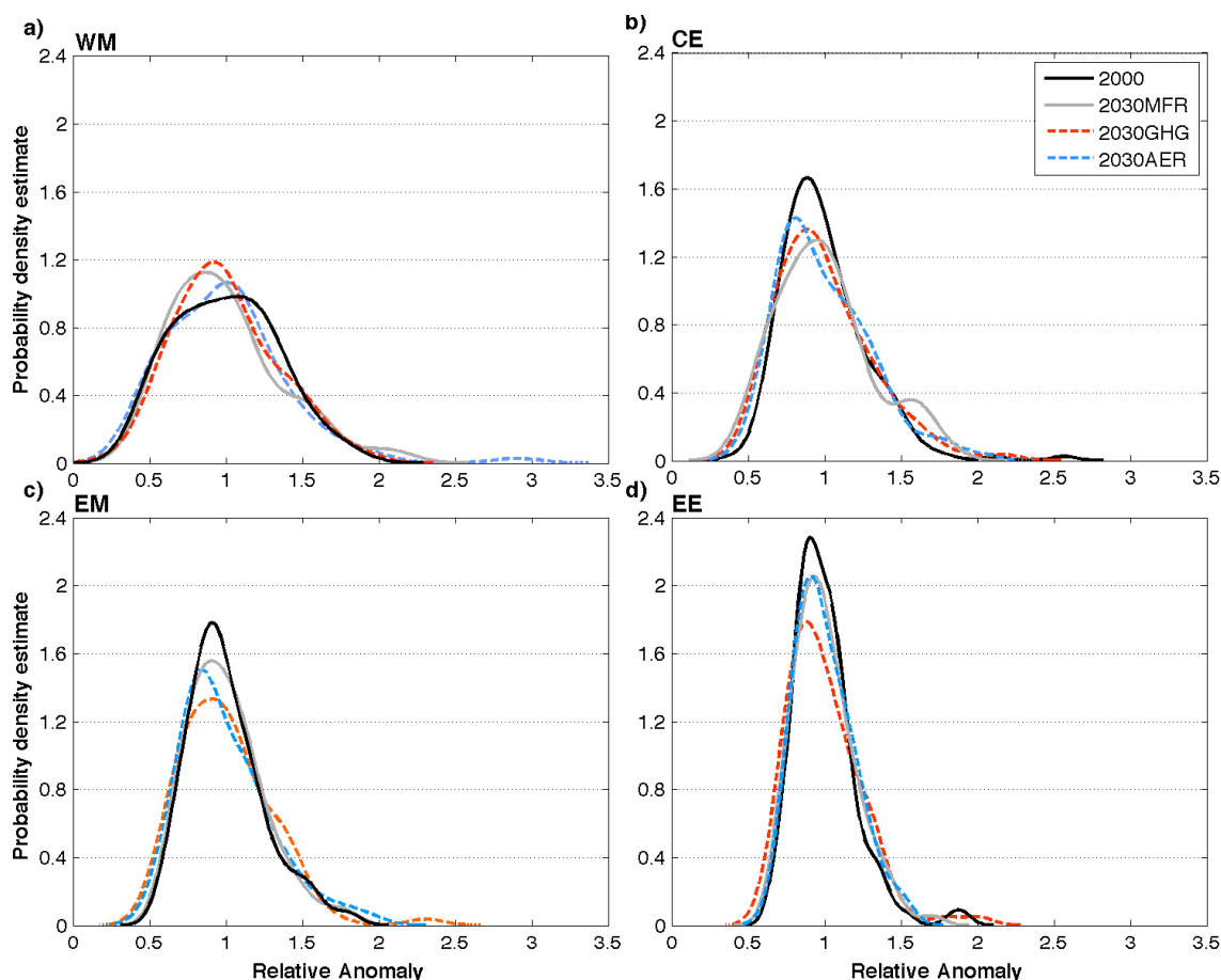
Figure 5. Probability density estimates (PDEs) of PM relative anomalies for each region (Western (a) and Eastern Mediterranean (c), Central (b) and Eastern Europe (d)) and for each experiment. Relative anomalies are computed as the ratio between winter (DJF) monthly time series and the winter (DJF) climatology of each experiment and region. The probability density estimates are based on a normal kernel function, which provides non-parametric PDEs for random variables (Rosenblatt, 1956). The probability for a given relative anomaly to occur is obtained by integrating the PDE in dx .
