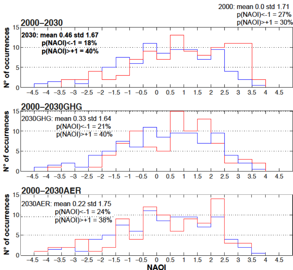
Figure 2. Frequency distributions of the winter (DJF) NAOI for the 2000 control simulation (blue, all panels), 2030 (red, upper panel), 2030GHG (red, central panel) and 2030AER (red, lower panel). Numbers show the NAOI mean value, the standard deviation (SD) and the probability of having a NAOI greater than +1 ( p(\text{NAOI}) > +1 ) or smaller than -1 ( p(\text{NAOI}) < -1 ). Values of the simulations having a NAOI mean significantly different from 2000 control mean at 95 % confidence level are shown in bold. The 2000s mean NAOI is by definition equal to 0 and the number of occurrences has been normalized to 30 years for a direct comparison with the other simulations.
