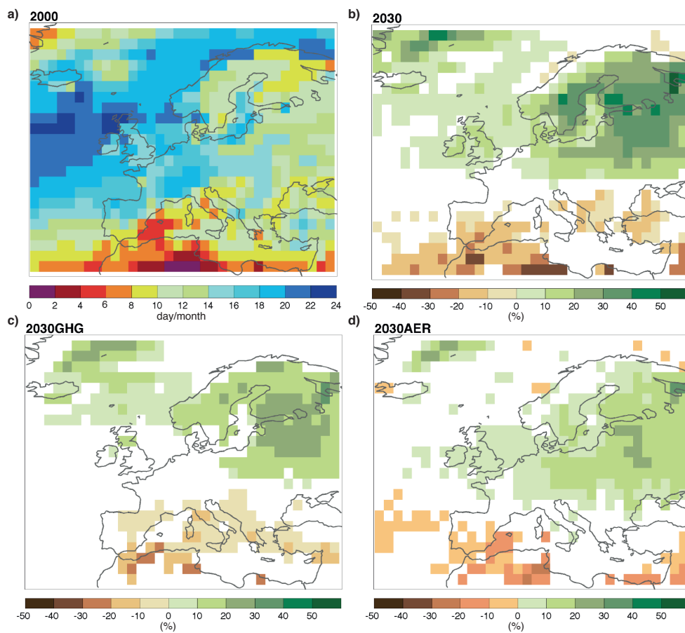
Figure C1. Average number of rainy days per month during winter (DJF) in the 2000 simulation (a). Percentage changes in the average number of rainy days per month for 2030 (b), 2030GHG (c), and 2030AER (d) simulations during winter. Only differences significant at the 95 % confidence level are shown.
