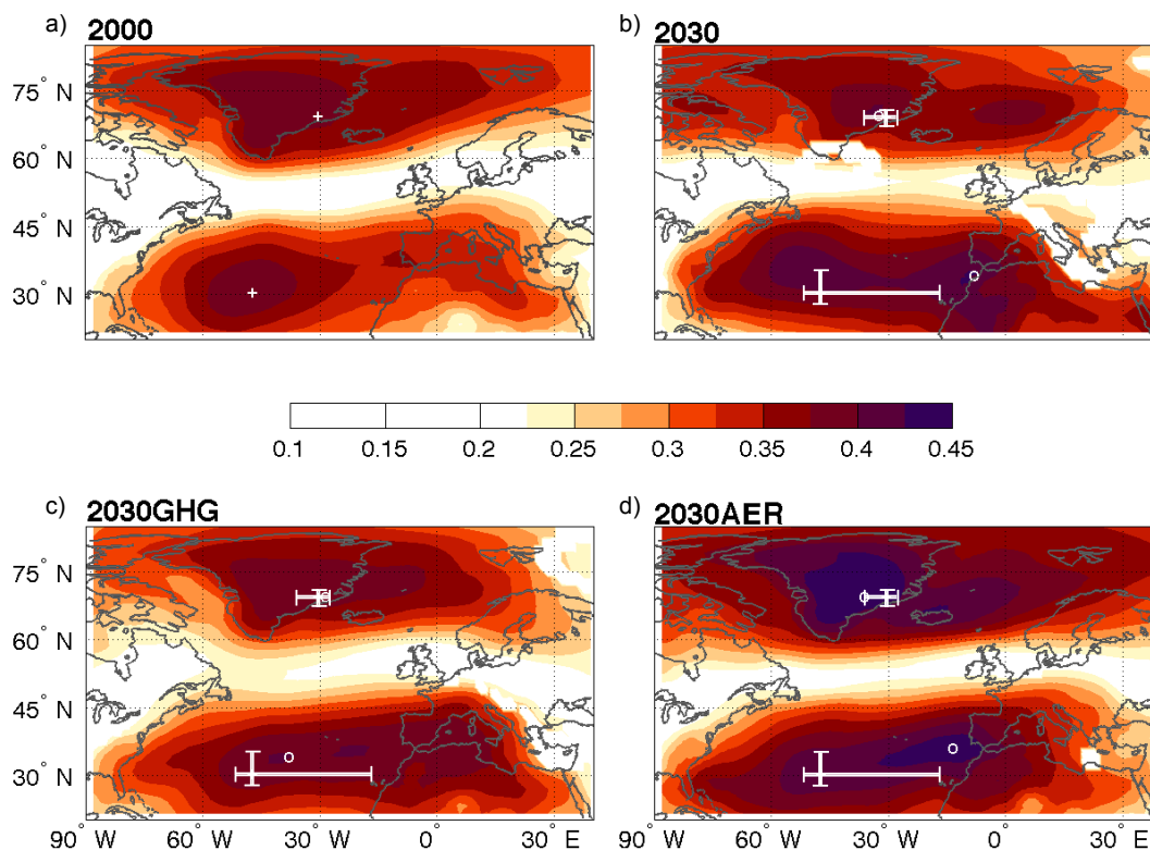
Figure 1. Sea-level pressure coherence index maps of the North Atlantic sector for the 2000 (a) and 2030 (b) simulations and the two sensitivity studies (c, d) in winter (DJF). The SLP centres of action (COAs) for the control run and for the 2030 simulations are shown by white crosses and white circles, respectively. The bars delimit the range between the 10th and 90th percentile of the CI maxima in the 2000 simulations. Only areas in which the difference between the 2000 control pattern and the sensitivity simulation is significant at the 95 % confidence level and CI values are greater than 0.225 are shaded. The choice of shading only CI values greater than 0.225 is arbitrary.
