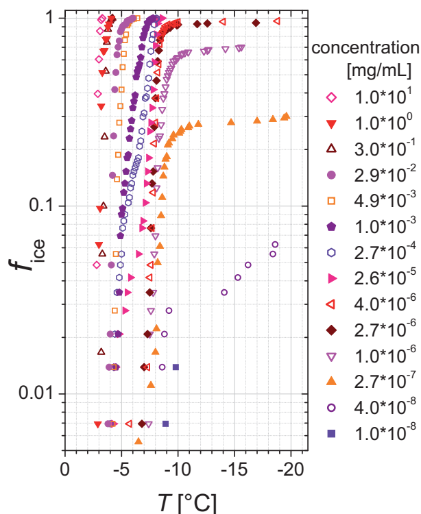
Figure 5. Frozen fractions as a function of temperature ( f_{ice} ) as measured by BINARY for 14 differently concentrated Snomax suspensions for droplets with diameters of 1240\ \mu\text{m} (i.e., 1\ \mu\text{L} ).
