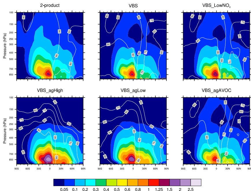
Figure 1. Annual mean zonally averaged SOA concentration ( \mu\text{g m}^{-3} ) (shown as colored shades) and the fraction of biogenic SOA (%) (shown as white contours) in CAM4-chem for different SOA treatments.
