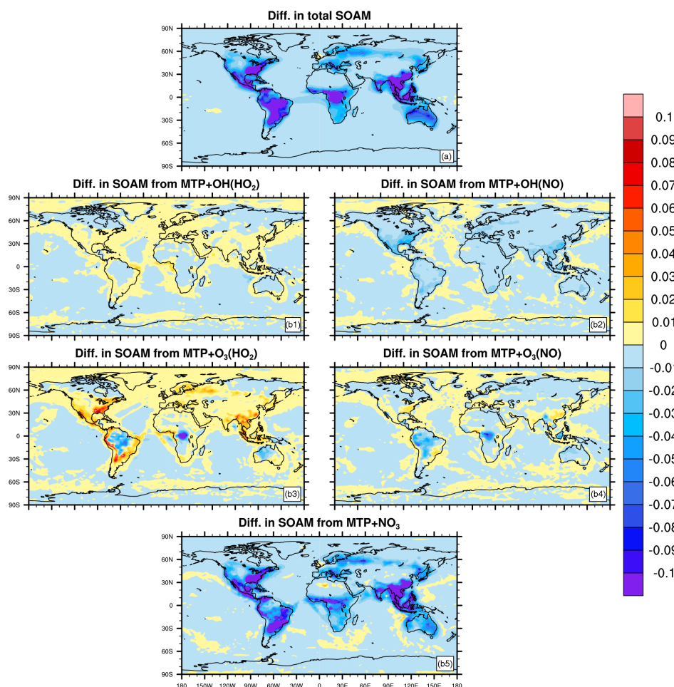
Figure 9. Changes in SOAM concentration ( \mu\text{g m}^{-3} ) in the sensitivity run with 50 % reductions in anthropogenic \text{NO}_x emissions compared to the control run using the VBS_agHigh scheme. The total SOAM change is shown in (a). The SOAM change in each formation branch is denoted as (b1) MTP+OH( \text{HO}_2 ) (low- \text{NO}_x OH-photooxidation), (b2) MTP+OH(NO) (high- \text{NO}_x OH-photooxidation), (b3) MTP+ \text{O}_3 ( \text{HO}_2 ) (low- \text{NO}_x ozonolysis), (b4) MTP+ \text{O}_3 (NO) (high- \text{NO}_x ozonolysis), and (b5) MTP+ \text{NO}_3 ( \text{NO}_3 -initiated oxidation).
