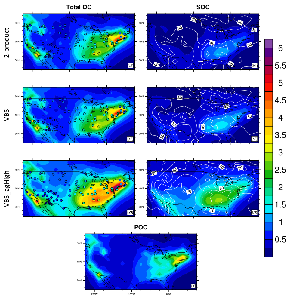
Figure 2. Annual mean surface concentrations (units: \mu\text{g}[\text{C}] \text{m}^{-3} ) of (a1)–(a3) total organic carbon (OC = POC + SOC), (b1)–(b3) secondary organic carbon (SOC) and (c) primary organic carbon (POC). The data is averaged from 2005 to 2009. In (a1)–(a3), scatters are IMPROVE observations and color shades are simulated total OC from the models 2-product, VBS and VBS_agHigh. In (b1)–(b3), white contours indicate the fraction of SOC in total OC (%), ranging from 30 to 70 % with an interval of 10 %. (c) shows simulated POC, which is identical in the three simulations.
