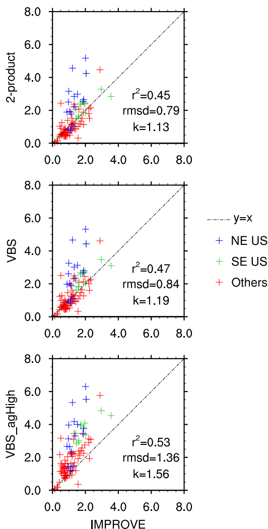
Figure 3. Comparison of averaged annual mean surface OC concentrations ( \mu\text{g}[\text{C}] \text{m}^{-3} ) between IMPROVE measurements and the three simulations: 2-product, VBS and VBS_agHigh. Different colors indicate sites in different regions. In each subplot, the dashed line is the 1 : 1 line. The coefficients of determination ( r^2 ), root-mean-square difference (rmsd) and the model-to-observation slope ( k ) are included.
