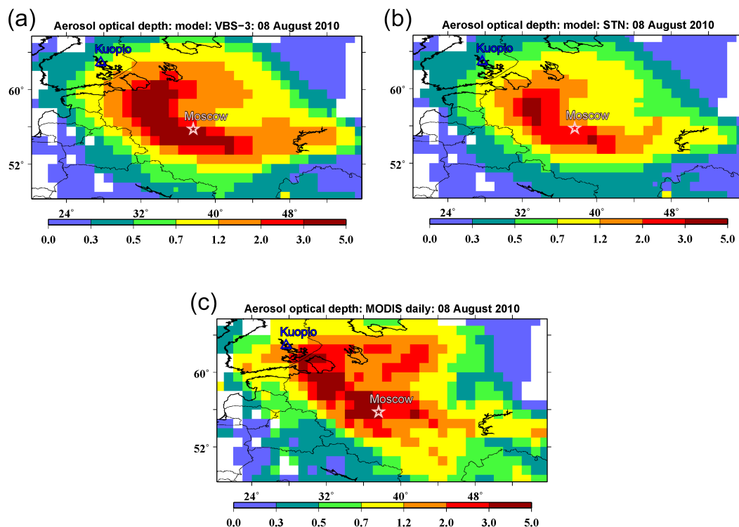
Figure 8. Spatial distributions of AOD at 550 nm on 8 August 2010 according to simulations for scenarios VBS-3 (a) and STN (b) in comparison with the MODIS measurement data (c).
