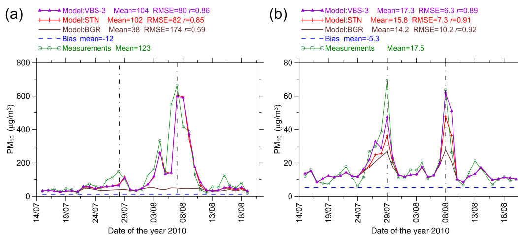
Figure 4. The same as in Fig. 3 but for PM 10 concentrations, except that in addition to results for the STN and BGR runs, this figure also shows (by a purple line) results for the VBS-3 run.
