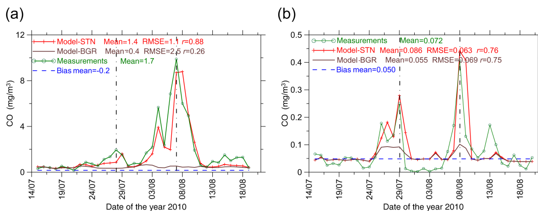
Figure 3. Time series of daily CO concentrations in Moscow (a) and in Kuopio (b). The CO concentrations for simulation scenario STN (see the red lines with crosses) are obtained by taking into account both anthropogenic and fire emissions (as explained in Sect. 2.8), while that for the BGR run (see the solid brown lines) reflects only anthropogenic CO emissions (along with other sources contributing to the boundary conditions for CO). The dashed blue lines depict the model bias (representing the systematic difference between the simulations and measurements on days not affected by fires); note that a negative bias (specifically, in plot a) is shown with the opposite sign. The measurement data (from Mosecomonitoring stations and the Maaherrankatu site in Kuopio) are shown by green lines. The vertical dashed lines indicate the CO concentrations observed (a) in Moscow on 28 July and 7 August and (b) in Kuopio on 29 July and 8 August.
