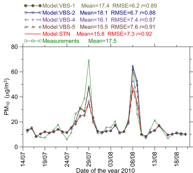
Figure 5. Time series of daily \text{PM}_{10} concentrations according to different simulation scenarios in comparison with measurements in Kuopio. Note that the time series for the VBS-3 scenario, which is shown in Fig. 4b, is omitted in this figure. Note also that the fire emissions for each scenario were fitted independently to measurements in the Moscow region (see the estimates of the emission correction factor, F_{\alpha} , in Table 4 and the respective remark in Sect. 2.8).
