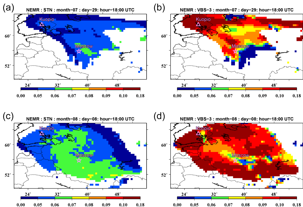
Figure 6. Normalized excess mixing ratio (NEMR) calculated as the ratio of near-surface mass concentrations of \text{PM}_{10} and \text{CO} ( \text{g g}^{-1} ) originating from the fires. The NEMR values are shown only in the grid cells with \text{CO} concentrations exceeding 100 \mu\text{g m}^{-3} for 29 July (a, b) and 8 August (c, d) 2010 according to the STN (a, c) and VBS-3 (b, d) scenarios.
