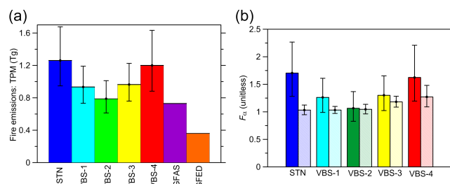
Figure 11. (a) Top-down estimates (in Tg) of total BB aerosol emissions from the study region in the period from 1 July to 31 August 2010 according to different simulation scenarios and in comparison with total particulate matter (TPM) emission data from the GFASv1.0 and GFED3.1 inventories. The estimates are derived from the MODIS AOD measurements. (b) The corresponding optimal estimates of F_\alpha derived from MODIS (boxes with solid filling) measurements in comparison with corresponding estimates (boxes with dashed filling) obtained from ground-based measurements in the Moscow region. Note that the estimates for the “unrealistic” scenario “VBS-5”, which would exceed the axis limits (see Sect. 3.4), are not shown.
