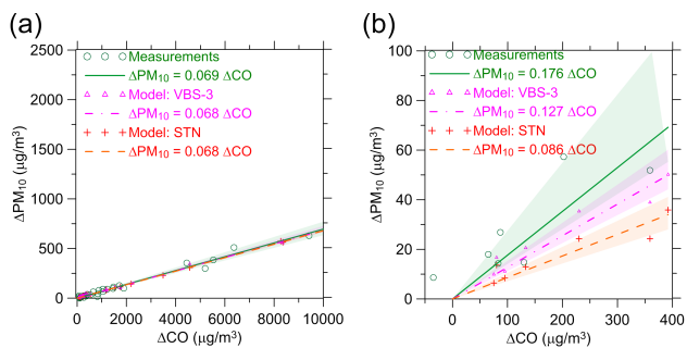
Figure 7. Scatterplots of the enhancements of \text{PM}_{10} and \text{CO} concentrations ( \Delta\text{PM}_{10} and \Delta\text{CO} ) in (a) Moscow and (b) Kuopio on days affected by smoke from fires. Note that the relative scales of the \Delta\text{PM}_{10} and \Delta\text{CO} values are the same in both plots. The slope of a linear fit (through the origin) to the data provides an estimate of NEMR (see Sect. 3.1). The shaded areas depict uncertainties of the fits at the 95 % confidence level.
