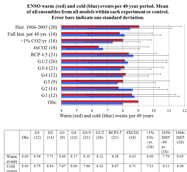
Figure 6. Number of ENSO warm (red) or cold (blue) events simulated or observed between 2030 and 2069 for G3, G4 and RCP4.5; years 11 and 50 for G1, G2, +1 % CO 2 yr -1 increase and 4XCO 2 ; and 1966 and 2005 for historical simulations and observations for the CanESM, CSIRO, GISS, HadGEM, IPSL and MPI models. The full historical record spans 1850–2005 and the number of events reported for this period is the per 40-year frequency of warm or cold events in this full record. Values in parentheses are the number of ensemble members for each experiment or family of experiments. Error bars represent ±1 standard deviation of ENSO events relative to the experiment mean. A table of values is provided under the graph.
