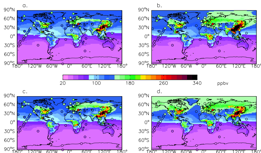
Figure 6. CO for March through May of 1999–2009 from the GMD observations (circles) overplotted on the surface CO from (a) RefGMI, (b) GMI-HiEmis, (c) RefCOonly, and (d) COonlyLowNHOH simulations.
