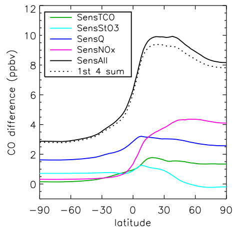
Figure 11. Zonal mean surface CO difference compared to RefCO–OH for the CO–OHSensTCO (green), CO–OHSensStO3 (cyan), CO–OHSensQ (blue), CO–OHSensNO _x (pink), and CO–OHSensAll (solid black) simulations averaged over March through August of 2005 to 2009. The sum of the differences for the CO–OHSensTCO, CO–OHSensStO3, CO–OHSensQ, and CO–OHSensNO _x compared to RefCO–OH is shown as the black dotted line.
