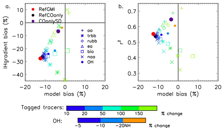
Figure 5. As in Fig. 4 but for June through August.
