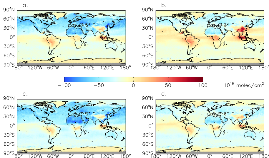
Figure 7. March through May difference between the simulated CO columns and MOPITT averaged over 2000–2009 for the (a) RefGMI, (b) GMI-HiEmis, (c) RefCOonly, and (d) COonlyLowNHOH simulations. The simulated CO is convolved with the MOPITT averaging kernels and a priori.
