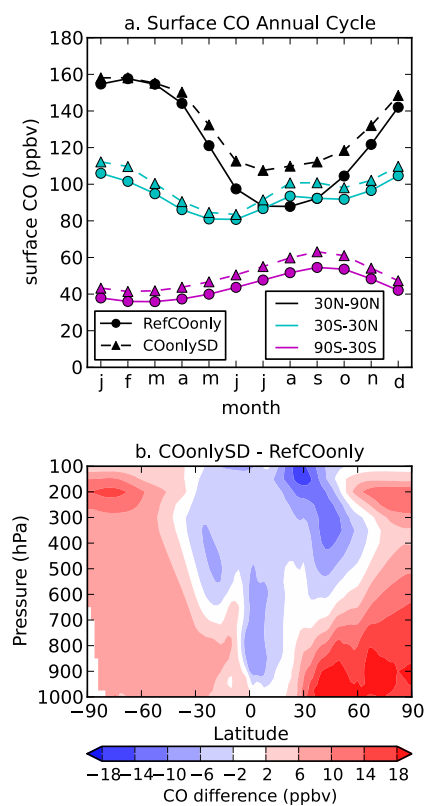
Figure 8. (a) Annual cycle of surface CO in the RefCOonly simulation (circles) and COonlySD simulation (triangles) for 30–90° N (black), 30° S–30° N (cyan), and 90–30° S (magenta). (b) Annual zonal mean cross section of the difference in CO between the COonlySD and RefCOonly simulations.
