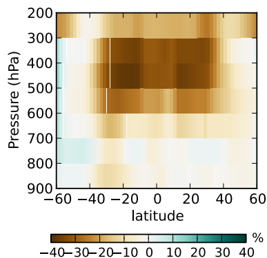
Figure 10. Annual mean percent change in specific humidity imposed in the CO–OHSensQ experiment between 900 and 200 hPa, 60° S–60° N.
