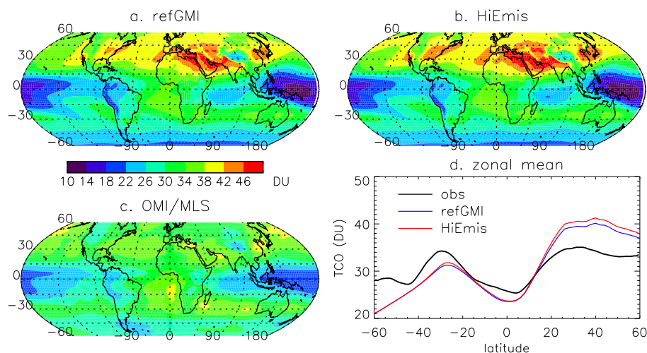
Figure 9. Annual mean tropospheric column ozone (TCO) from the RefGMI (a) and GMI-HiEmis (b) simulations compared to the OMI/MLS TCO product (c) of Ziemke et al. (2011). Panel (d) compares the zonal mean simulated and OMI/MLS values. The simulated values are averaged over the years of the time slice (1999–2009).
