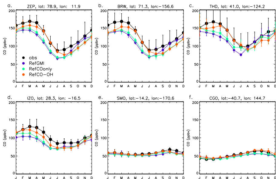
Figure 2. Monthly mean GMD observations (black) and results from the RefGMI (purple), RefCOonly (green), and RefCO–OH (orange) simulations. Circles and error bars represent the mean and min–max range, respectively, for 1999–2009. The GMD sites are as follows: (a) Ny-Alesund, Svalbard (ZEP, 78.9° N, 11.9° E); (b) Barrow, Alaska (BRW, 71.3° N, 156.6° W); (c) Trinidad Head, California (THD, 41.0° N, 124.2° W); (d) Izana, Tenerife, Canary Islands (IZO, 28.3° N, 16.5° W); Tutuila, American Samoa (SMO, 14.2° S, 170.6° W); and (e) Cape Grim, Tasmania (CGO, 40.7° S, 144.7° E).
