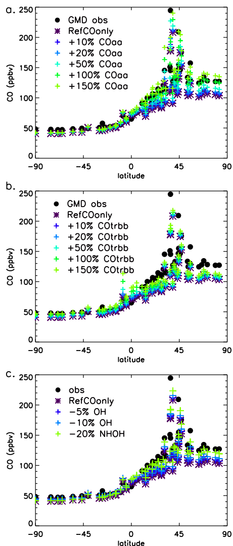
Figure 3. Latitudinal distribution of CO observations from the GMD network (black circles) and simulated CO from the RefCOonly simulation (purple stars) averaged over March–August. Blue–green + signs indicate the effect of (a) increasing the Asian anthropogenic CO tracer, (b) increasing the tropical biomass burning CO tracer, and (c) decreasing OH globally by 5 or 10 %, or decreasing NH OH by 20 %.
