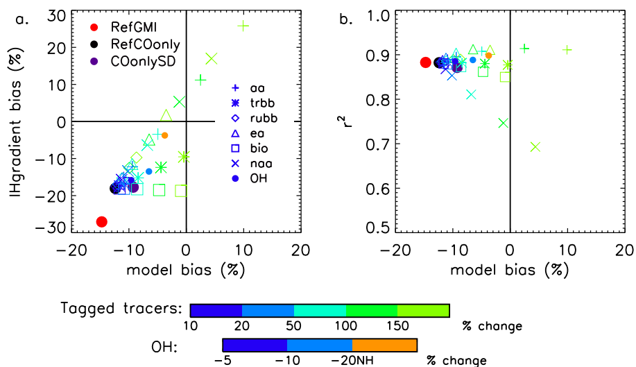
Figure 4. The impact of increasing the tagged-CO tracers for Asian anthropogenic (+), tropical biomass burning (stars), Russian biomass burning (diamonds), European anthropogenic (triangles), biogenic (squares), and North American anthropogenic (x) sources on (a) bias in the inter-hemispheric gradient versus global mean bias and (b) correlation versus global mean bias compared to GMD observations from March to May. Large circles represent the RefGMI (red), RefCOonly (black), and COonlySD (purple) simulations. Small circles show the impact of changing global or NH OH in the RefCOonly simulation.
