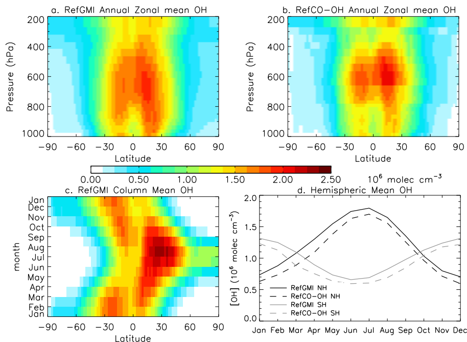
Figure 1. Simulated annual zonal mean OH concentration for the RefGMI (a) and RefCO–OH simulations (b) averaged over 1999–2009. (c) The annual cycle of the pressure-weighted column mean OH by latitude from the RefGMI simulation. The column is averaged between the surface and 200 hPa. (d) The annual cycle of hemispheric mean OH from the RefGMI (solid lines) and RefCO–OH (dashed lines) simulations for the Northern Hemisphere (black lines) and Southern Hemisphere (gray lines).
