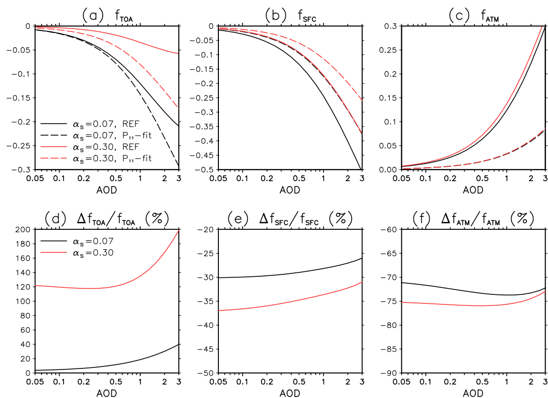
Figure 9. (a–c) Normalized aerosol radiative effects (Eqs. 12–14) for the REF (solid lines) and P_{11} -fit cases (dashed lines) for surface albedos of \alpha_s = 0.07 (black) and \alpha_s = 0.30 (red). (d–f) Corresponding relative differences (in %) between the P_{11} -fit and REF cases.
