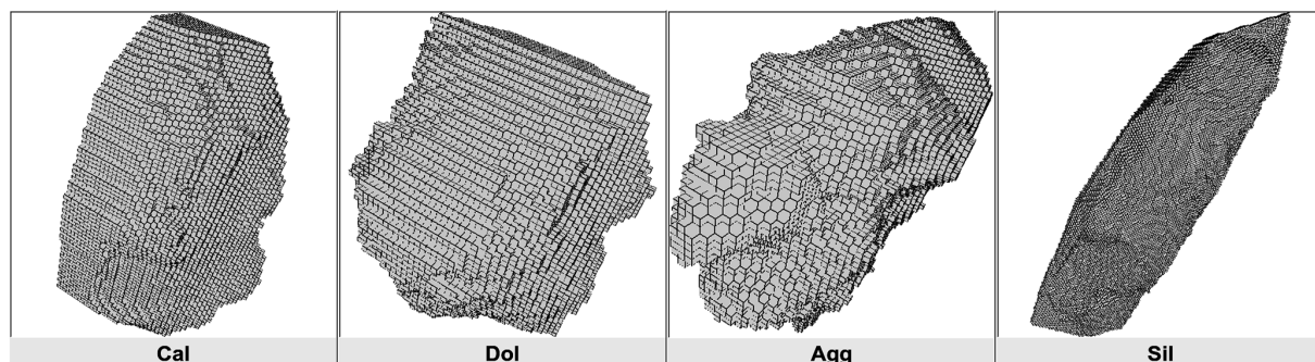
Figure 1. Renders of the DDA representations of the four target particles. The particles are depicted here with one-eighth of the dipole resolution compared to the calculations.
