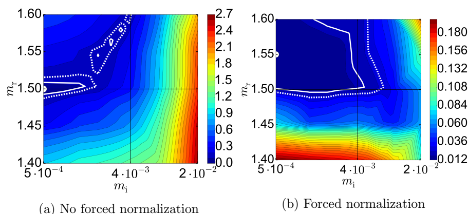
Figure 6. Illustration of two combined P_{11} and P_{12} normalization scenarios for the particle ensembles, as Fig. 3. (a) shows the sum the individual E_{ij} directly such as they are, while (b) the individual errors are first scaled in such a way that the error range of each element is the same, i.e. unity. The behavior of scattering error depends greatly on how the components of the multi-element errors are weighted.
