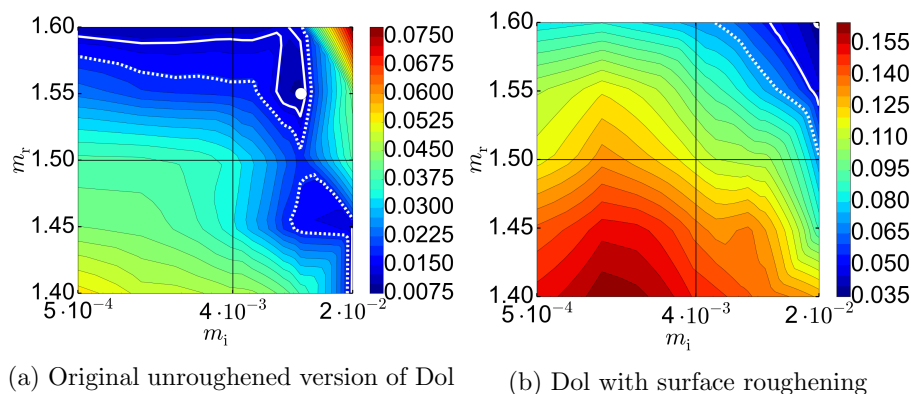
Figure 5. Illustration of the effect of roughening on P_{34} of Dol as in Fig. 3. The added modest surface roughness in (b) changes the behavior of the scattering error as function of the refractive index dramatically.
