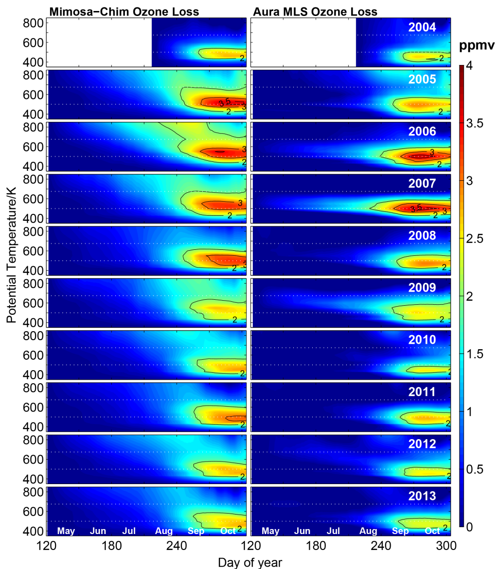
Figure 5. Vertical distribution of the vortex-averaged (defined by \geq 65^\circ EqL) ozone loss estimated for the Antarctic winters in 2004–2013. The model results are interpolated with respect to the time and location of the MLS measurements inside the vortex and then averaged for the corresponding day. Left: the ozone loss derived from the difference between the passive ozone and the chemically integrated ozone by MIMOSA–CHIM. Right: the ozone loss derived from the difference between the MIMOSA–CHIM passive ozone and the ozone measured by MLS. Both model results and MLS data are smoothed for 7 days. The y axis represents potential temperature in K. The white dotted lines represent 500 K ( \sim 19 km) and 675 K ( \sim 26 km).
