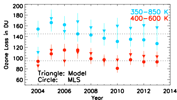
Figure 6. Vortex-averaged (defined by \geq 65^\circ EqL) column ozone loss computed from the MIMOSA–CHIM model simulations and MLS measurements, during the maximum ozone loss period in the Antarctic, at 350–850 K and 400–600 K for the 2004–2013 period. The estimated uncertainty of the column loss computed from both simulations and measurements is about 10% (e.g., Kuttippurath et al., 2011).
