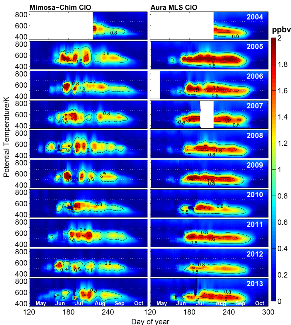
Figure 3. Vertical distribution of the vortex-averaged (defined by \geq 65^\circ EqL) ClO estimated from the MIMOSA-CHIM model and MLS measurements for the Antarctic winters 2004–2013. The model results are interpolated with respect to the time and location of the MLS measurements inside the vortex and then averaged for the corresponding day. ClO data are not available for early May 2006 and late July and early August 2007. The measurements are selected for 10:00–16:00 local solar time and solar zenith angles below 89^\circ . Both model results and MLS data are smoothed for 7 days. The y axis represents potential temperature in K. The white dotted lines represent 500 K ( \sim 19 km) and 675 K ( \sim 26 km).
