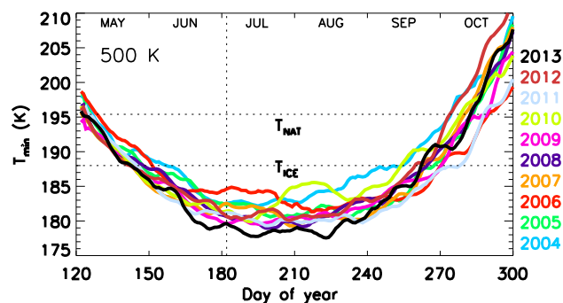
Figure 2. Evolution of polar cap (50–90° S) minimum temperature derived from the ECMWF operational analyses for each winter from 2004 to 2013 at 500 K (~19 km) potential temperature. The T_{\text{NAT}} and T_{\text{ICE}} thresholds are also marked.
