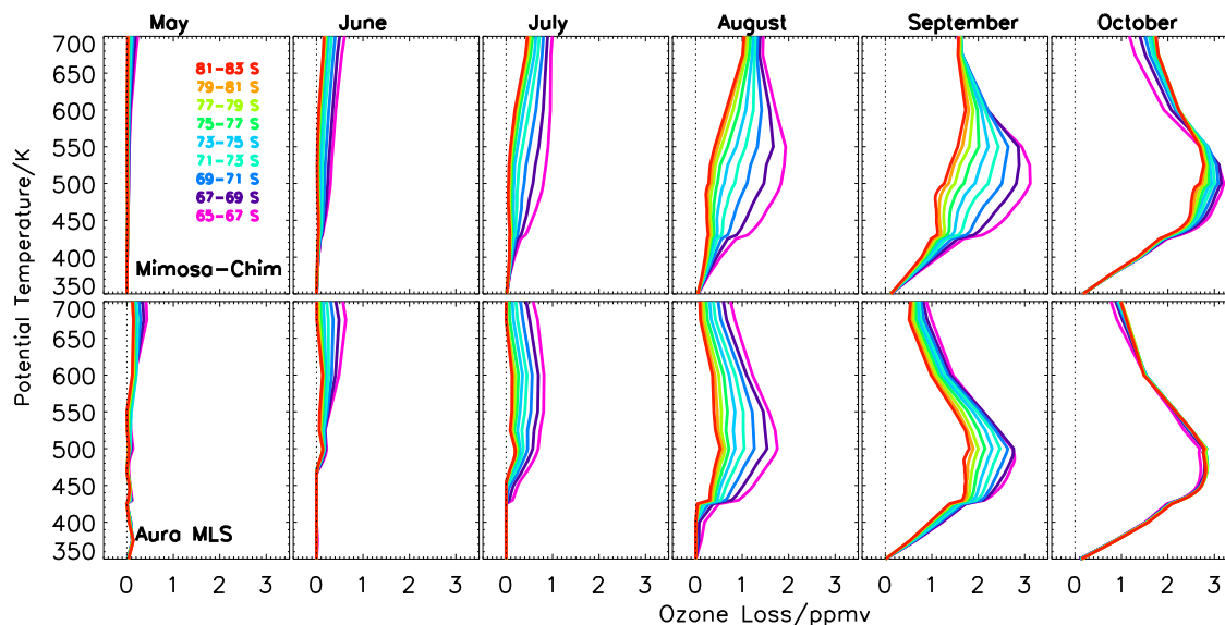
Figure 1. The 10-year (2004–2013) average monthly mean ozone loss estimated at different equivalent latitude (EqL) bins (of 2°) from 65 to 83° S EqL from the MIMOSA–CHIM simulations and MLS measurements. The model results are interpolated with respect to the time and location of the MLS measurements inside the vortex and then averaged for the corresponding day. The y axis represents potential temperature in K. The black dotted lines represent 0 ppmv.
