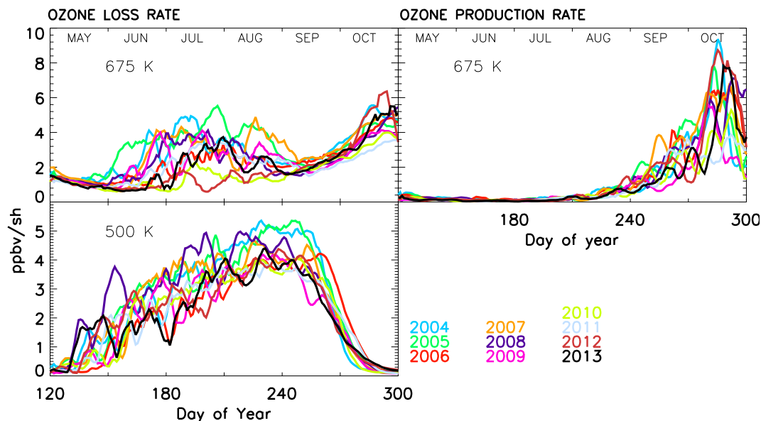
Figure 7. Vortex-averaged (defined by \geq 65^\circ EqL) chemical ozone loss and production rates at 675 K ( \sim 26 km) and 500 K ( \sim 19 km) in ppbv per sunlit hour ( \text{ppbv sh}^{-1} ) for the Antarctic winters 2004–2013 estimated from the MIMOSA–CHIM model simulations.
