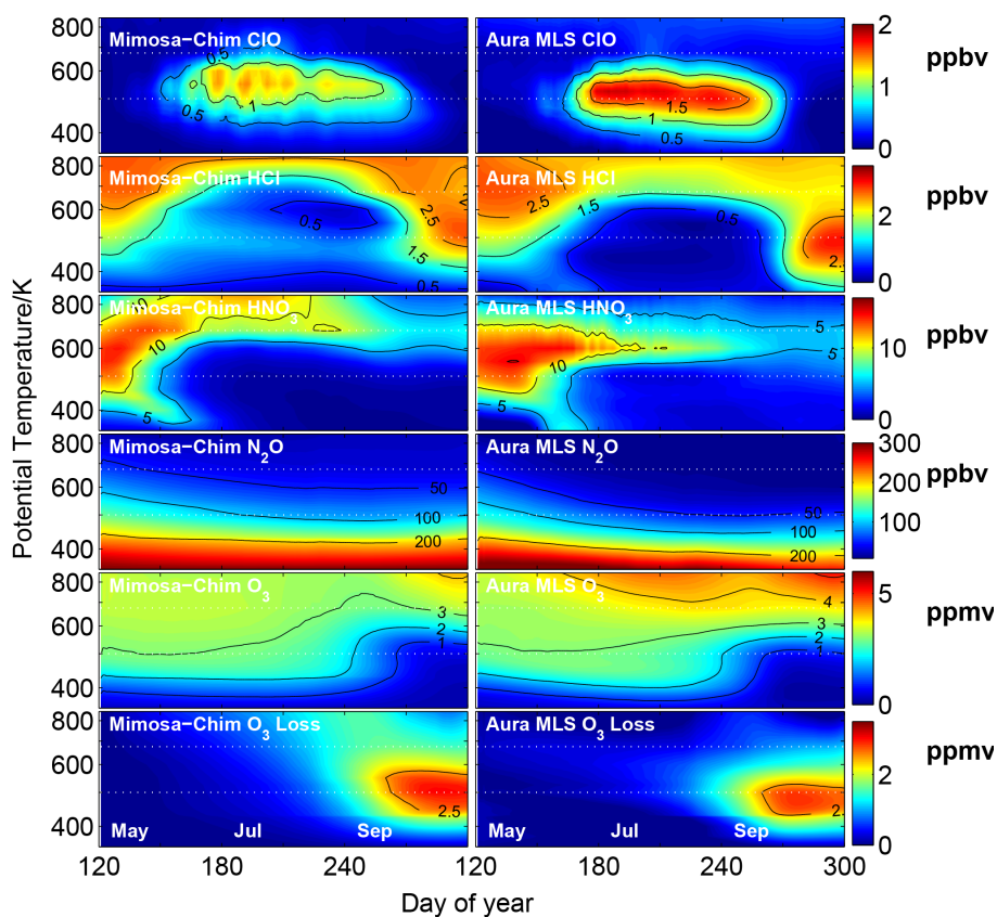
Figure 4. The vortex-averaged (defined by \geq 65^\circ EqL) vertical and temporal evolution of ClO, HCl, HNO 3 , N 2 O, O 3 and ozone loss from the MIMOSA–CHIM model and MLS measurements. The model results are interpolated with respect to the time and location of the MLS observations inside the vortex and then averaged for the corresponding time period. The data are the average of 10 Antarctic winters (2004–2013) and are smoothed for 7 days. ClO data are not available for early May 2006 and late July and early August 2007. The ClO measurements are selected for 10:00–16:00 for local solar time and solar zenith angles below 89^\circ . The y axis represents potential temperature in K and is on a logarithmic scale. The white dotted lines represent 500 K ( \sim 19 km) and 675 K ( \sim 26 km).
