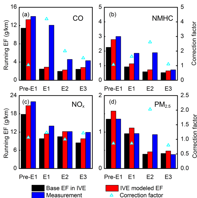
Figure 2. Comparison between measured emission factors for HDTs in China, IVE modeled emission factors and base emission factors in IVE model; and correction factors of HDTs for (a) CO, (b) NMHC, (c) NO x and (d) PM 2.5 .
