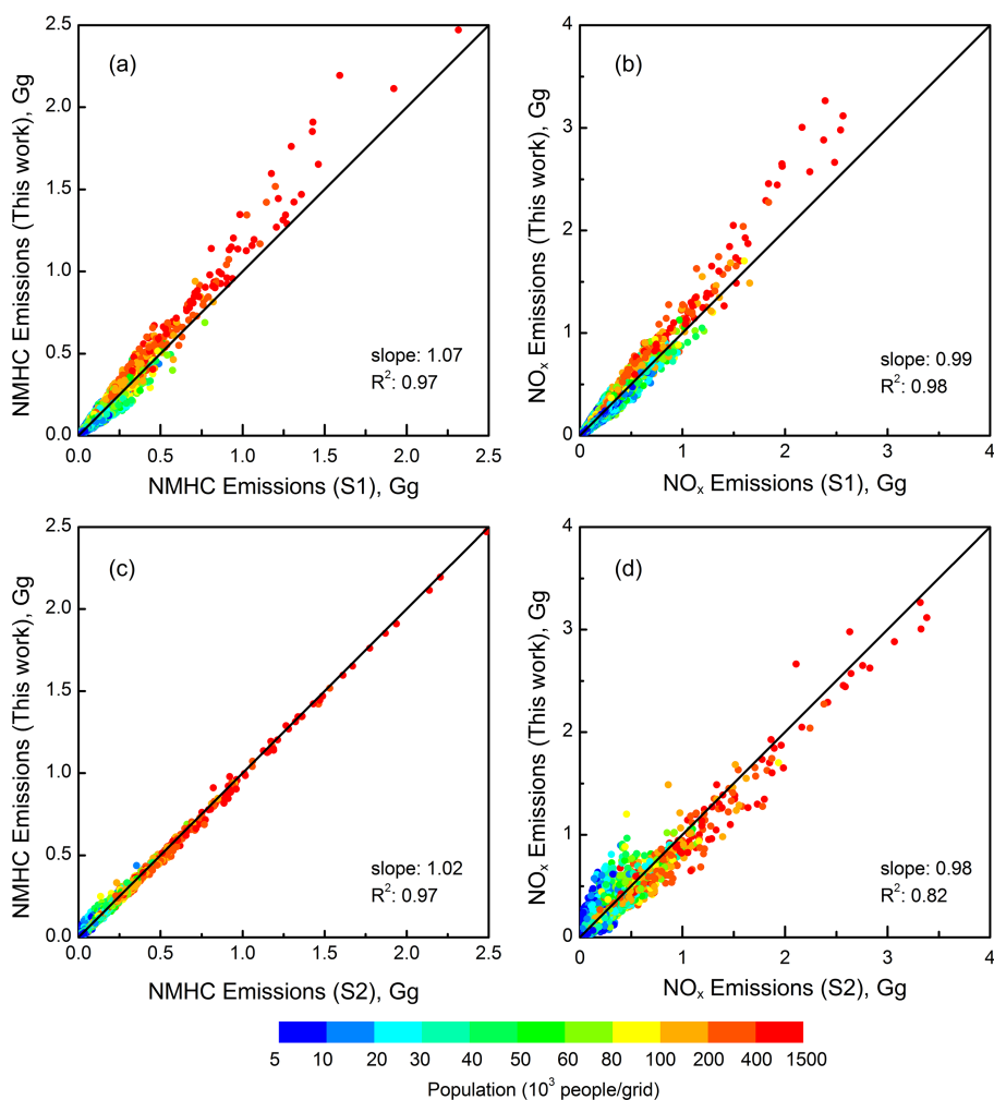
Figure 16. Comparison of gridded emissions at a resolution of 0.05^\circ \times 0.05^\circ between this work and the two sensitivity cases (S1 and S2): (a) gridded NMHC emissions of this work versus S1; (b) gridded \text{NO}_x emissions of this work versus S1; (c) gridded NMHC emissions of this work versus S2 and (d) gridded \text{NO}_x emissions of this work versus S2.
