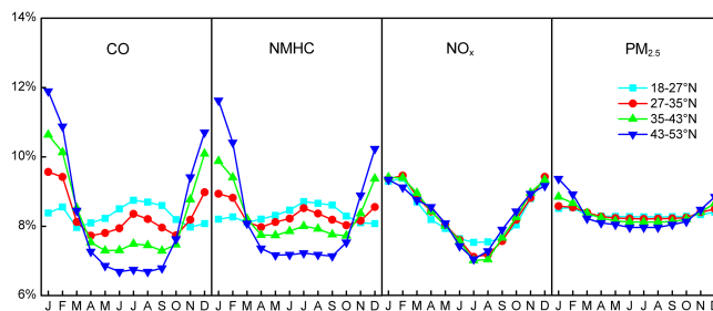
Figure 11. Share of monthly emissions of the whole year at different latitudes. Counties here are located in regions with the altitudes lower than 1000 m and the longitudes larger than 103° E.
