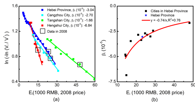
Figure 1. Gompertz regression of the Hebei Province and its cities: (a) Gompertz function fitting of Hebei versus three selected cities within it (Cangzhou, Tangshan and Hengshui); (b) The relationship between \beta values and per-cap GDP in 2008 of the Hebei province and all its cities.
