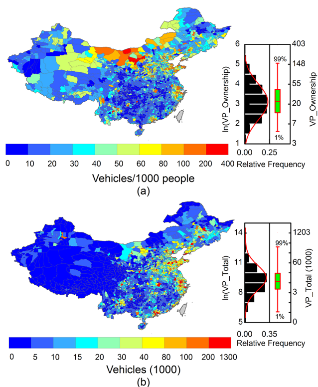
Figure 3. County-level vehicle population and vehicle ownership in 2008: (a) vehicle ownership (vehicles/1000 people) and (b) vehicle population (1000 units).
