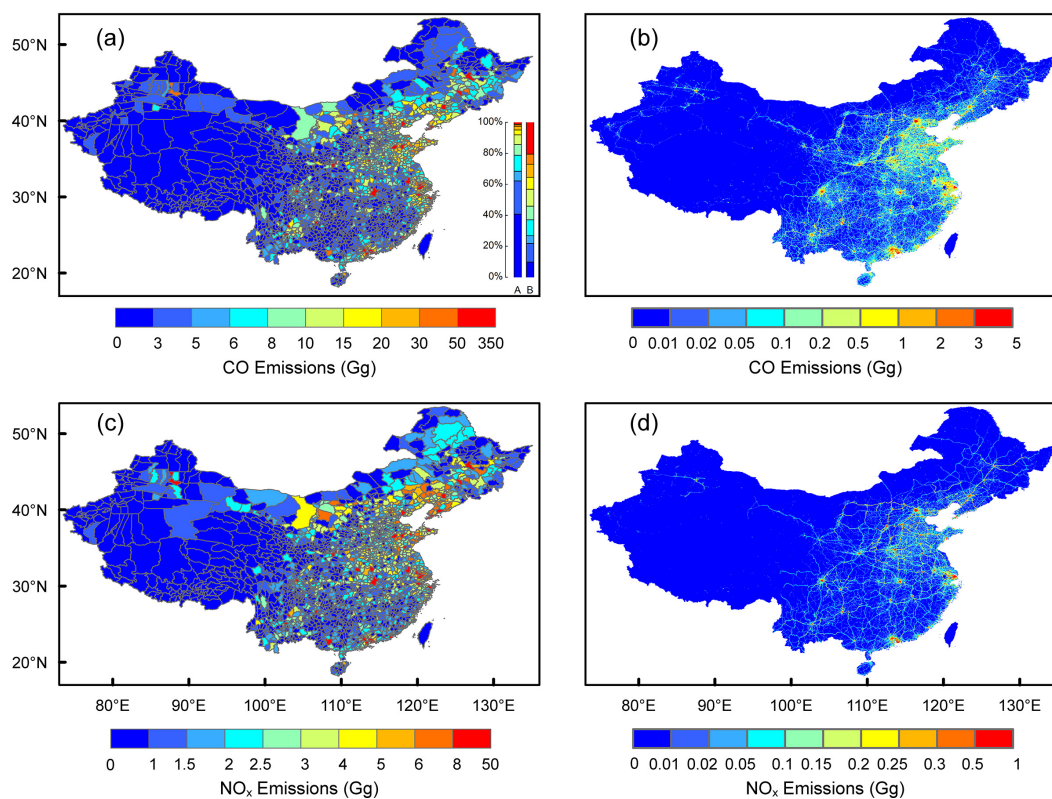
Figure 12. County and gridded emissions in 2008: (a) CO emissions by county (bar A represents the share of county numbers; bar B represents the share of county emissions); (b) gridded CO emissions at 0.05^\circ \times 0.05^\circ resolution; (c) NO x emissions by county and (d) gridded NO x emissions at 0.05^\circ \times 0.05^\circ resolution.
