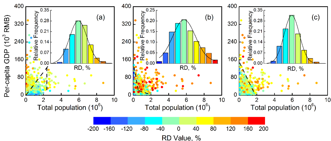
Figure 13. Distribution of the relative difference (RD) in gridded NMHC emissions at a resolution of 0.05^\circ \times 0.05^\circ between this work and other methods, and their relationships with county population and per-capita GDP: (a) this work versus M1; (b) this work versus M2 and (c) this work versus M3. RD is defined as RD_i = (E1_i - E2_i) / ((E1_i + E2_i) / 2) , where i represents county, E1 and E2 represent emissions by county generated from this study and other allocation methods (M1, M2, or M3). A positive (or negative) RD means that our method generates higher (or lower) emissions for this county than the other method.
