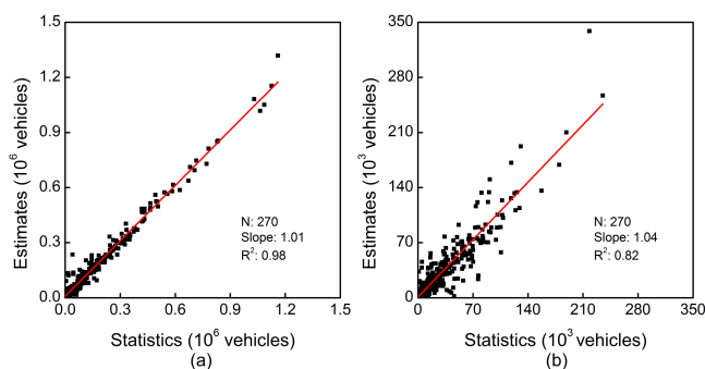
Figure 7. Comparison of the new vehicles simulated in this work and newly registered vehicles reported in statistics: (a) passenger vehicles and (b) trucks.
