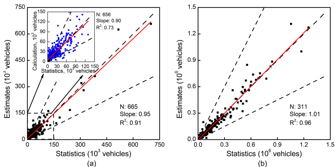
Figure 4. Comparison of the simulated and statistical vehicle population for (a) 665 counties and (b) 311 cities.
