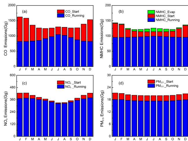
Figure 10. Monthly variations of vehicle emissions in 2008: (a) CO; (b) NMHC; (c) NO x and (d) PM 2.5 .
