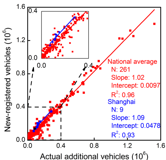
Figure 6. Correlation between newly registered vehicles and vehicle population growth from 2002 to 2010.
