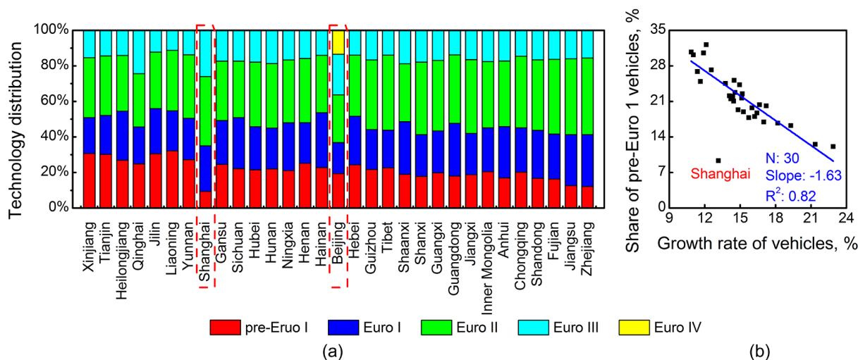
Figure 5. Relationship between vehicle technology distribution and vehicle growth rates: (a) technology distribution for each province in 2008 (provinces are ranked in order of annual vehicle growth rate from low to high, Beijing and Shanghai are highlighted because they implemented vehicle emission standards ahead of the country); (b) shares of pre-Euro 1 vehicles versus vehicle growth rates of 31 provinces. The growth rate is defined as the average growth rate between 2002 and 2010.
