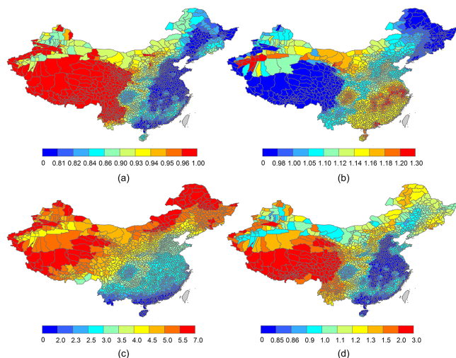
Figure 9. Spatial distribution of the meteorological correction factors for CO emissions of gasoline LDBs by county: (a) running emissions in January; (b) running emissions in July; (c) start emissions in January and (d) start emissions in July.
