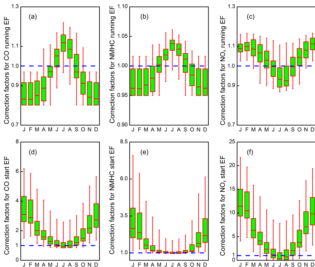
Figure 8. Meteorological correction factors of vehicle emissions by month: (a) running CO of gasoline LDBs; (b) running NMHC of gasoline LDBs; (c) running \text{NO}_x of diesel HDTs; (d) start CO of gasoline LDBs; (e) start NMHC of gasoline LDBs; (f) start \text{NO}_x of diesel HDTs. Each box plot displays the statistics of 2364 counties in China. The upper line of each box represents the 75 %, the middle line the 50 %, and the lower line the 25 % quartiles.
