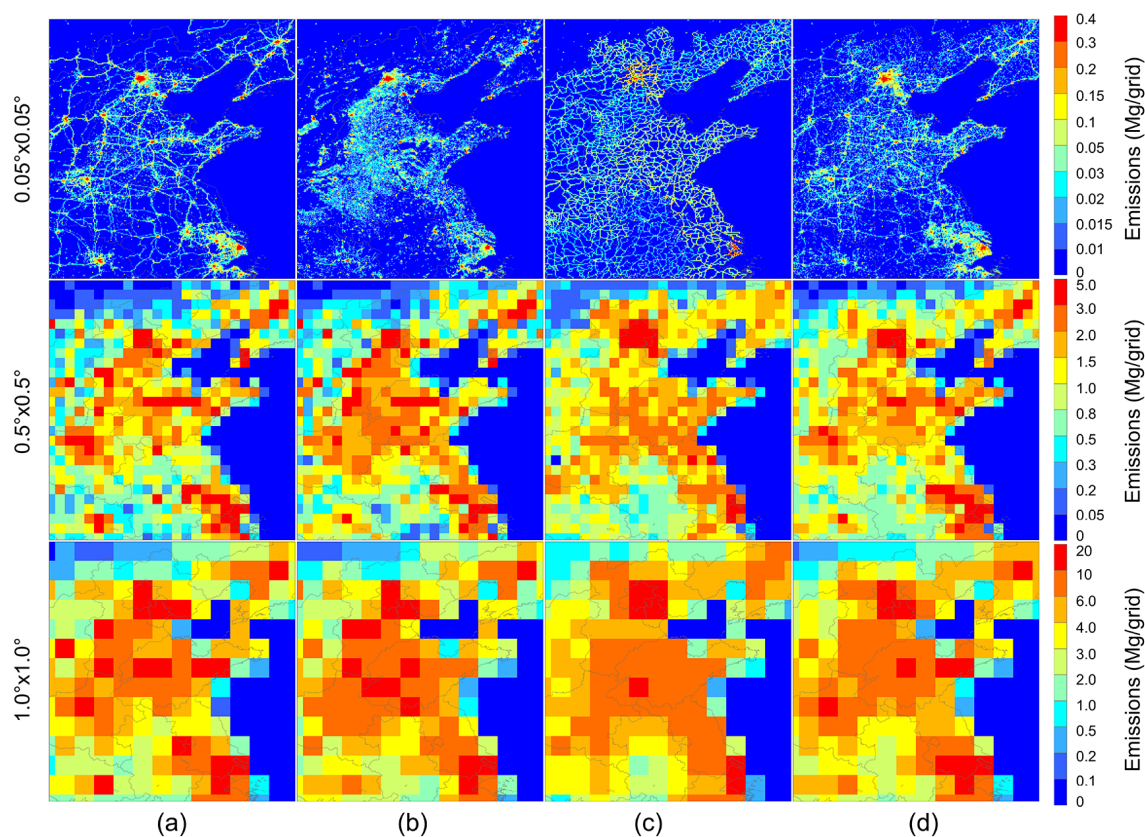
Figure 14. Vehicle NMHC emissions from different spatial allocation methods: (a) this work; (b) population-based method (M1); (c) DCW-based method (M2) and (d) CDRM-based method (M3).
