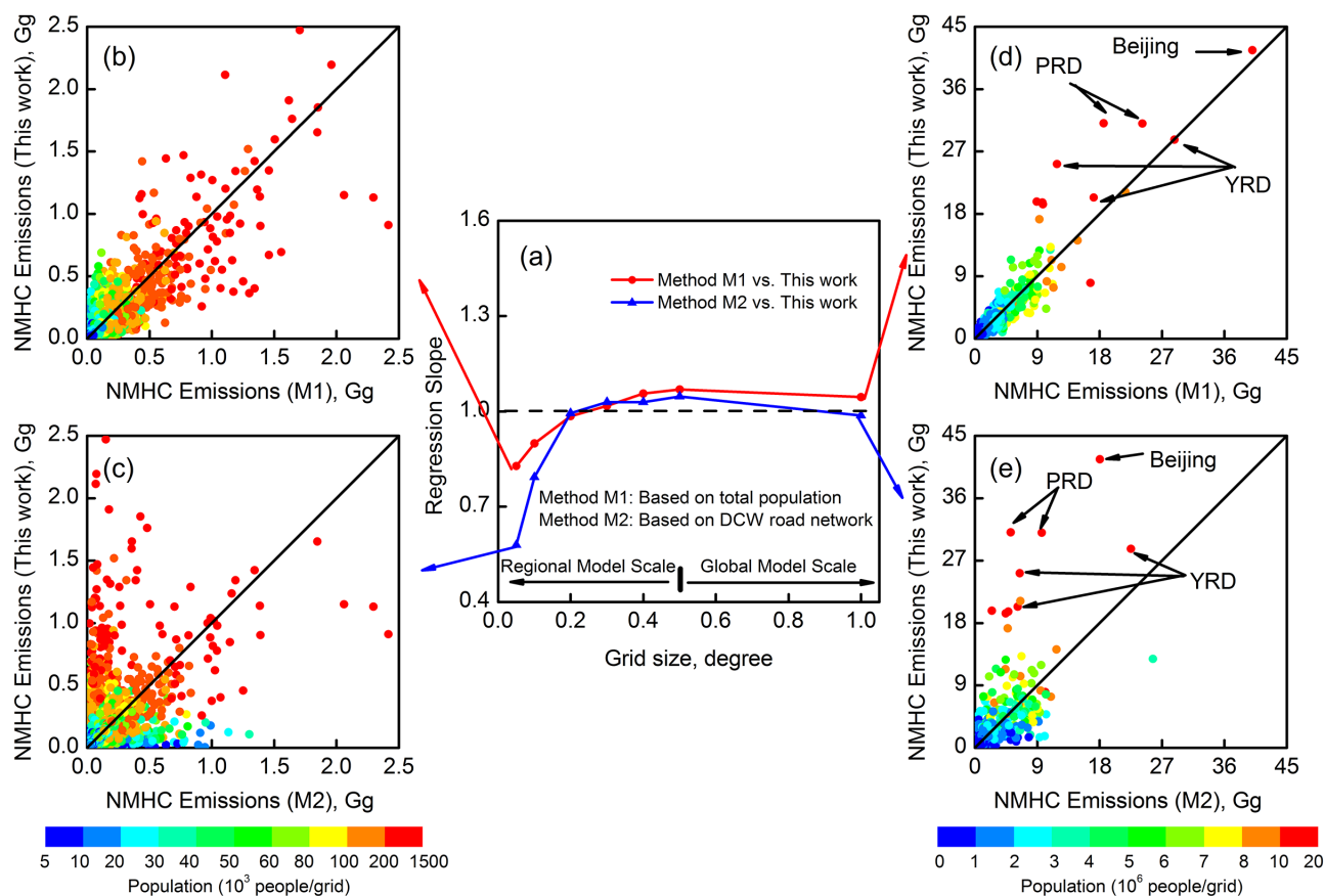
Figure 15. Comparison of the gridded emissions with different allocation methods: (a) average differences of gridded emissions between M1, M2 and this work at various resolutions; (b) this work versus M1 at a resolution of 0.05^\circ \times 0.05^\circ ; (c) this work versus M2 at a resolution of 0.05^\circ \times 0.05^\circ ; (d) this work versus M1 at a resolution of 1.0^\circ \times 1.0^\circ and (e) this work versus M2 at a resolution of 1.0^\circ \times 1.0^\circ .
