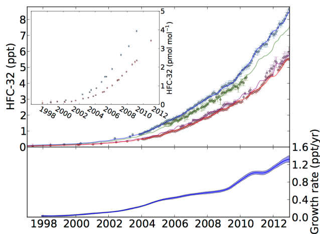
Figure 4. Semi-hemispheric monthly average HFC-32 mole fractions (30–90° N: blue; 0–30° N: green; 30–0° S: purple; 90–30° S: red). Averaged observations are shown as data points with error bars. The more sparse circles represent NH and SH air archive samples, and are highlighted in the inset box. The solid trend lines were calculated using a 12-box model with emissions from the inversion as input. The lower plot shows the annual running mean global mole fraction growth rate.
