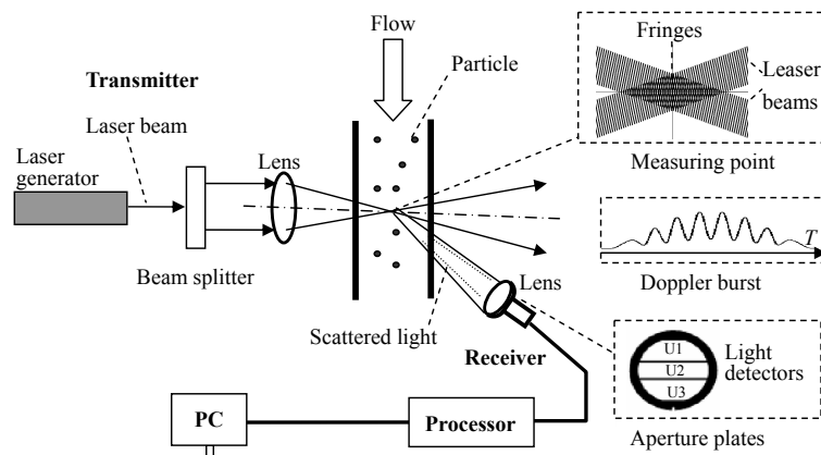
Figure 2. Basic structure of PDA. The velocities and sizes of particles passing through the measuring point are obtained by analyzing the light scattered by the particles.
