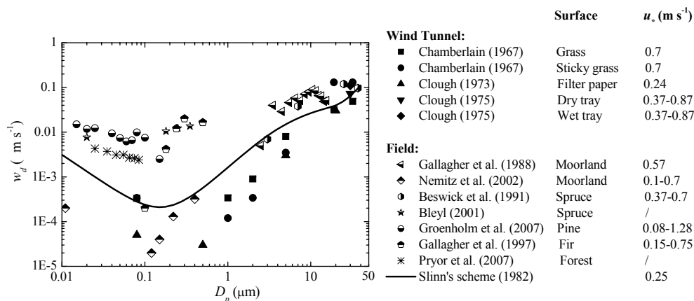
Figure 1. Some existing measurements of deposition velocities against particle size for different surfaces.
