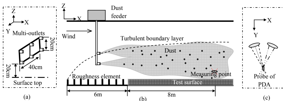
Figure 4. Configuration of the wind-tunnel experiment. (a) Dust feeding outlets; (b) Working section; the roughness elements fixed at the front of the working section generate a deep (at least 0.4 m) turbulent boundary layer. Downstream of the roughness-element section is the test surface. A dust feeder is placed at the beginning of the working section and injects dust ( \text{SiO}_2 ) into the tunnel through a tubular manifold. The measuring point is located near the end of the working section; (c) Probe of the PDA with laser beams intersecting at the measuring point.
