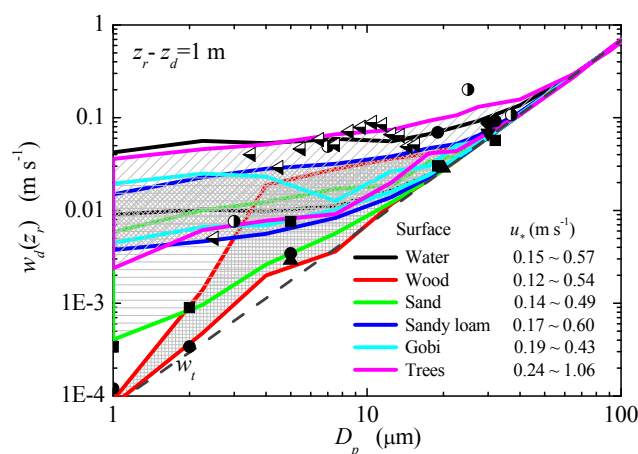
Figure 13. Comparison between the results of our measurements and other experiments. The lines and the shaded areas represent the range of dust deposition velocity over different surfaces, extracted from our data set. The dots are the results of the existing studies corresponding to Fig. 1 (with the same shape), but are recalculated to z_r = (z_d + 1) m.
