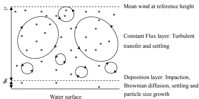
Figure A1. A schematic illustration of the two-layer model for dust deposition to a smooth surface.
