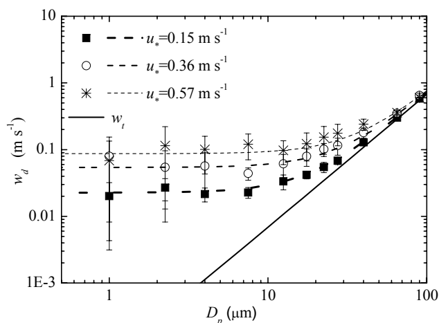
Figure 11. As Fig. 10, but for the water surface. The curves are the results predicted with the SS80 scheme by setting the laminar layer resistance 1/w_D to zero. The height of the measuring point is 25 mm above the water surface.
