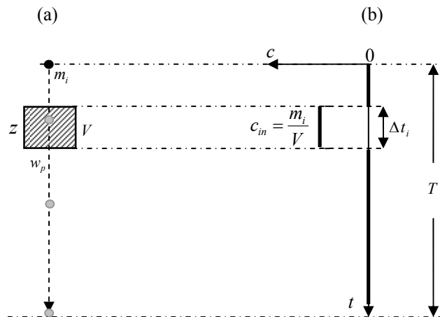
Figure 6. Illustration of one particle's contribution to dust concentration. (a) A dust particle (dot) passes through the sampling area (shaded); (b) Dust concentration corresponding to the situation shown in (a).
