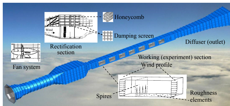
Figure 3. A sketch of the Lanzhou University wind tunnel.
