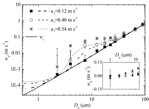
Figure 10. Deposition velocity against particle size under different wind conditions over the wood surface. The dots are averaged w_d and the error bars represent the variability of the three runs. The curves are the results predicted with the SS80 scheme. The height of the measuring point is 15 mm above the wood surface. w_d for small particles (1–12.5 \mu\text{m} ) have been inserted in the lower right corner to display the possible negative deposition velocities which impossibly appear in logarithmic coordinate system.
