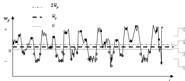
Figure 7. Illustration of the PDA data of particle velocity. Solid and open dots represent positive and negative w_p measured by PDA, respectively, and the solid line w_a + w_t . As an example, suppose \bar{w}_p > 0 , the full data set is divided into four parts: (1) 0 < w_p < \bar{w}_p ; (2) \bar{w}_p < w_p < 2\bar{w}_p ; (3) w_p > 2\bar{w}_p ; and (4) \bar{w}_p < 0 .
