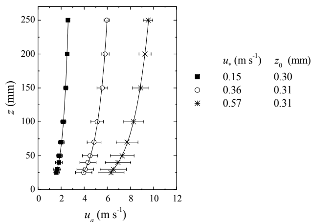
Figure 9. Wind profiles measured over the water surface for three experiments with the fan speed set to 3000, 9000 and 12 000 rpm. The dots are the mean wind speeds, and the error bars show the standard deviations. The curves are the logarithmic profiles fitted to the data.
