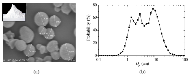
Figure 5. SiO 2 powder used as dust for the wind-tunnel experiment. (a) Powder appearance (top left corner) and microscopic picture (measured by Scanning Electron Microscope, SU1500); (b) Probability distribution of particle size (measured by Particle Size Analyzer, S3500).
