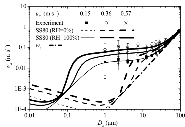
Figure A2. Results of our measurements and the SS80 scheme.
