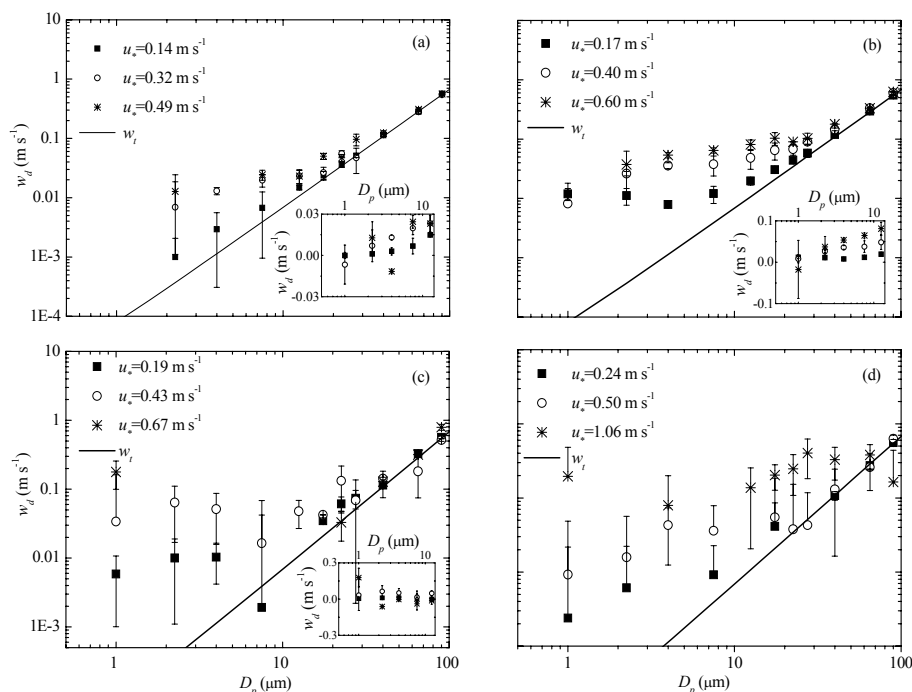
Figure 12. As Fig. 10, but for (a) sand, (b) sandy loam, (c) gobi, and (d) tree surface. For the tree surface, the measurement height is z_m = 250 mm.
