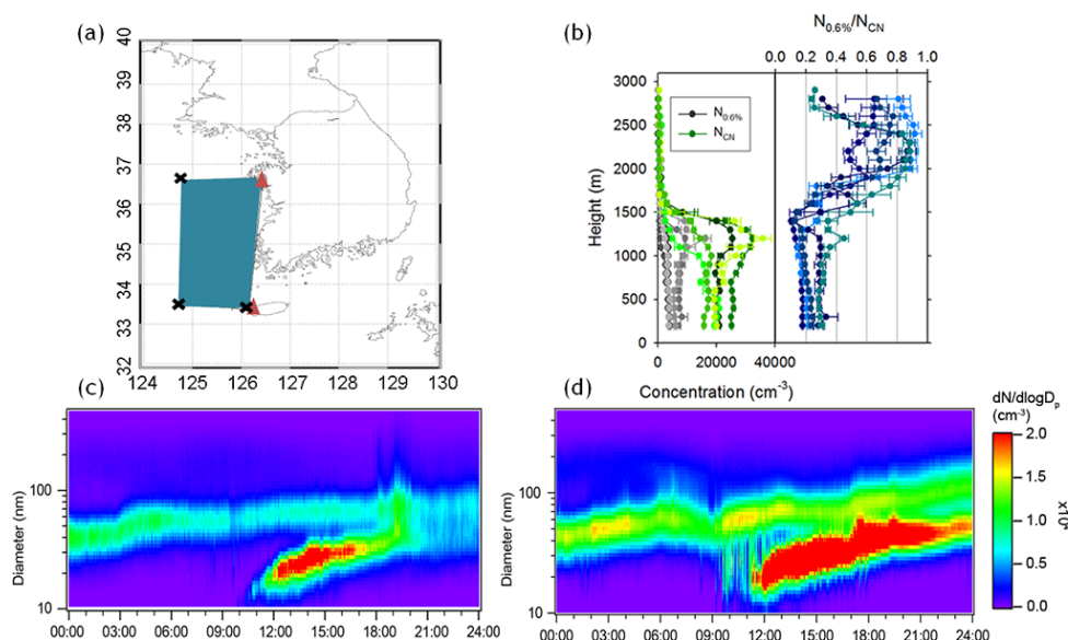
Figure 15. (a) Locations (X) where low N_{0.6\%}/N_{\text{CN}} was found in the lowest altitude during a flight between 12:14 and 15:30 on 18 October 2009 and the locations (triangle) of the surface SMPS measurements at KGAWC and Gosan; (b) vertical distributions of N_{\text{CN}} (green variant), N_{0.6\%} (grey variant) and N_{0.6\%}/N_{\text{CN}} (blue variant) during this flight; and the time variation of aerosol size distributions measured at (c) KGAWC and (d) Gosan on 18 October 2009.
