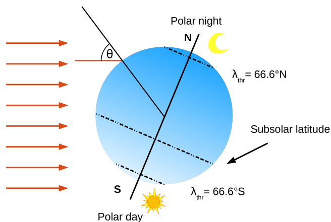
Figure 5. Geometry of incident solar radiation and Earth rotation at the December solstice. The threshold latitudes \lambda_{\text{thr}} separates the polar day and polar night regions from regions of alternating day and night periods. \Theta is to the solar zenith angle.
