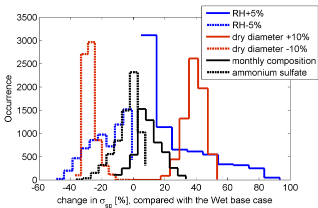
Figure 10. Sensitivity of the hourly calculated \sigma_{sp} to RH, aerosol dry size and chemical composition as compared with the Wet base case (see Table 2).
