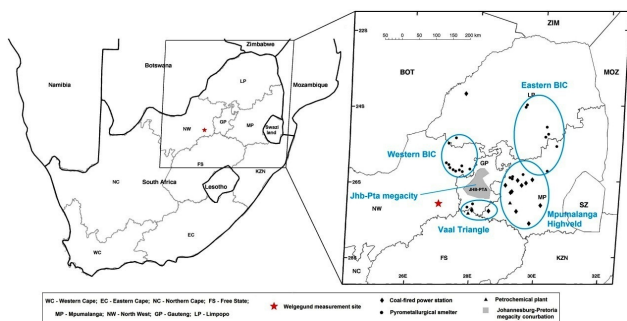
Figure 1. Map of southern Africa indicating the location of the Welgegund measurement station, large point sources in the industrial hub of South Africa and anthropogenic source regions impacting Welgegund.
