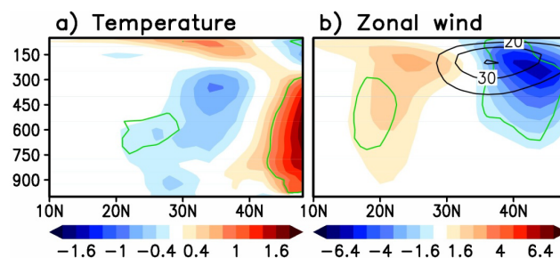
Figure 11. Zonal mean temperature (K) and wind (m s -1 ) differences between HighBoth and Zero Both BBA for 110–140° E in May. Green contour identifies regions with >95 % significant differences according to the Student’s t test. Black contour on (b) is zonal mean wind in HighBoth run.
