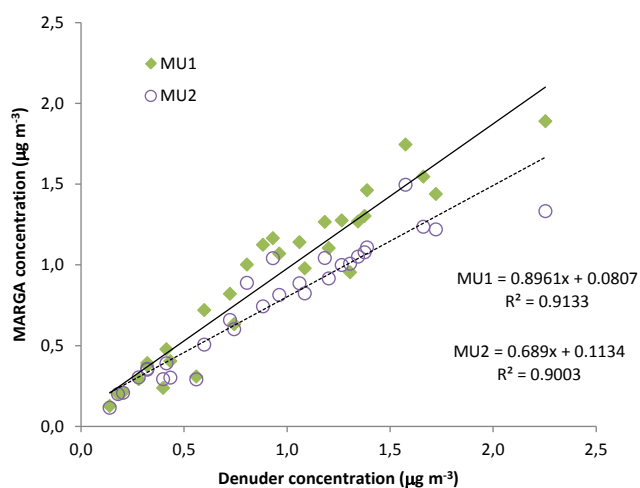
Figure 14. Regression analysis of 24 h average MARGA \text{HNO}_3 concentrations against denuder \text{HNO}_3 concentrations.
