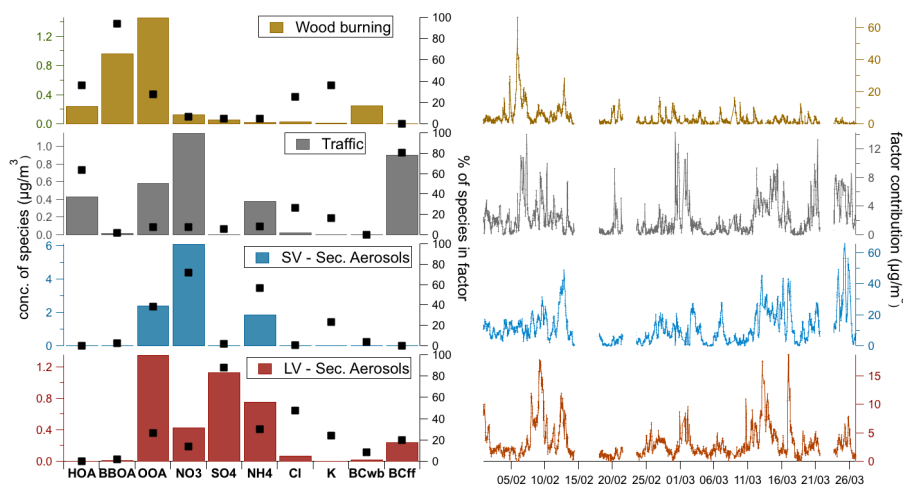
Figure 6. Factor profiles and time series for the four-factor solution of the global PM 1 source apportionment analysis. Note the different scales.
