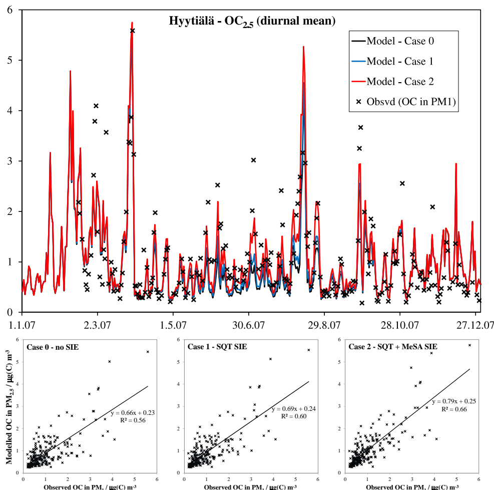
Figure 2. Modelled diurnal mean organic carbon in \text{PM}_{2.5} ( \text{OC}_{2.5} ) at Hyytiälä (Finland) for 2007 compared to measured OC in \text{PM}_1 (Aurela et al., 2011). Results from three different model simulations (see Sect. 2.5) are shown in the top panel: Case 0 (black line) – reference scenario, without explicit stress-induced emissions (SIE); Case 1 (blue) – current situation scenario with SIE of sesquiterpenes (SQT); Case 2 (red) – current situation scenario with SIE of SQT and methyl salicylate. The lower panels show the model–measurement scatter plots for the three cases. Unit: \mu\text{g}(\text{C})\text{m}^{-3} .
