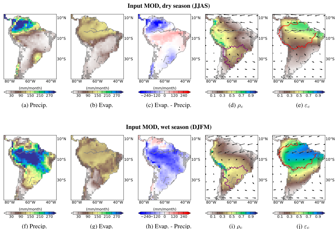
Figure 1. WAM-2layers input and output as calculated for the period 2001–2010 for MODIS and TRMM (input MOD; see Table 1): long-term seasonal mean of precipitation ( a, f ), evapotranspiration ( b, g ), precipitation–evapotranspiration ( c, h ), continental precipitation recycling ratio \rho_c ( d, i ) and continental evapotranspiration recycling ratio \varepsilon_c ( e, j ) indicating respective sinks and sources of continental moisture. Here and in the following figures, the vectors indicate the horizontal moisture flux field (in \text{m}^3 of moisture \times \text{m}^{-2} \times \text{month}^{-1} ) and the hatches represent grid cells where mean annual evapotranspiration exceeds mean annual precipitation. The red lines delimit the Amazon basin and the purple lines delimit the La Plata basin. Results are given for the dry season (upper row) and the wet season (lower row).
