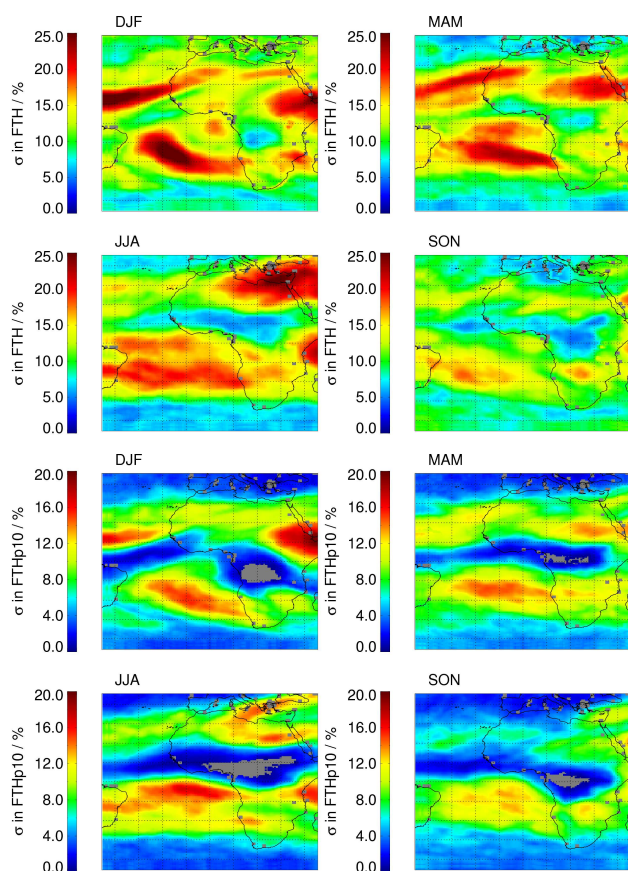
Figure 8. Relative standard deviation in FTH for each season (top four panels) and in FTHp10 (bottom four panels) over the period 1984–2009. Areas where only a small number of observations are valid are shown in grey.
