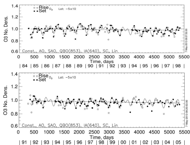
Fig. 12. Time series of SAGE II v7 ozone at 5^{\circ} S and 47.5 km for (top) 1984–1998 and (bottom) for 1991–2005.
