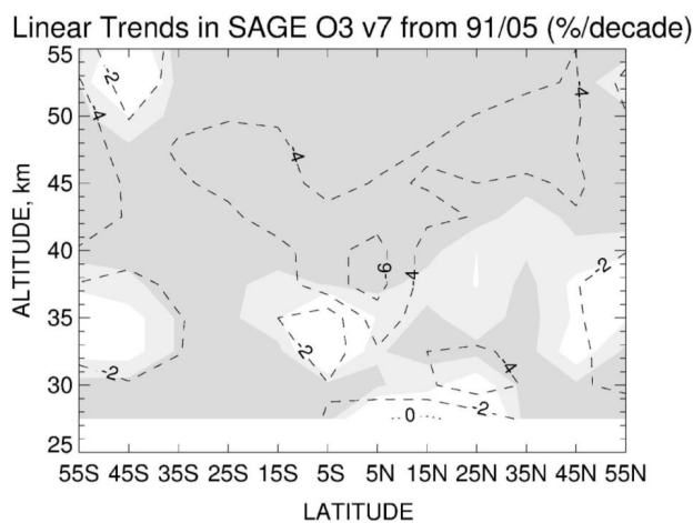
Fig. 4. Contour plot of the linear trend terms ( \% \text{ decade}^{-1} ) from the MLR models for the SAGE II ozone data of 1991–2005. Contour interval is 2\% \text{ decade}^{-1} . Dashed contours denote negative trends, and the dotted contour is where the trends are zero. Darker shading denotes where \text{CI} > 90\% for the trends; lighter shading has 70\% < \text{CI} < 90\% .
