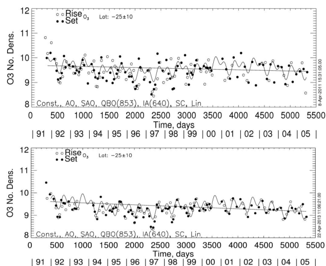
Fig. 1. Time series of bin-averaged SAGE II SR and SS ozone number density measurements (in \text{cm}^{-3} multiplied by 10^{-11} ) at 25^{\circ} S and 37.5 km (top) v6.2, (bottom) v7. Terms of the MLR model are indicated at the lower left, where SC refers to an 11 yr sinusoid term. The oscillating solid curve is the model fit to the data, while the straight line curve is the sum of just the constant and linear trend terms.
