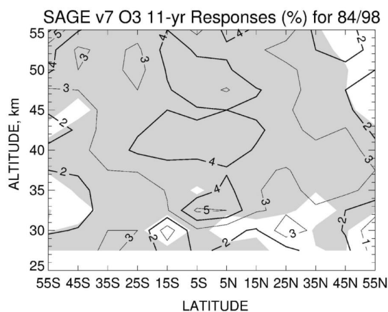
Fig. 7. As in Fig. 2, but the max minus min variations are from the SAGE II data from November 1984 through October 1998.
