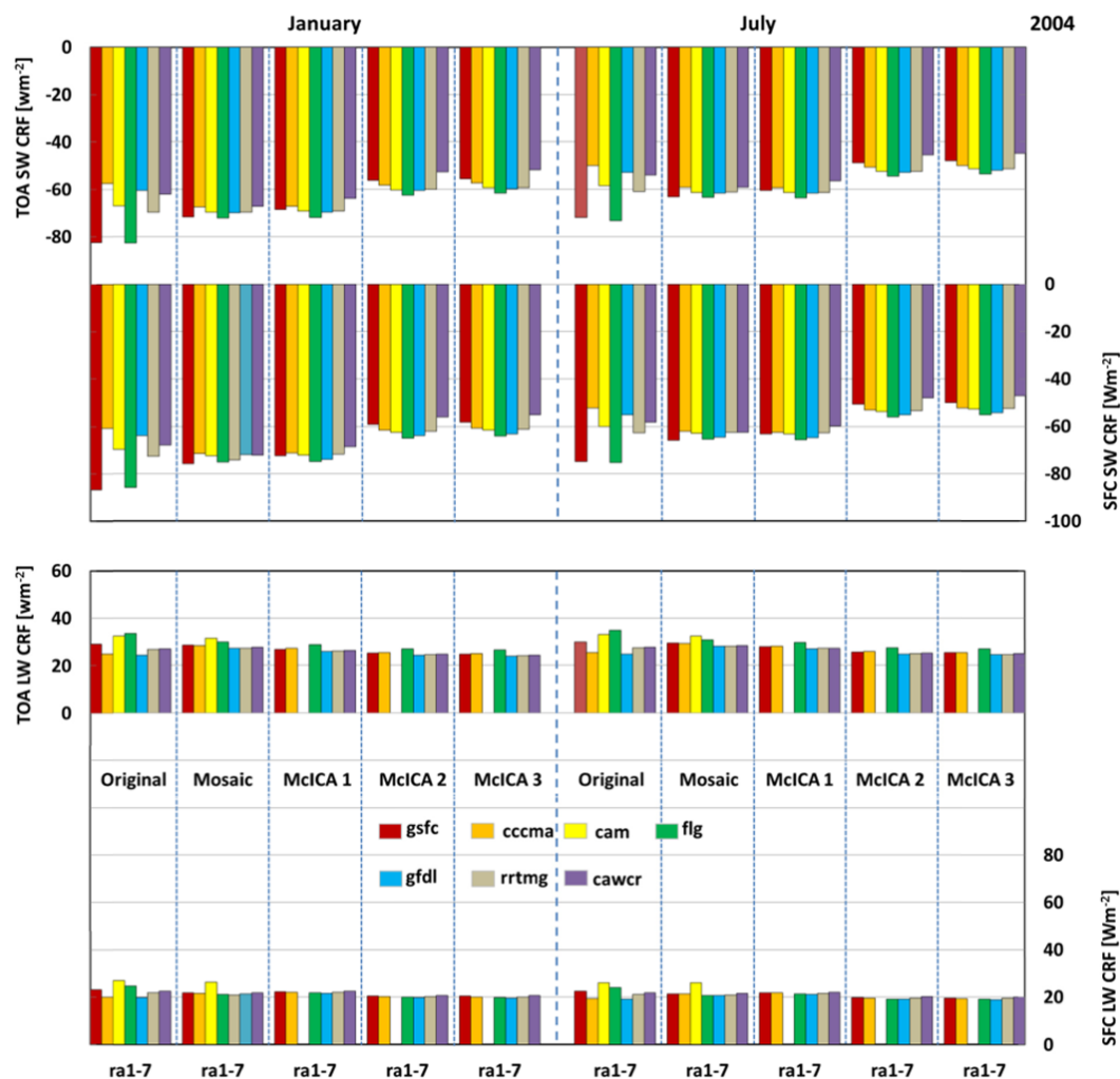
Fig. 8. The effects of cloud overlap treatment comparing the original scheme, mosaic, and McICA with three cloud generators on TOA and surface (SFC) SW and LW cloud radiative forcing (CRFs) averaged over [60^{\circ}\text{S}–60^{\circ}\text{N}] for January (left) and July (right) 2004.
