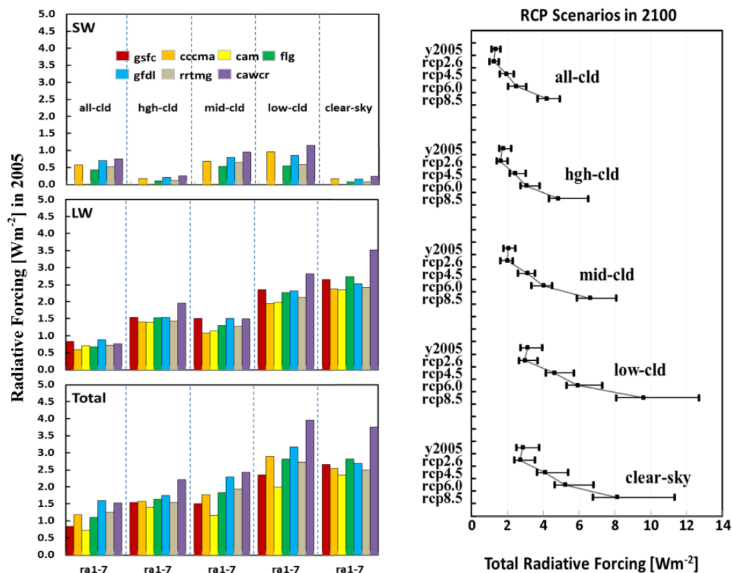
Fig. 3. The SW, LW, and total radiative forcings ( \text{Wm}^{-2} ) for the present condition in year 2005 among the seven major radiation transfer schemes (left), and the total radiative forcings ( \text{Wm}^{-2} ) under the clear-sky and prescribed low-, middle-, high-, and all-cloud conditions for the four IPCC RCP scenarios in year 2100 and present conditions (right). Error bars depict the min–max ranges among the radiation transfer schemes excluding gsfc and cam. These forcings are the instantaneous changes in TOA radiative fluxes relative to the aerosol-free condition in 1765AD without stratospheric adjustment.
