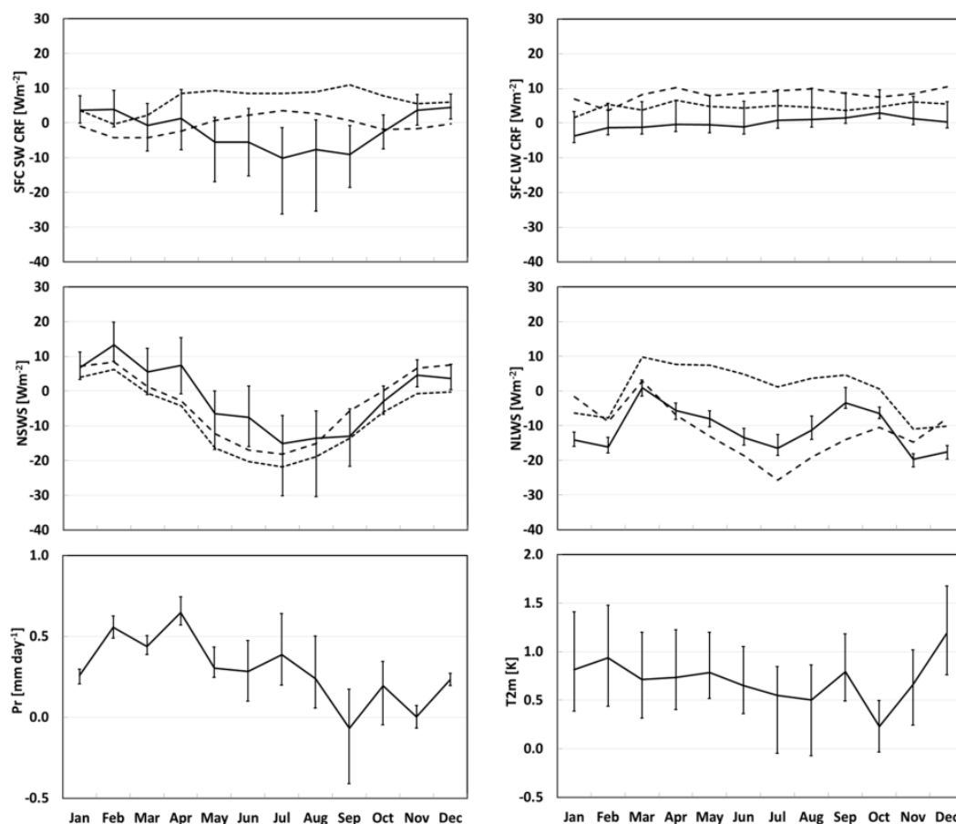
Fig. 9. Monthly variations during 2004 of CWRf biases averaged over the US land for surface net SW and LW radiative fluxes and the CRFs ( \text{Wm}^{-2} ), surface air temperature (T2m, K), and precipitation (Pr, \text{mm day}^{-1} ), including the ensemble mean and min–max range among the seven major radiation packages. The reference for radiative quantities is from ISCCP, along with the observational uncertainty shown as the departures of SRB (dashed) and CERES (dotted).
