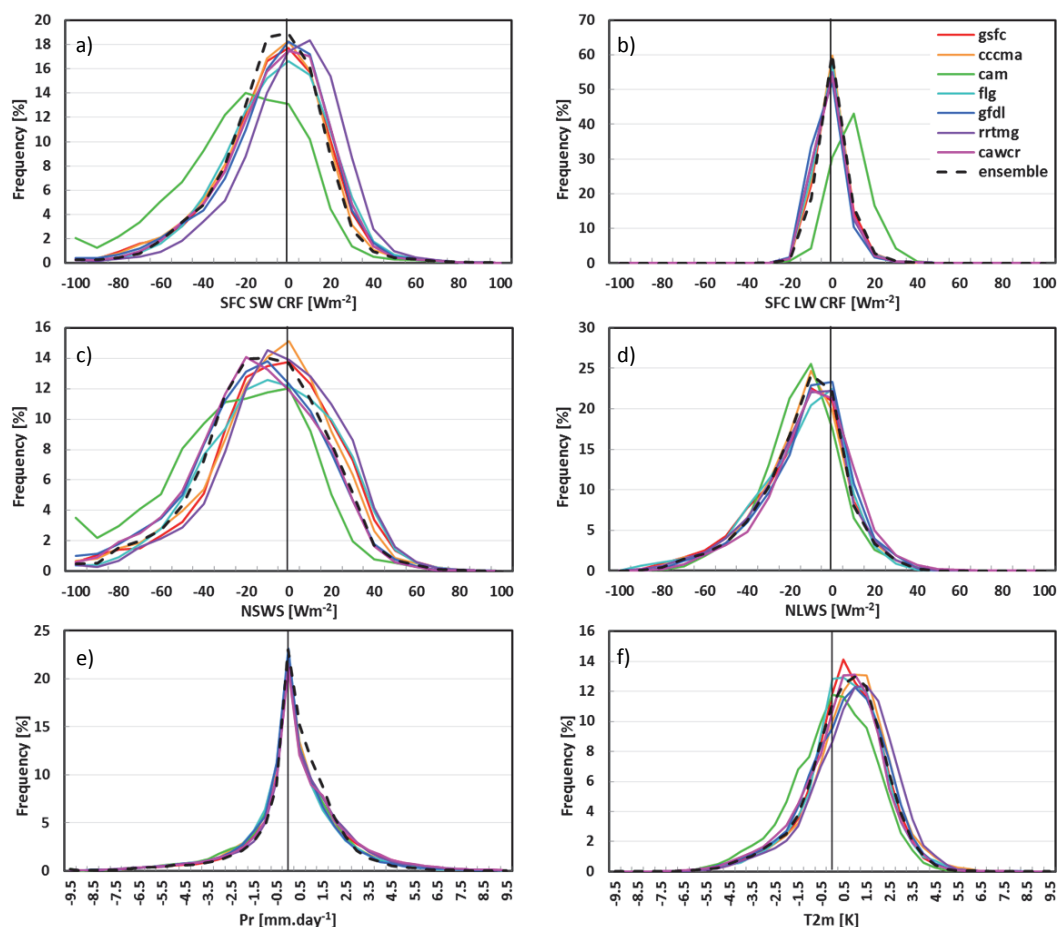
Fig. 10. Spatial frequency distributions of CWRP biases in surface net SW (left) and LW (right) CRFs (a, b), net radiative fluxes (c, d), Pr (e) and T2m (f) among the seven major radiation packages. The statistics are based on monthly means during June, July, and August 2004 over all US land grids.
