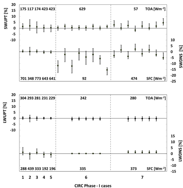
Fig. 2. The percentage differences (%) from the LBL reference (LW: LBLRTM, SW; LBLRTM-CHARTS) among the seven major radiation transfer schemes, including their mean (block) and min–max range (error bar). For CIRC Phase I case 6 and 7, the results for five LW and eight SW cloud optical property schemes are shown. The reference values are listed in each panel at the top for TOA and the bottom for SFC, with the corresponding scaling at the upper left and lower right.
