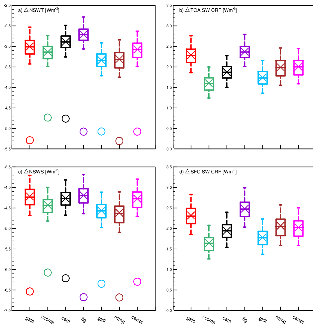
Fig. 4. Global mean aerosol direct radiative effects on TOA (top) and surface (bottom) SW all-sky net fluxes with clear-sky values (circle, a , c ) and CRFs ( b , d ) on average for January and July 2004 using the MISR climatological aerosol distribution. The box plot shows the minimum, 25th percentile, median, 75th percentile, and maximum values among the 64 cloud members for each radiation transfer scheme, while the X within each box depicts the ensemble mean.
