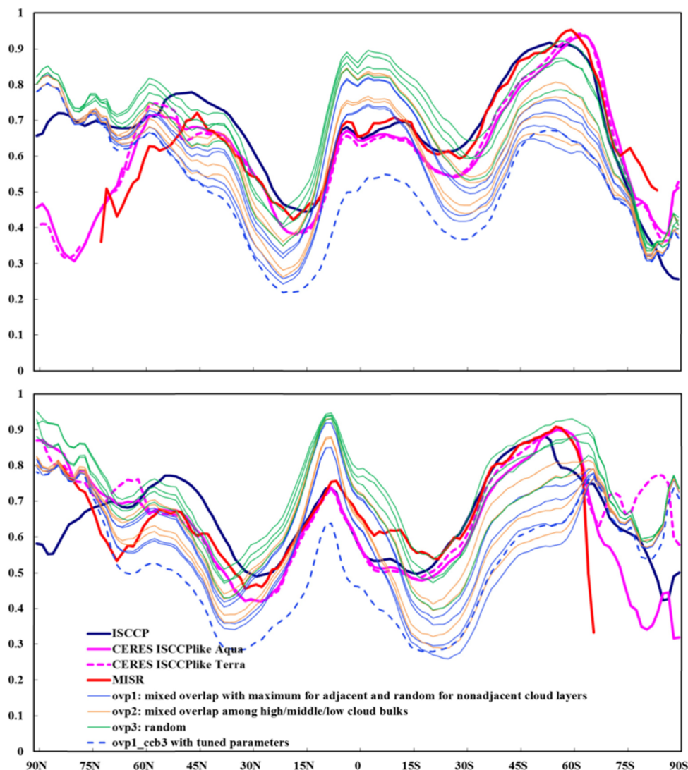
Fig. 6. Zonal mean total cloud cover fractions for January (top) and July (bottom) 2004 among three vertical overlap schemes built in CAR, as compared with four satellite products. For each overlap scheme, four cloud cover prediction schemes are shown using the same color.
