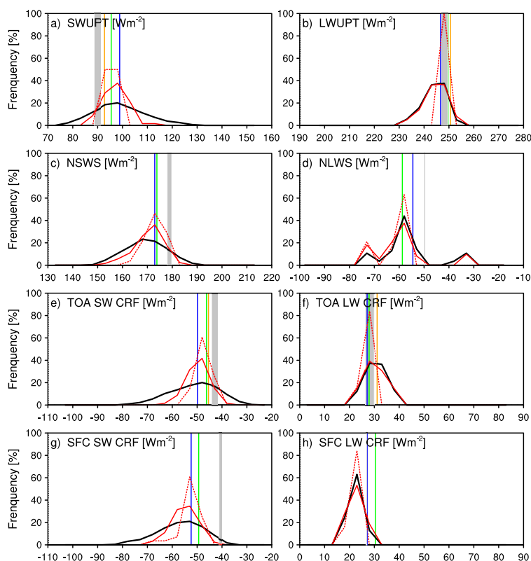
Fig. 5. The CAR member frequency distributions (thick black curves) in predicting the top and surface net radiative fluxes ( a–d ), \text{Wm}^{-2} and cloud radiative forcings (CRF, e–g ), \text{Wm}^{-2} averaged over [60^{\circ}\text{S}–60^{\circ}\text{N}] in July 2004 for SW (left) and LW (right) to a subset of 448 members. The red curves are the respective results from the subset with the observational constraints on NSWT and NLWT separately (dashed) and their sum (solid). The CAR ensemble mean (black) is compared with the observational data from ISCCP (red), SRB (green), various versions of CERES (purple shading), and CERES_EBAF (orange).
