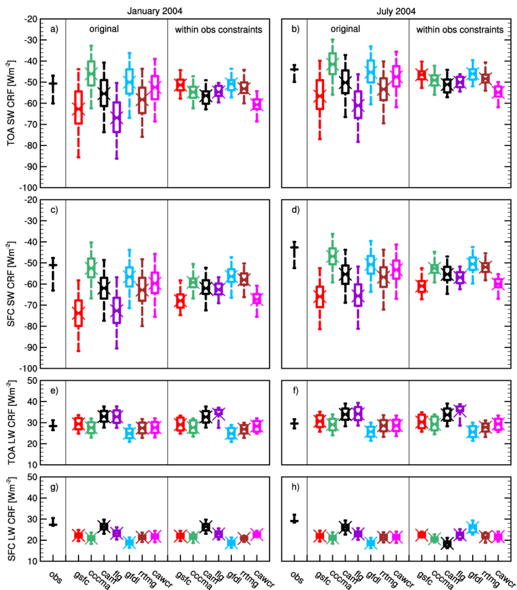
Fig. 7. The SW cloud radiative forcing (CRF) averaged over [60^{\circ}\text{S}–60^{\circ}\text{N}] in January (left) and July (right) 2004. Shown are observations (min–max ranges among ISCCP, SRB, CERES, and CERES EBAF), the original results and those with the observational constraints on (NSWT + NLWT), respectively. The box plot illustrates the minimum, 25th percentile, median, 75th percentile, and maximum values among different cloud members for each radiation transfer scheme, while the X within the boxes depicts the ensemble mean.
