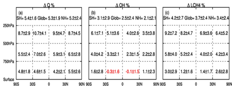
Fig. 6. Percent change in multi-model mean (10 models) regional a) specific humidity, b) tropospheric OH and c) methane loss flux due to climate change only (2000–Em2000C1850). Decreases are shown in red and increases are in black.
