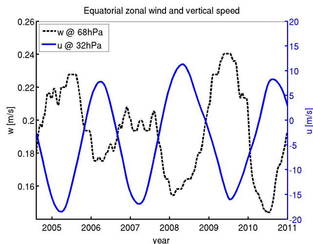
Fig. 10. Ascent rate w at the Equator between the 68 and 56 hPa level (dashed black, left y-axis) together with the average equatorial zonal wind u (solid blue, right y-axis) higher up at 32 hPa. In order to compare to the ascent rate the zonal wind is smoothed with a one year forward moving average. The data confirm the sketch in Fig. 9 and show maximum ascent rates during the easterly phase ( u < 0 ) and minimum during the westerly phase ( u > 0 ).
