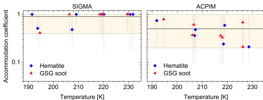
Fig. 6. Accommodation coefficients \alpha_{\text{ice}} obtained from SIGMA and ACPIIM model calculations for the AIDA experiments listed in Table 3. Best-fit values relate to the median of the distributions of \alpha_{\text{ice}} values that were retrieved by the uncertainty analysis described in Sect. 5.1, while error bars indicate the respective lower and upper quartiles. Likewise, median as well as lower and upper quartiles were determined from the temperature distribution of each experiment and applied accordingly. The temperature-averaged \alpha_{\text{ice}} values obtained by SIGMA \alpha_{\text{ice}}^{\text{SIGMA}} = 0.9^{+0.1}_{-0.5} and ACPIIM \alpha_{\text{ice}}^{\text{ACPIIM}} = 0.5^{+0.5}_{-0.3} are given by the solid black lines with the shaded region indicating their uncertainty.
