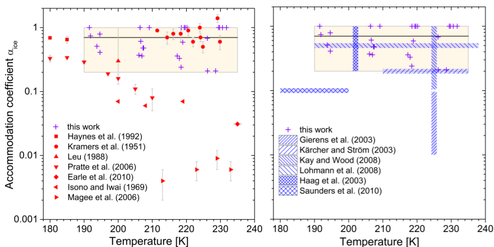
Fig. 7. Comparison of the combined SIGMA and ACPIIM result \alpha_{\text{ice}} = 0.7^{+0.3}_{-0.5} (black solid line, uncertainty illustrated by the shaded region) resulting from the AIDA cirrus cloud experiments (purple crosses, cf. Fig. 6) between 190 K and 235 K with literature data from laboratory measurements (red symbols, cf. Table 1) and cirrus cloud model studies (blue bars, cf. Table 2). Error bars are included when given in the original publication. For the cirrus cloud model studies, the bars indicate the range of preferred \alpha_{\text{ice}} values at one temperature or the preferred \alpha_{\text{ice}} value within the considered temperature range, respectively.
