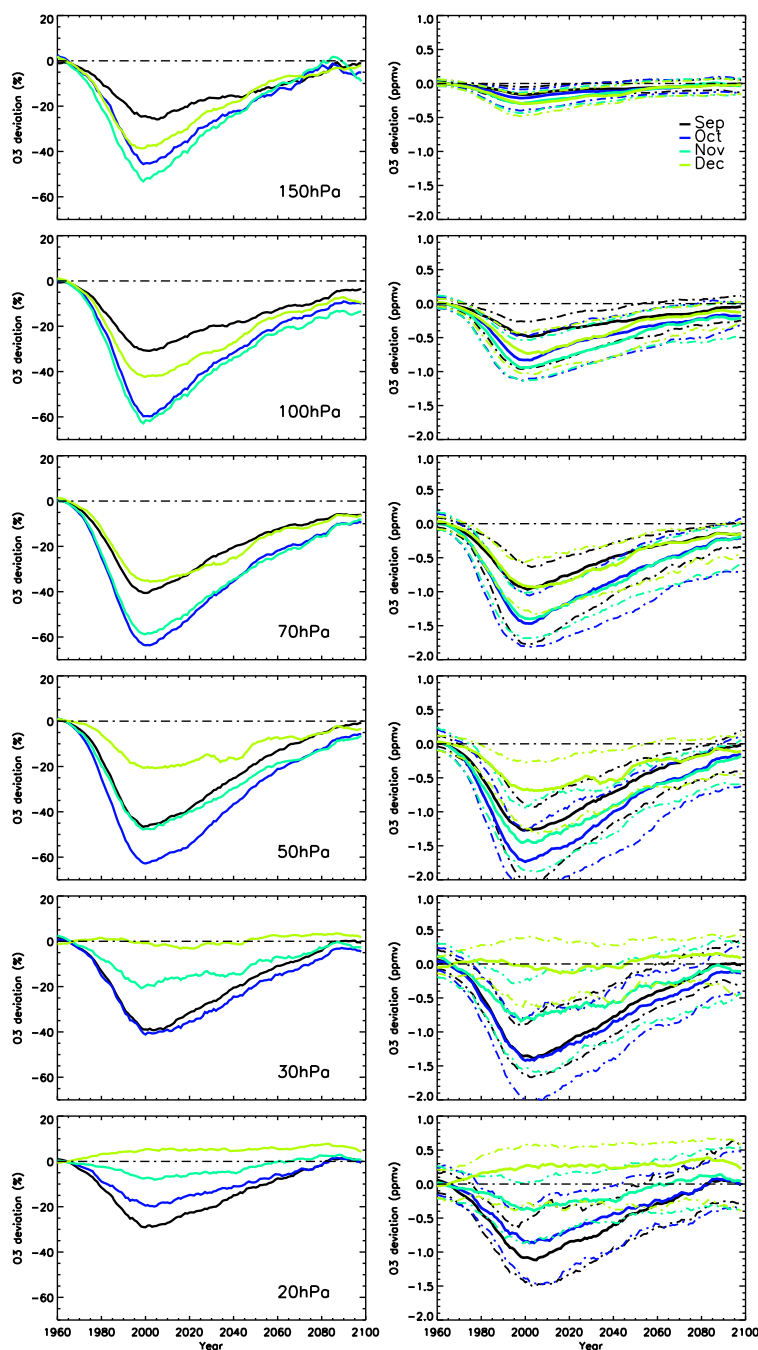
Fig. 5. Deviations of monthly multi-model median ozone VMR from 1965 baseline, zonally averaged poleward of 60^{\circ} S for all available pressure levels considered by CCMVal-2 models in the range of 20–150 hPa. Left panels – percent deviation from baseline, right panels – absolute deviation from baseline. Dashed lines indicate 95 % confidence level of median. Model data have been smoothed with a 15 yr boxcar filter.
