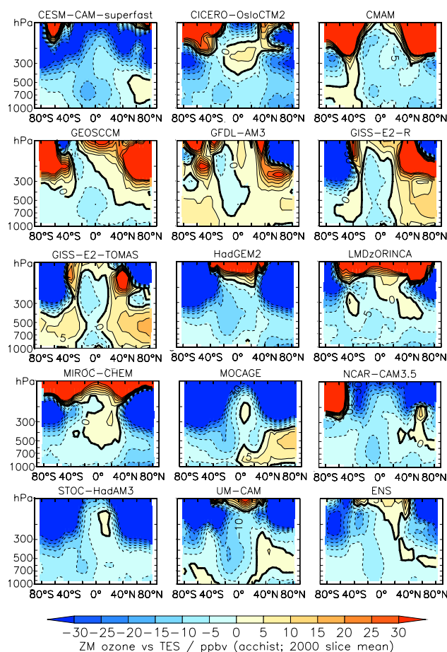
Fig. 2. Zonal bias between ACCMIP models and TES ozone averaged over 2005–2010. Ensemble average of ACCMIP compared to TES ozone is shown under ENS in the bottom right.
