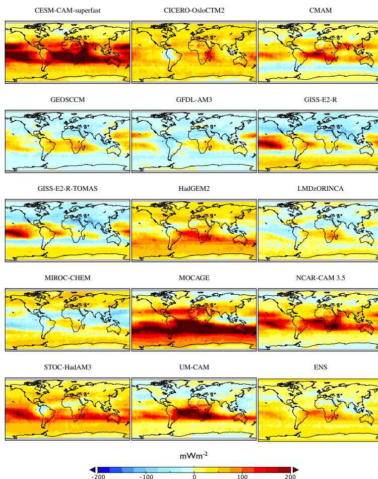
Fig. 4. Spatial distribution of ACCMIP OLR bias from tropospheric ozone, \delta\text{OLR}_m^j , from 2005–2010, limited to 80^\circ\text{S} – 80^\circ\text{N} , and based on a chemical tropopause q = 150 ppb as diagnosed from TES. ACCMIP ensemble, \overline{\delta\text{OLR}}_j , is denoted by ENS.
