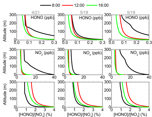
Fig. 8. Modeled vertical profiles of daytime HONO (upper panel), NO 2 (middle panel) and HONO/NO 2 ratios (lower panel) at 08:00, 12:00, and 16:00 CST on 21 April, 18 May, and 19 May. Results are from model runs with photolytic HONO sources at the ground and on aerosol.
