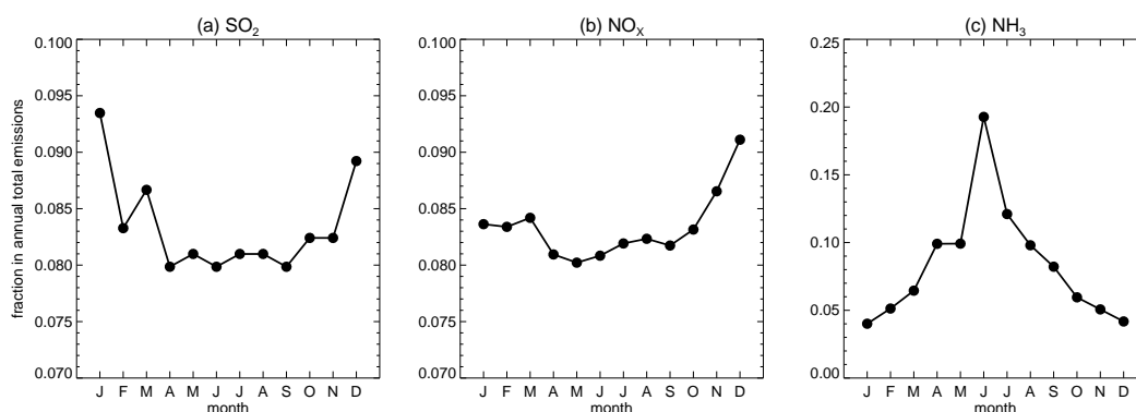
Fig. 2. Seasonality of (a) \text{SO}_2 , (b) \text{NO}_x and (c) \text{NH}_3 emissions from China.
