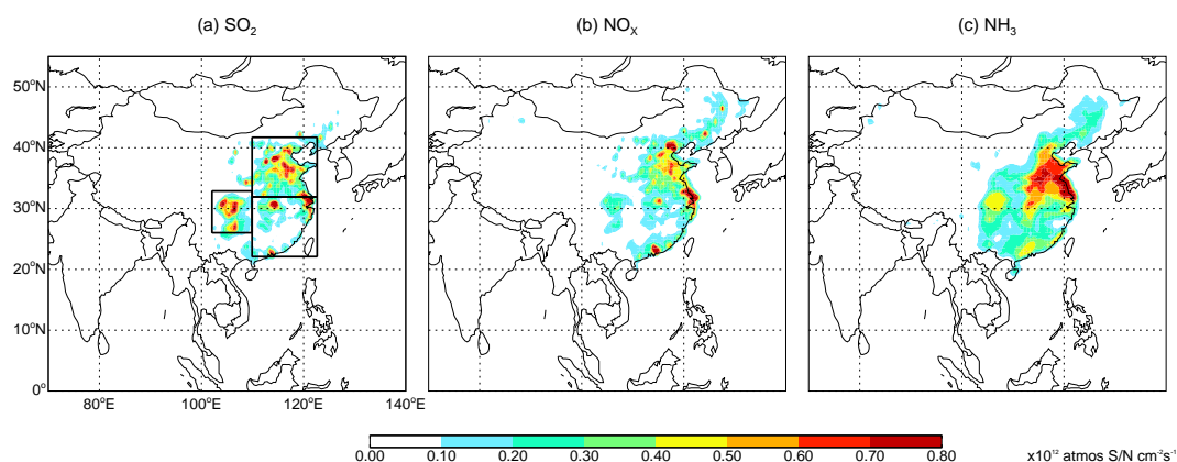
Fig. 1. Spatial distributions of (a) \text{SO}_2 , (b) \text{NO}_x and (c) \text{NH}_3 emissions from China used in the 2006C simulation. Please note that this figure is not the whole East Asian model domain, which is shown in Fig. 3, and that emissions outside of China are omitted. The rectangles in (a) represent North China (upper right), South China (lower right), and the Sichuan Basin (left).
