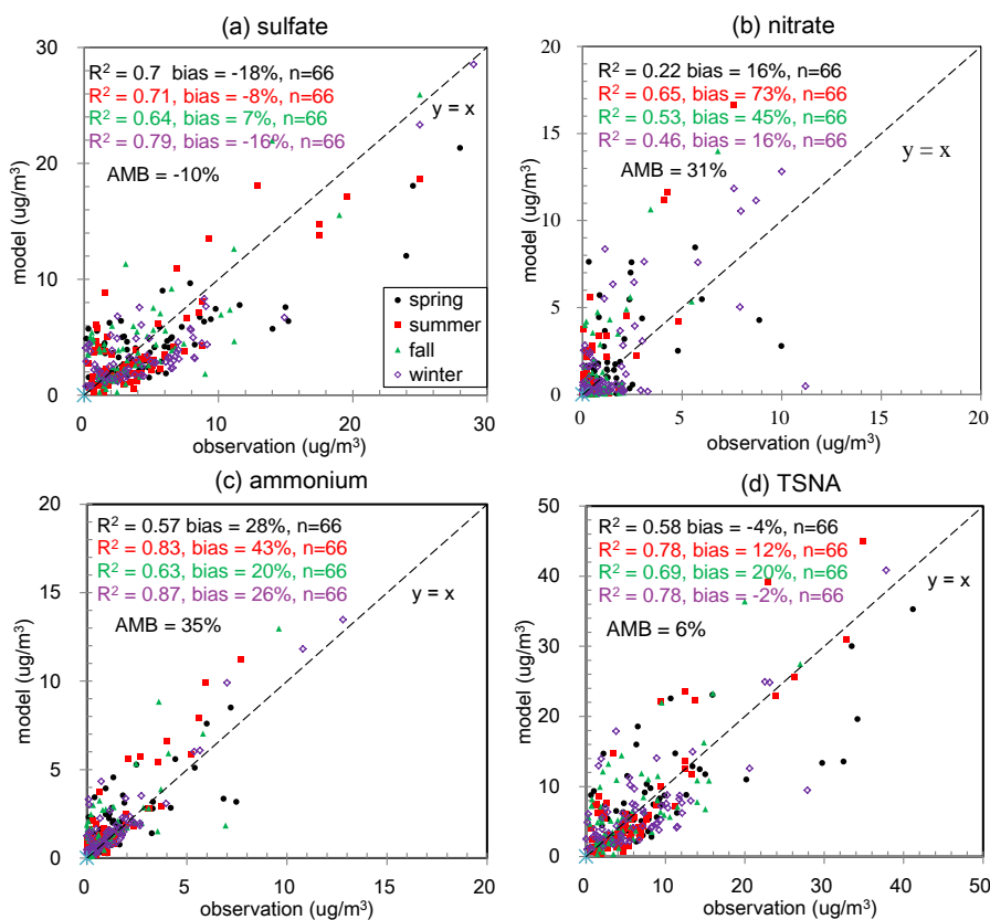
Fig. 5. Scatter plots of simulated versus observed SNA concentrations at 22 (the 4 EANET sites inside China have no observation data for SNA) sites in East Asia, including 2 sites in China (BB and MY) and 20 sites from other countries. Values are seasonal mean for 2006. The black dots represent spring, the red squares represent summer, the green triangles represent fall, and the violet hollow diamonds represent winter. AMB = annual mean bias. The square of correlation coefficient ( R^2 ), normalized mean bias, and annual mean bias (AMB) are given in each scatter plot. The y = x relationship (dashed lines) is shown.
