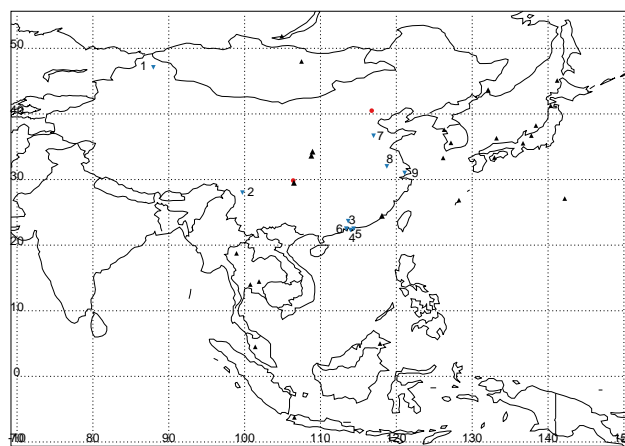
Fig. 3. The nested-grid model domain and locations of observational data used in this study. The black triangles represent 25 sites from EANET; the red circles represent Miyun and Beibe sites with weekly observations; blue inverted triangles represent 9 Chinese rural sites from published papers: (1) Akdala, (2) Shangri-La (X. Y. Zhang et al., 2012), (3) Conghua, (4) Tung Chung, (5) Tap Yun, (6) Zhongshan (Hagler et al., 2006), (7) Jinan (Yang, 2008), (8) Nanjing (Yang et al., 2005), and (9) Shanghai (Wang et al., 2006).
