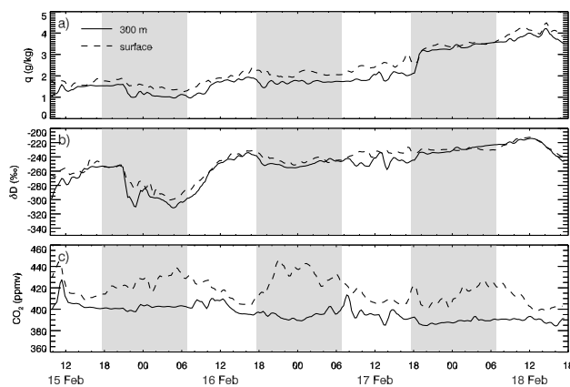
Fig. 4. Time series of (a) q ( \text{g kg}^{-1} ), (b) \delta\text{D} (‰) and (c) \text{CO}_2 (ppmv) near the surface (taken at 10 m) and at the top of the tower over the four-day experiment. The time axis is in hours (local) Mountain Standard Time. Shading indicates the time between local sunset at 05:40 p.m. and sunrise at 06:50 a.m.
