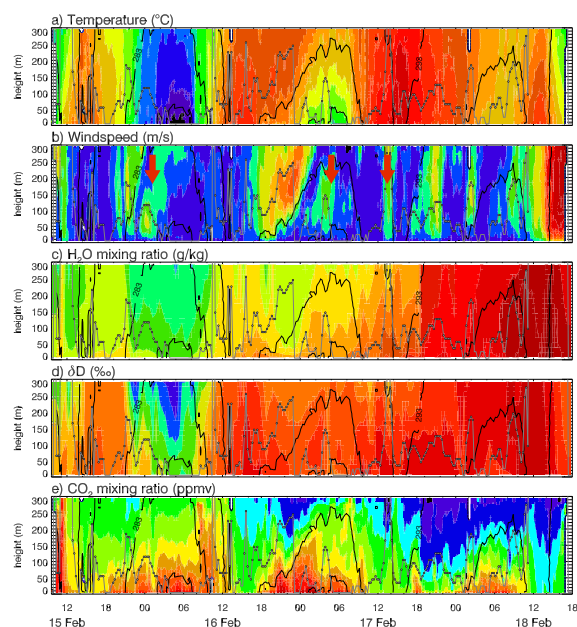
Fig. 3. Time height sections of (a) temperature ( ^{\circ}\text{C} ), (b) wind speed ( \text{m s}^{-1} ), (c) water vapor mixing ratio (i.e., q , \text{g kg}^{-1} ), (d) \delta\text{D} (‰), and (e) \text{CO}_2 volume mixing ratio (ppmv). Contours show potential temperature (K). Grey dots show where the Richardson number is the critical value, and the grey line estimates the depth of the convective layer. The time axis is in hours local Mountain Standard Time, and spans from 09:00 a.m. 15 February to 06:00 p.m. on 18 February. Arrows indicate examples of intermittent turbulent burst events.
