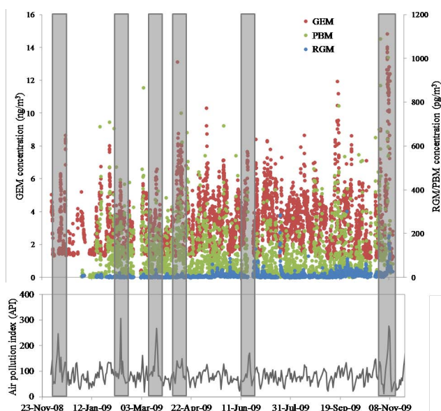
Fig. 2. Hourly averaged GEM, RGM and PBM concentrations at the monitoring site and air pollution index (API) in the Beijing urban area from December 2008 to November 2009.
