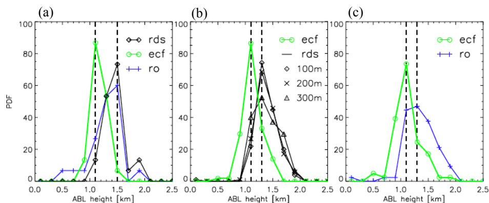
Fig. 4. The PDF of the ABL heights (a) for radiosondes (25 profiles, with 100-m smoothing) and the near-coincident COSMIC RO and ECMWF analysis; (b) for radiosonde (190 profiles) with three vertical smoothing intervals (100, 200 and 300 m) and the near-coincident ECMWF analysis over the region (15–25° S, 70–86° W) from 25 October to 1 December 2008; (c) for COSMIC RO soundings (70 profiles) and the near-coincident ECMWF analysis over the region (20–25° S, 70–86° W) from 25 October to 1 December 2008. For better illustration, the normalized PDF is divided by 3 to scale the maximum PDF close to 100. The shape of the PDF is not changed due to the scaling.
