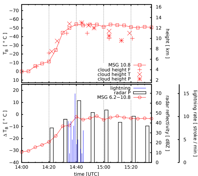
Fig. 2. Temporal evolution of cloud system characteristics derived from remote sensing instruments. Upper panel: minimum brightness temperature of IR channel ( 10.8\ \mu\text{m} ) with corresponding cloud top height (assuming wet adiabatic lapse rate), and estimated cloud top heights from PPI scans of 3 radars (F: Feldberg, T: Türkheim, P: Poldirad). Lower panel: difference between minimum brightness temperatures of WV ( 6.2\ \mu\text{m} ) and IR ( 10.8\ \mu\text{m} ) channels, maximum radar reflectivity measured by Poldirad (at 2^\circ elevation), and lightning rate detected by LINET.
