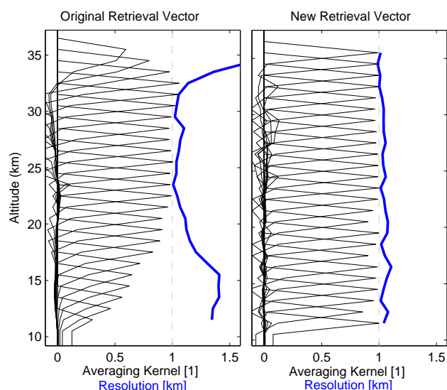
Fig. 2. The averaging kernel in black and resolution in terms of Full Width Half Maximum (FWHM) in blue for a simulated aerosol retrieval using lines-of-sight spaced 1 km in tangent altitude. The left panel shows the result when using the retrieval vector defined in Eq. (1). The right panel shows the improvement when using the retrieval vector defined in Eq. (5).
