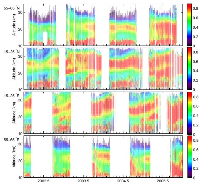
Fig. 7. The daily zonal average OSIRIS aerosol extinction ratio for the SAGE III time period for the following latitude bands shown from top to bottom: 55\text{--}65^\circ N, 15\text{--}25^\circ N, 15\text{--}25^\circ S, and 55\text{--}65^\circ S. Periods when sunlit measurements are not possible due to solar zenith angle greater than 90^\circ or when OSIRIS was turned off for engineering tests are indicated in white.
