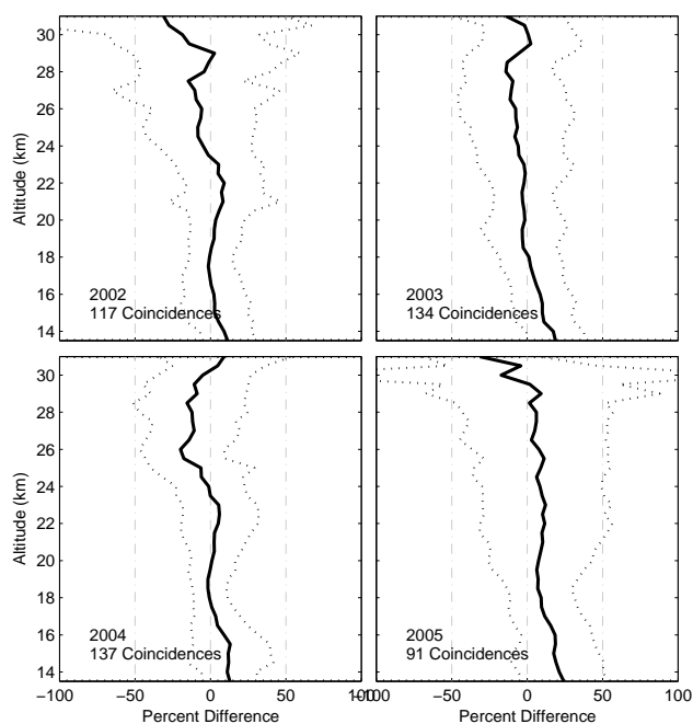
Fig. 4. The mean (solid) and standard deviation (dashed) of the percent difference of all OSIRIS and SAGE III coincidences over the four years of mission overlap, 2002–2005. Top left panel shows the results for 117 coincident measurements in 2002; top right panel shows the results for 134 coincident measurements in 2003; bottom left panel shows the results for 137 coincident measurements in 2004; and, bottom right panel shows the results for 91 coincident measurements in 2005.
