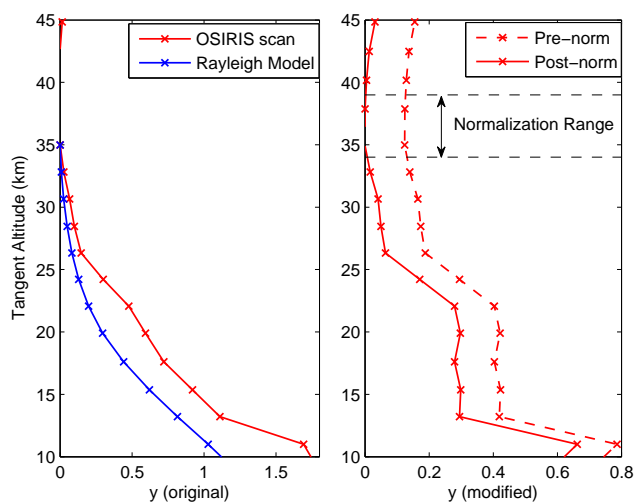
Fig. 1. The stratospheric aerosol retrieval vector, y . The left panel shows y as calculated according the original algorithm for a typical OSIRIS scan in red as well as y for a model calculation of an aerosol-free atmosphere in blue. The right panel shows the modified version of y , before and after the normalization (with dashed red and solid red lines according to Eqs. (4) and (5) respectively).
