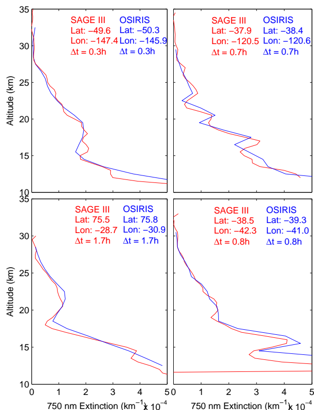
Fig. 3. Four coincident SAGE III and OSIRIS aerosol extinction coefficient measurements. SAGE III measurements at 755 nm are shown in red and OSIRIS measurements at 750 nm are shown in blue. The latitude, longitude of each measurement and the time difference between each coincident SAGE III and OSIRIS measurement are given in each corresponding plot.
