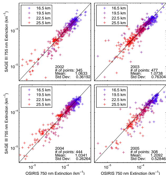
Fig. 5. Comparison of, for OSIRIS and SAGE III aerosol extinction coefficient at four altitude levels: 16.5 km (blue), 19.5 km (purple), 22.5 km (maroon) and 25.5 km (red). Each panel represents one of the four years of overlapping measurements: 2002 in top left, 2003 in top right, 2004 in bottom left and 2005 in bottom right. The mean and standard deviation given in the plots are calculated based on the ratio given in Eq. (8).
