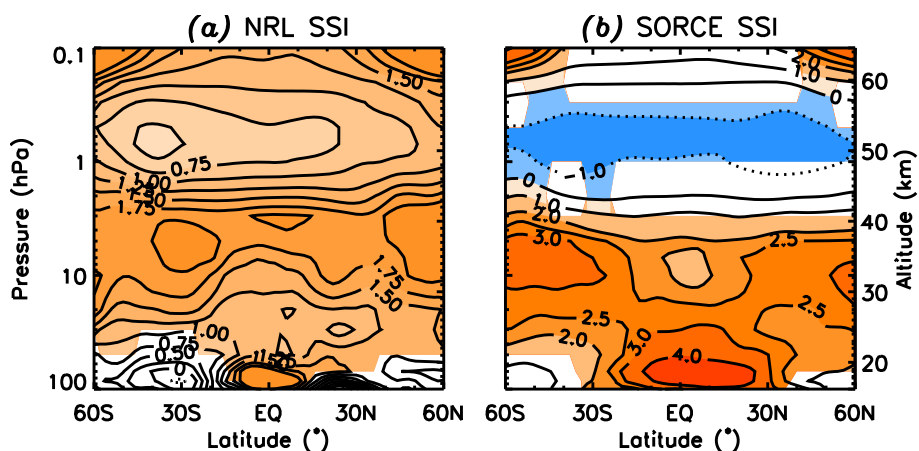
Fig. 5. Simulated ozone solar cycle response in the GEOSCCM, similar to Fig. 4 but in altitude-latitude cross section, using (a) NRL and (b) SORCE SSI. The colored (non-white) portions of the plots indicate regions where the ozone response is statistically significant at the 95 % confidence level.
