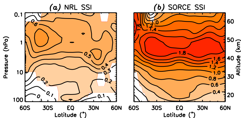
Fig. 8. Same as Fig. 5 but for temperature.
