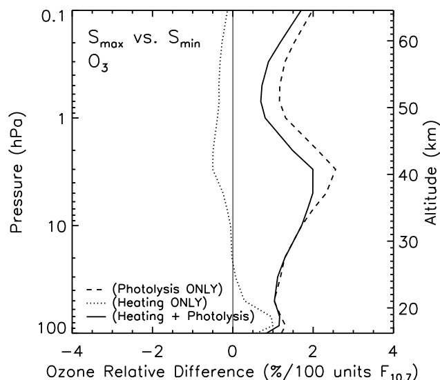
Fig. 2. Ozone response to the 11-yr solar cycle, S_{\max} - S_{\min} (relative %) per 100 units of F_{10.7} , in the stratosphere and lower mesosphere and averaged over 60^\circ S - 60^\circ N latitude, as modeled by the GEOSCCM using the NRL SSI. Three cases are shown, where the solar cycle has been applied (1) only to direct radiative heating, (2) only to photolysis, and (3) with both effects combined.
