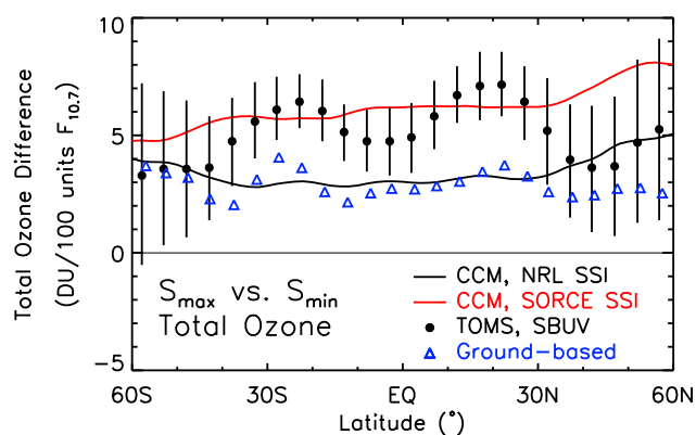
Fig. 6. Total ozone response to the 11-yr solar cycle, as modeled by the GEOSCCM and inferred from observations by regression analyses of the TOMS, SBUV merged total ozone dataset (Stolarski et al., 2006, Fig. 6) and ground-based observations (Randel and Wu, 2007, Fig. 12).
