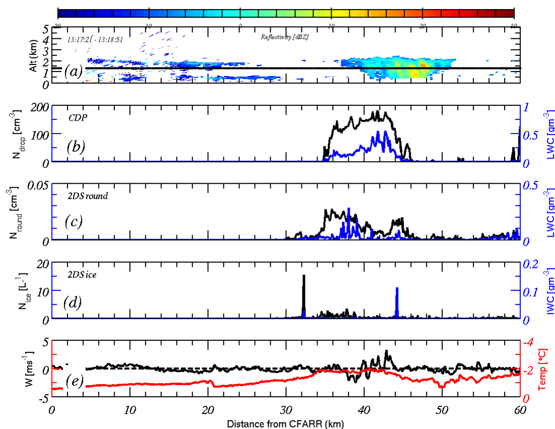
Fig. 4. Reflectivity from the 3 GHz CAMRa RHI scan along the 253^{\circ} radial and GPS altitude (a) – (top panel, time of scan indicated in top left). In situ total particle number concentration (black lines, left axes) and mass loadings (blue lines, right axes) measured by the CDP (b) as a function of distance from CFARR; 2DS round classification (c), and 2DS ice classification (d). Also shown (e); in situ temperature from the de-iced Rosemount sensor; vertical wind speed from the 5-hole pressure port turbulence probe, all from run R1, inbound to CFARR.
